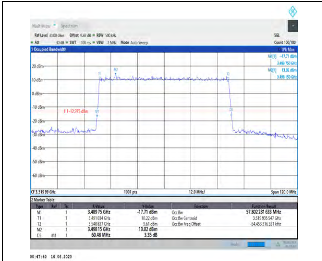
1-N78-3450-3550-PC1.5-30-60-H-5-DFT-256QAM-Outer_Full-162@0-Ant1-57.802-60.480-≤60-PASS
