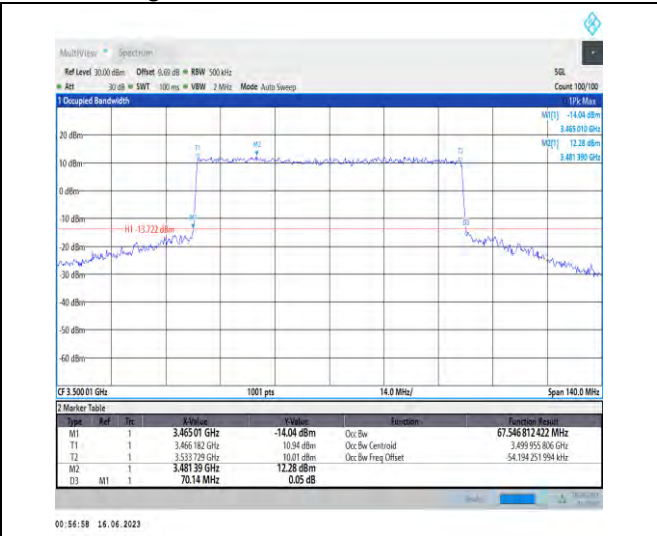
1-N78-3450-3550-PC1.5-30-70-M-8-CP-64QAM-Out er_Full-189@0-Ant1-67.547-70.140-≤70-PASS
