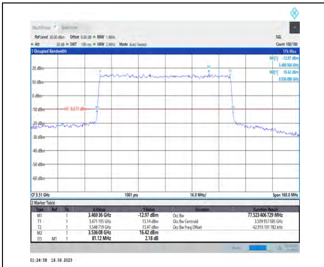
1-N78-3450-3550-PC1.5-30-80-H-7-CP-16QAM-Out er_Full-217@0-Ant1-77.523-81.120-≤80-PASS
