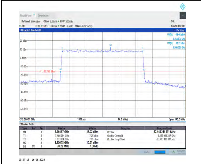
1-N78-3450-3550-PC1.5-30-70-M-9-CP-256QAM-Out er_Full-189@0-Ant1-67.444-70.280-≤70-PASS
