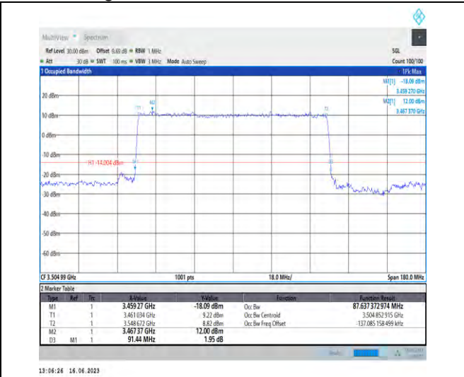
1-N78-3450-3550-PC1.5-30-90-H-9-CP-256QAM-Out er_Full-245@0-Ant1-87.637-91.440-≤90-PASS
