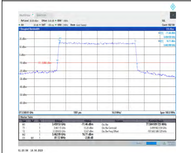
1-N78-3450-3550-PC1.5-30-80-M-6-CP-QPSK-Outer_Full-217@0-Ant1-77.505-81.120-≤80-PASS
