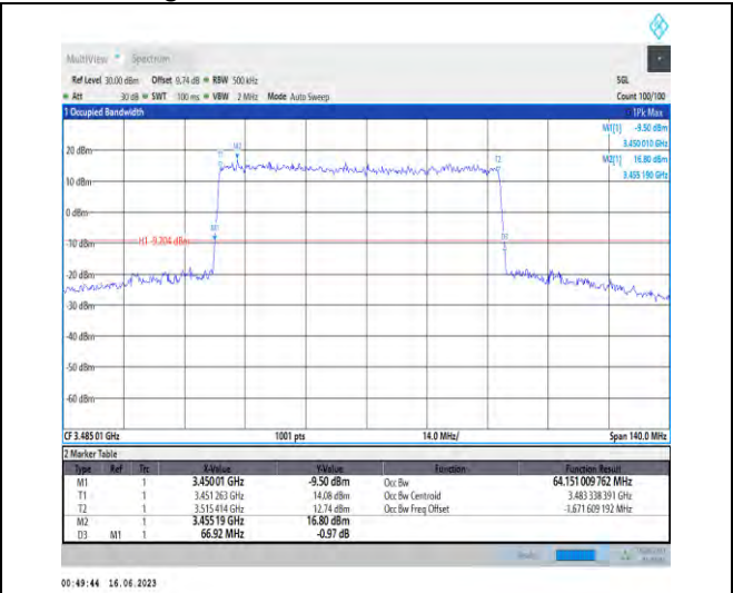
1-N78-3450-3550-PC1.5-30-70-L-1-DFT-QPSK-Outer_Full-180@0-Ant1-64.151-66.920-≤70-PASS
