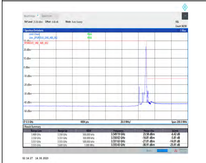
1-N78-3450-3550-PC1.5-30-10-H-5-CP-QPSK-Edge_1RB_Right-1@23-Ant1-1--PASS-see graph
