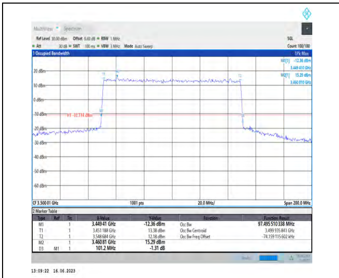
1-N78-3450-3550-PC1.5-30-100-L-7-CP-16QAM-Out er_Full-273@0-Ant1-97.496-101.200-≤100-PASS
