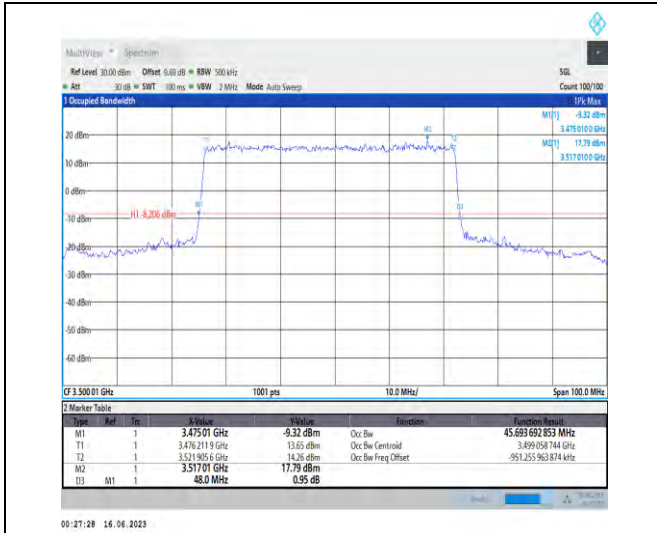
1-N78-3450-3550-PC1.5-30-50-M-1-DFT-QPSK-Out er_Full-128@0-Ant1-45.694-48.000-≤50-PASS
