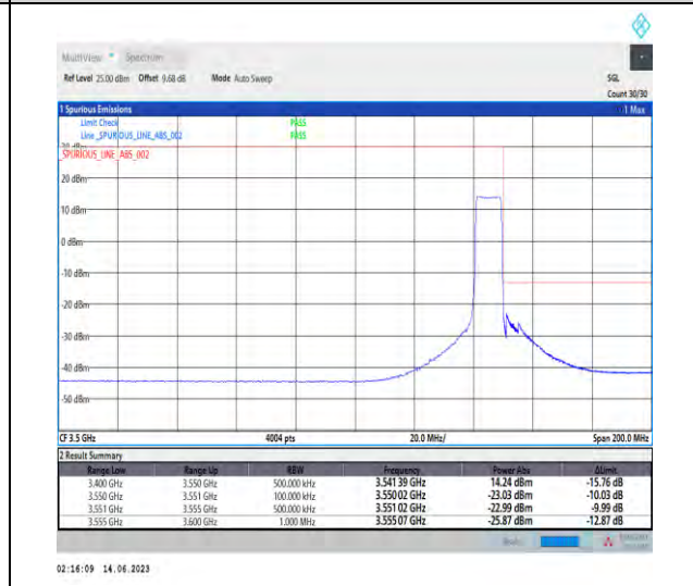
1-N78-3450-3550-PC1.5-30-10-H-6-CP-QPSK-Outer_Full-24@0-Ant1-1--PASS-see graph
