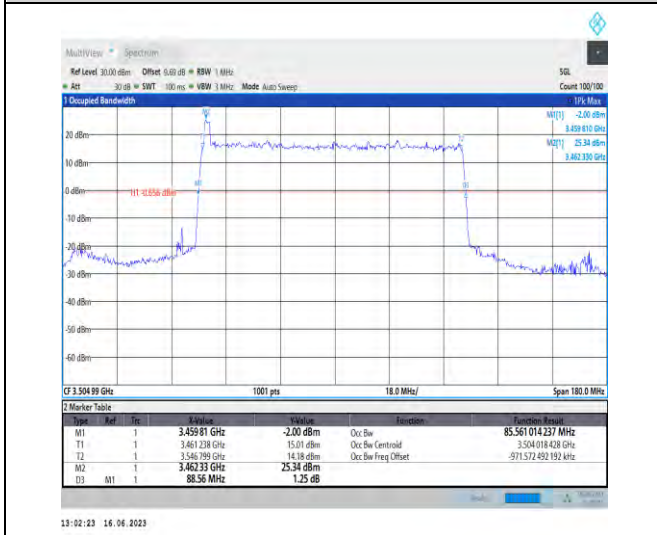
1-N78-3450-3550-PC1.5-30-90-H-2-DFT-PI2BPSK-Outer_Full-240@0-Ant1-85.561-88.560-≤90-PASS
