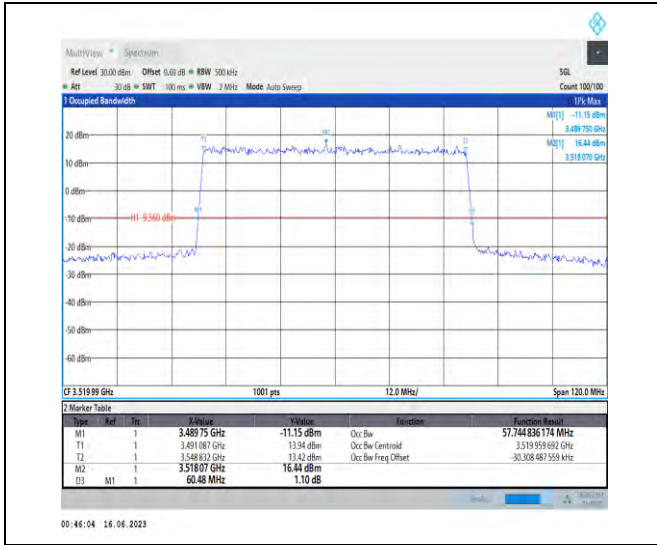
1-N78-3450-3550-PC1.5-30-60-H-1-DFT-QPSK-Out er_Full-162@0-Ant1-57.745-60.480-≤60-PASS
