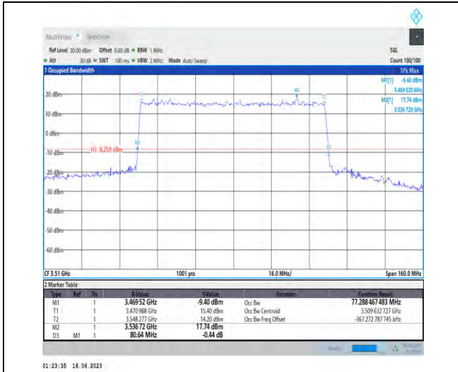
1-N78-3450-3550-PC1.5-30-80-H-3-DFT-16QAM-Outer_Full-216@0-Ant1-77.288-80.640-≤80-PASS
