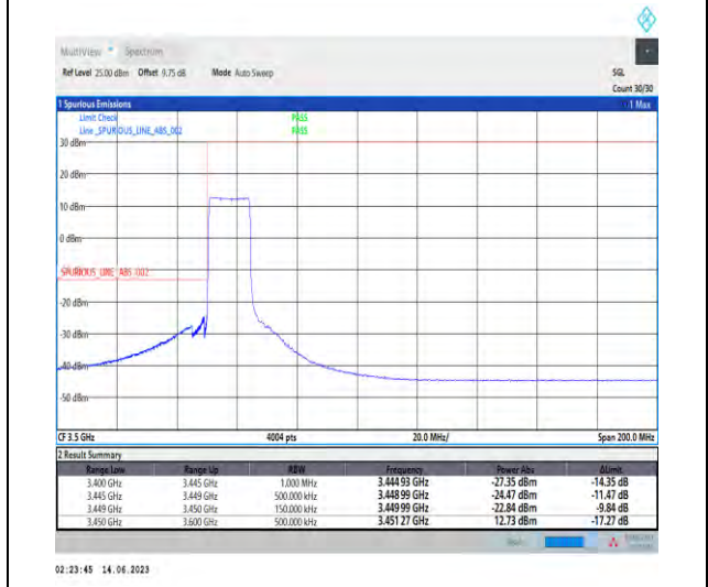
1-N78-3450-3550-PC1.5-30-15-L-6-CP-QPSK-Outer_Full-38@0-Ant1-1--PASS-see graph
