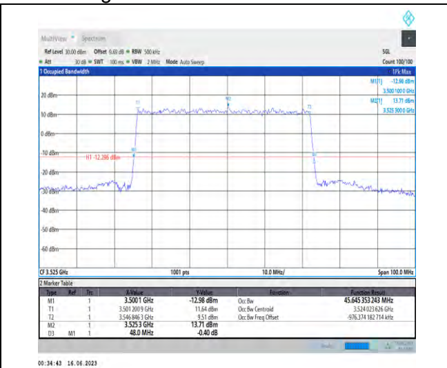
1-N78-3450-3550-PC1.5-30-50-H-5-DFT-256QAM-Outer_Full-128@0-Ant1-45.645-48.000-≤50-PASS
