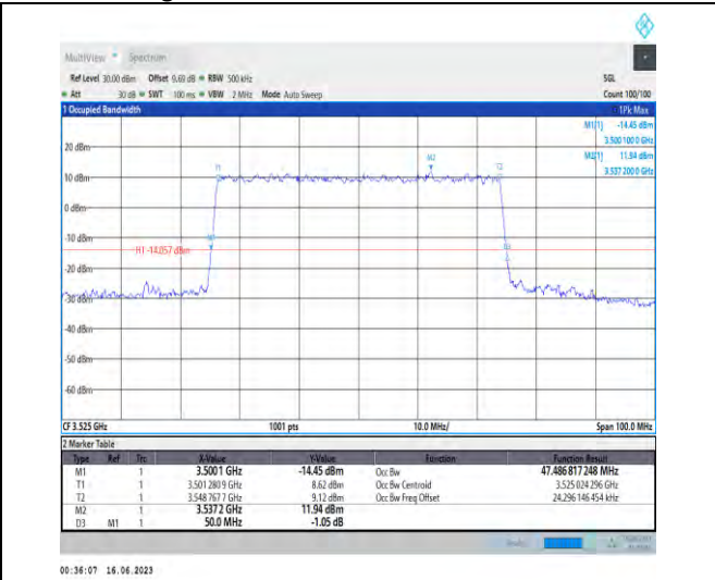
1-N78-3450-3550-PC1.5-30-50-H-9-CP-256QAM-Out er_Full-133@0-Ant1-47.487-50.000-≤50-PASS
