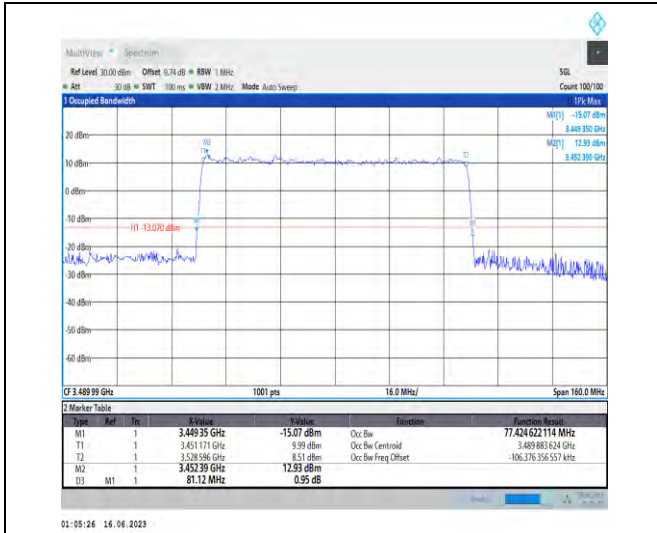
1-N78-3450-3550-PC1.5-30-80-L-9-CP-256QAM-Out er_Full-217@0-Ant1-77.425-81.120-≤80-PASS
