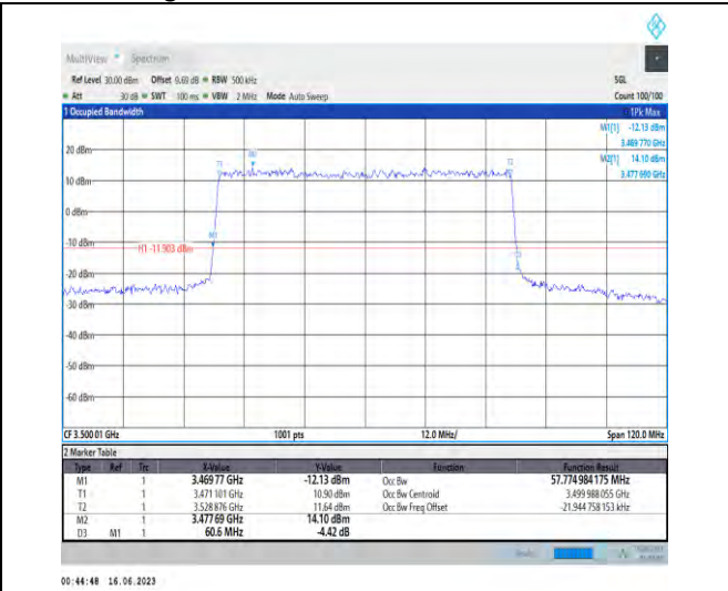
1-N78-3450-3550-PC1.5-30-60-M-7-CP-16QAM-Out_er_Full-162@0-Ant1-57.775-60.600-≤60-PASS
