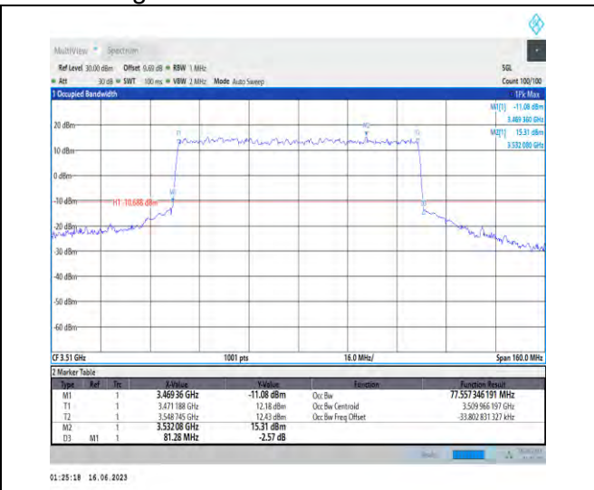
1-N78-3450-3550-PC1.5-30-80-H-8-CP-64QAM-Out er_Full-217@0-Ant1-77.557-81.280-≤80-PASS
