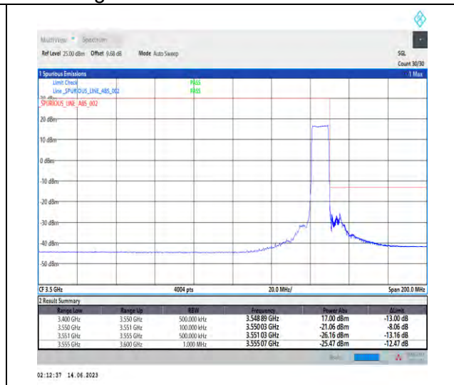
1-N78-3450-3550-PC1.5-30-10-H-3-DFT-PI2BPSK-Outer_Full-24@0-Ant1-1--PASS-see graph
