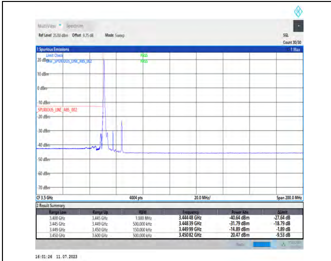
1-N78-3450-3550-PC1.5-30-15-L-1-DFT-PI2BPSK-Edge_1RB_Left-1@0-Ant1-1--PASS-see graph
