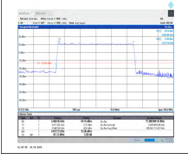
1-N78-3450-3550-PC1.5-30-80-H-9-CP-256QAM-Out er_Full-217@0-Ant1-77.389-81.120-≤80-PASS
