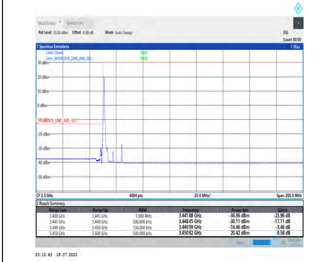
1-N78-3450-3550-PC1.5-30-15-L-4-CP-QPSK-Edge_1RB_Left-1@0-Ant1-1--PASS-see graph
