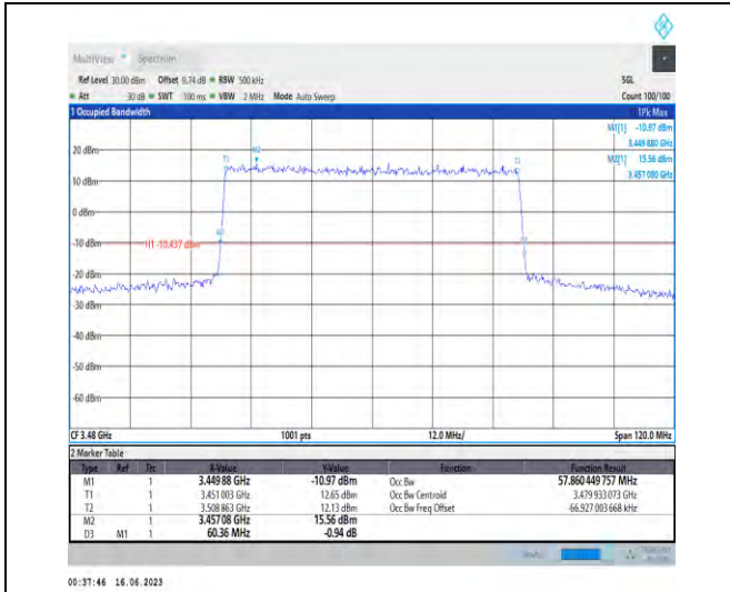
1-N78-3450-3550-PC1.5-30-60-L-3-DFT-16QAM-Out er_Full-162@0-Ant1-57.86-60.360-≤60-PASS
