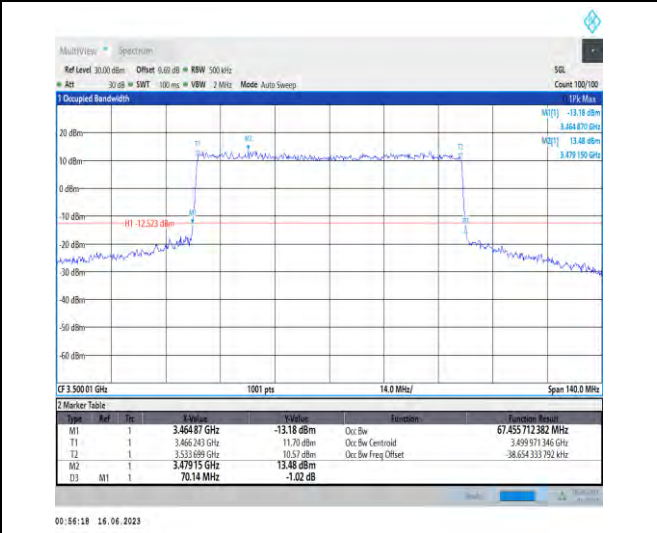
1-N78-3450-3550-PC1.5-30-70-M-6-CP-QPSK-Outer_Full-189@0-Ant1-67.456-70.140-≤70-PASS
