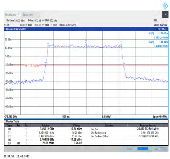
1-N78-3450-3550-PC1.5-30-30-L-5-DFT-256QAM-O uter_Full-75@0-Ant1-26.851-28.680-≤30-PASS
