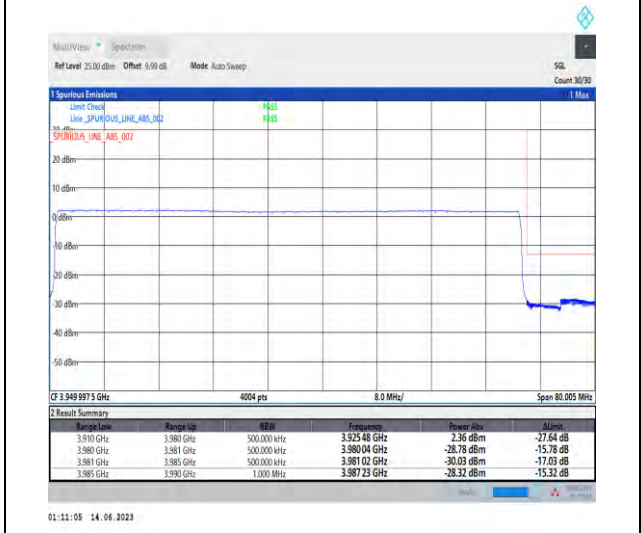
1-N77-3700-3980-PC1.5-30-70-H-6-CP-QPSK-Out_1RB_Right-1@188-Ant1-1--PASS-see graph
