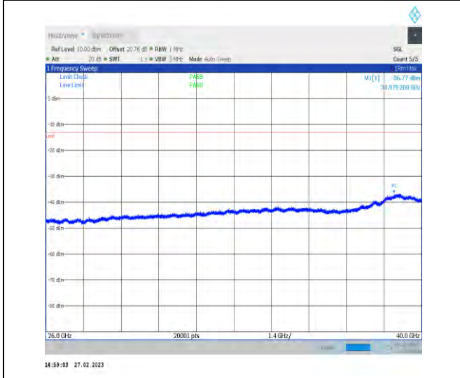
1-N77-3700-3980-PC1.5-30-100-L-1-N/A-DFT-QPSK -Edge_1RB_Left-1@0-26000-40000-Ant1-26000.00-- 49.82--13-PASS
