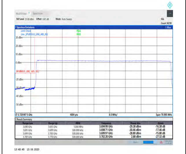
1-N77-3700-3980-PC1.5-30-70-L-6-CP-QPSK-Outer_Full-189@0-Ant1-1-PASS-see graph
