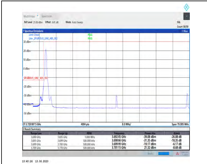
1-N77-3700-3980-PC1.5-30-70-L-1-DFT-PI2BPSK-Edge_1RB_Left-1@0-Ant1-1-PASS-see graph
