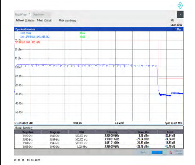
1-N77-3700-3980-PC1.5-30-60-H-6-CP-QPSK-Outer_Full-162@0-Ant1-1--PASS-see graph
