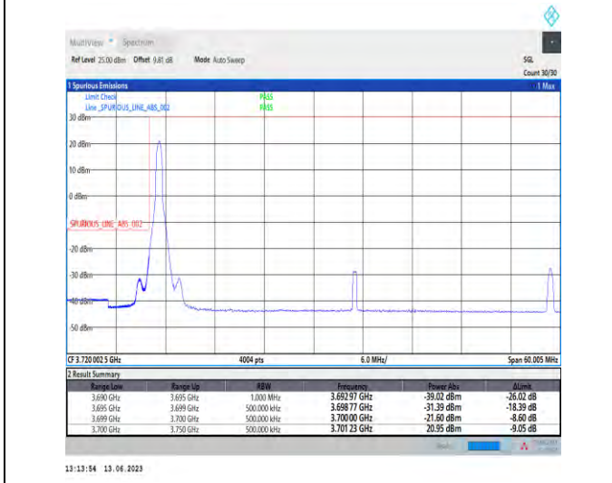
1-N77-3700-3980-PC1.5-30-50-L-4-CP-QPSK-Edge_1RB_Left-1@0-Ant1-1-PASS-see graph
