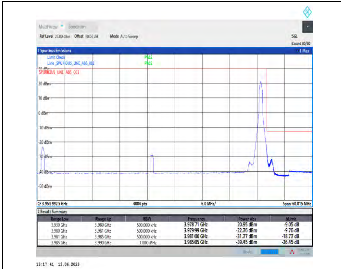
1-N77-3700-3980-PC1.5-30-50-H-2-DFT-PI2BPSK-Edge_1RB_Right-1@132-Ant1-1--PASS-see graph
