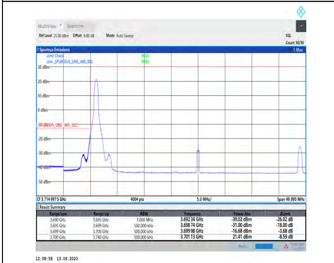
1-N77-3700-3980-PC1.5-30-40-L-4-CP-QPSK-Edge_1RB_Left-1@0-Ant1-1-PASS-see graph
