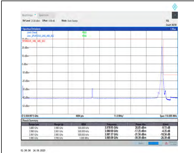
1-N77-3700-3980-PC1.5-30-100-H-2-DFT-PI2BPSK-E dge_1RB_Right-1@272-Ant1-1--PASS-see graph
