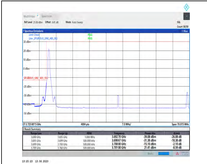
1-N77-3700-3980-PC1.5-30-60-L-1-DFT-PI2BPSK-Edge_1RB_Left-1@0-Ant1-1-PASS-see graph
