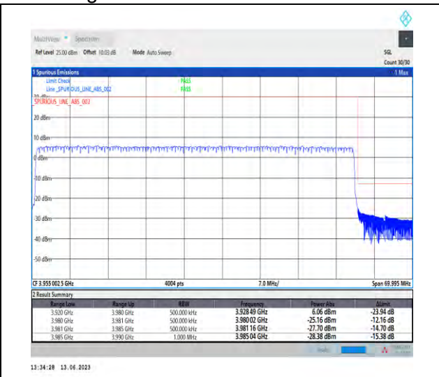
1-N77-3700-3980-PC1.5-30-60-H-3-DFT-PI2BPSK-Outer_Full-162@0-Ant1-1--PASS-see graph
