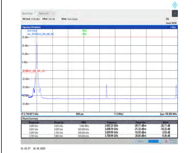
1-N77-3700-3980-PC1.5-30-100-L-4-CP-QPSK-Edge_1RB_Left-1@0-Ant1-1--PASS-see graph
