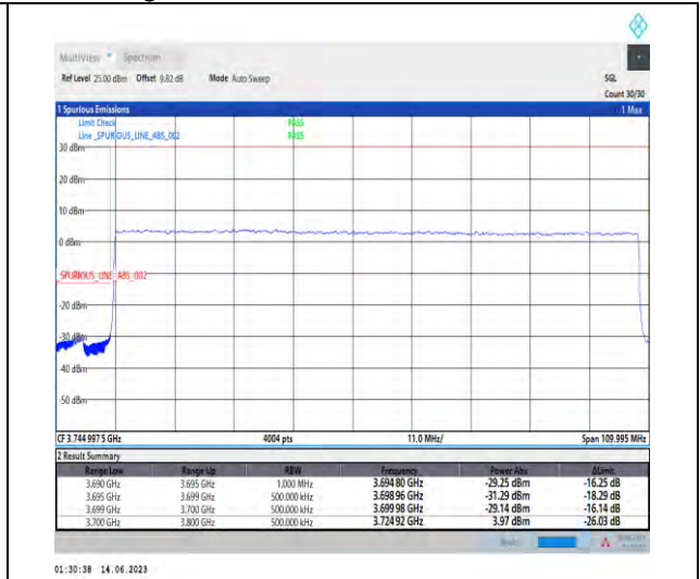
1-N77-3700-3980-PC1.5-30-100-L-3-DFT-PI2BPS K-Outer_Full-270@0-Ant1-1--PASS-see graph
