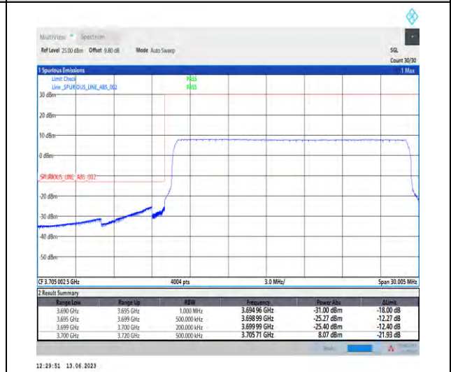
1-N77-3700-3980-PC1.5-30-20-L-6-CP-QPSK-Outer_Full-51@0-Ant1-1--PASS-see graph
