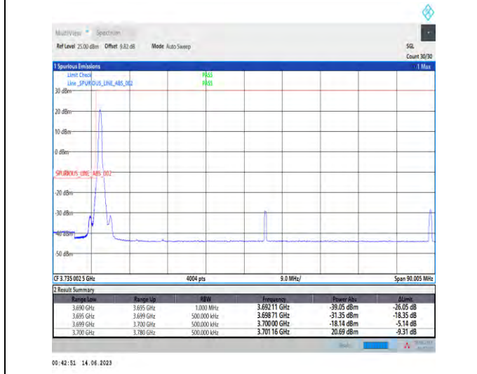
1-N77-3700-3980-PC1.5-30-80-L-4-CP-QPSK-Edge_1RB_Left-1@0-Ant1-1-PASS-see graph
