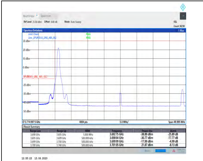
1-N77-3700-3980-PC1.5-30-40-L-1-DFT-PI2BPSK-Edge_1RB_Left-1@0-Ant1-1-PASS-see graph
