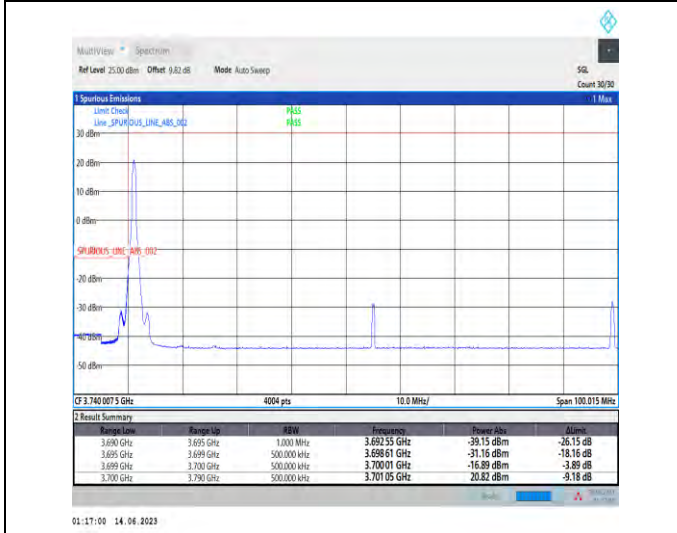
1-N77-3700-3980-PC1.5-30-90-L-4-CP-QPSK-Edge_1RB_Left-1@0-Ant1-1-PASS-see graph
