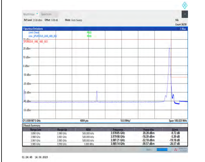
1-N77-3700-3980-PC1.5-30-90-H-5-CP-QPSK-Edge_1RB_Right-1@244-Ant1-1--PASS-see graph
