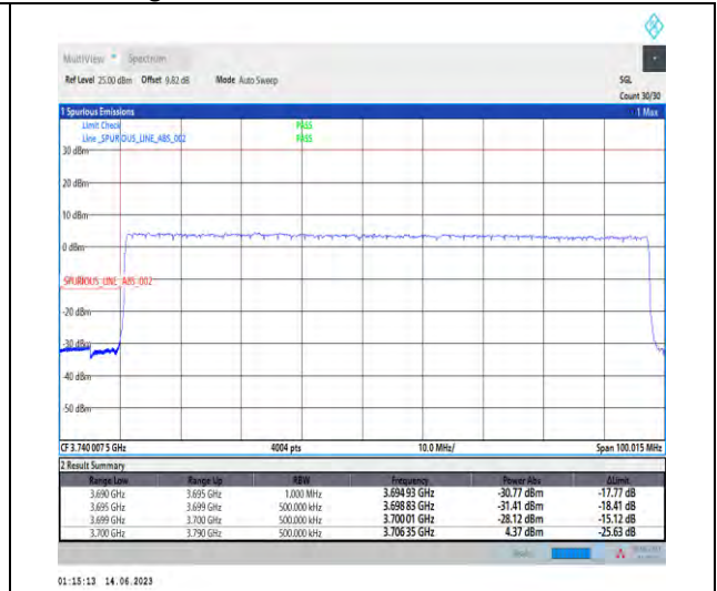
1-N77-3700-3980-PC1.5-30-90-L-3-DFT-PI2BPSK-Outer_Full-240@0-Ant1-1-PASS-see graph
