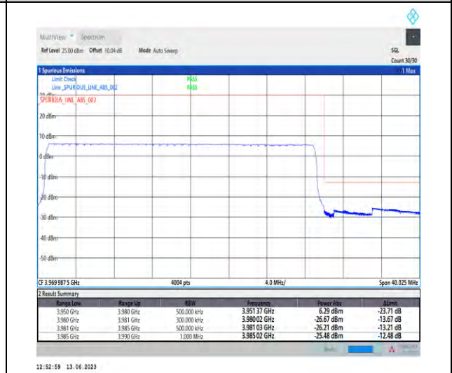
1-N77-3700-3980-PC1.5-30-30-H-6-CP-QPSK-Outer_Full-78@0-Ant1-1--PASS-see graph
