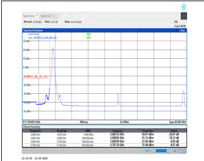
1-N77-3700-3980-PC1.5-30-50-L-1-DFT-PI2BPSK-Edge_1RB_Left-1@0-Ant1-1-PASS-see graph
