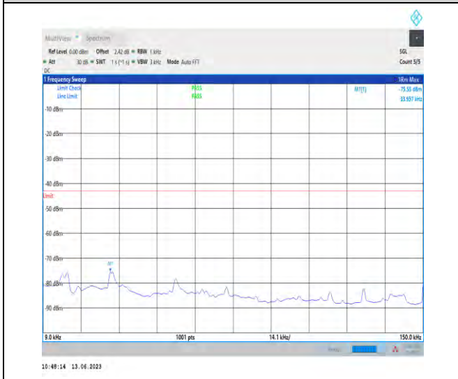
1-N77-3700-3980-PC1.5-30-100-H-1-N/A-DFT-QPS K-Edge_1RB_Left-1@0-0.009-0.15-Ant1-0.03--75.55--43-PASS
