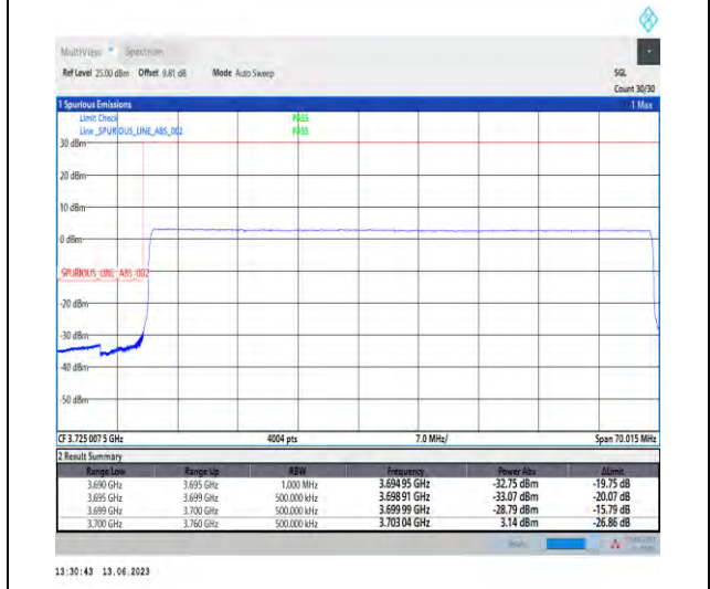
1-N77-3700-3980-PC1.5-30-60-L-6-CP-QPSK-Outer_Full-162@0-Ant1-1-PASS-see graph
