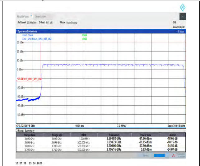
1-N77-3700-3980-PC1.5-30-60-L-3-DFT-PI2BPSK-Outer_Full-162@0-Ant1-1-PASS-see graph
