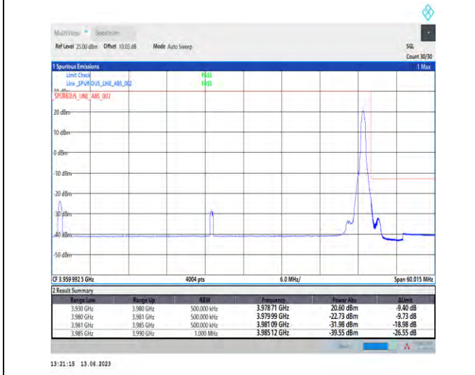
1-N77-3700-3980-PC1.5-30-50-H-5-CP-QPSK-Edge_1RB_Right-1@132-Ant1-1--PASS-see graph
