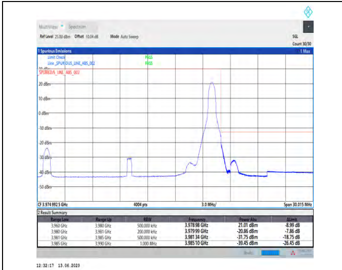
1-N77-3700-3980-PC1.5-30-20-H-2-DFT-PI2BPSK-Edge_1RB_Right-1@50-Ant1-1--PASS-see graph
