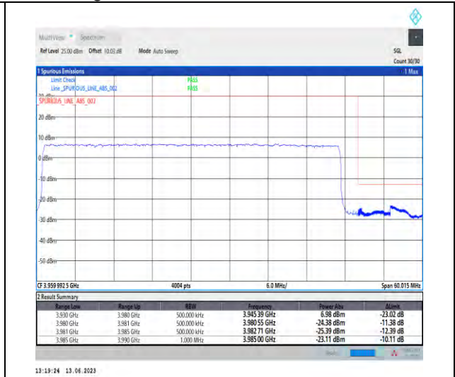
1-N77-3700-3980-PC1.5-30-50-H-3-DFT-PI2BPSK-Outer_Full-128@0-Ant1-1--PASS-see graph
