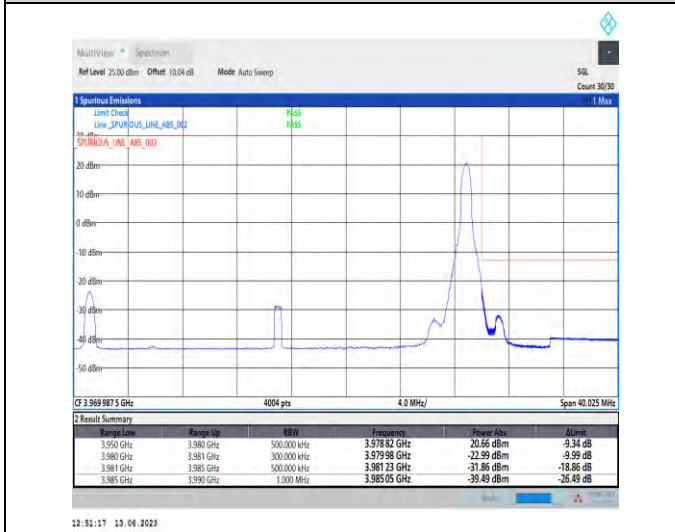
1-N77-3700-3980-PC1.5-30-30-H-5-CP-QPSK-Edge_1RB_Right-1@77-Ant1-1--PASS-see graph
