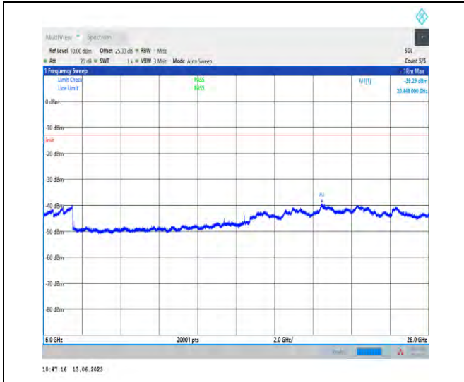
1-N77-3700-3980-PC1.5-30-100-M-1-N/A-DFT-QPS K-Edge_1RB_Left-1@0-6000-26000-Ant1-20448.00-39.29--13-PASS
