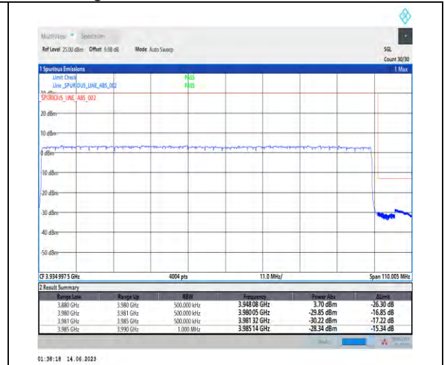
1-N77-3700-3980-PC1.5-30-100-H-3-DFT-PI2BPS K-Outer_Full-270@0-Ant1-1--PASS-see graph
