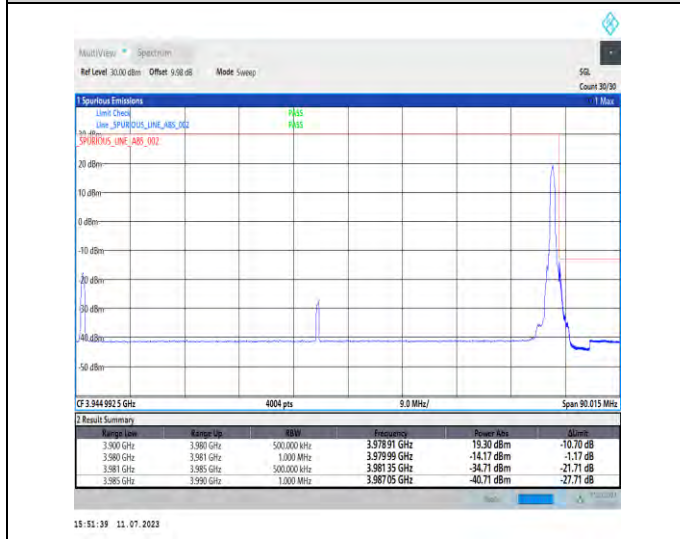
1-N77-3700-3980-PC1.5-30-80-H-5-CP-QPSK-Edge_1RB_Right-1@216-Ant1-1--PASS-see graph
