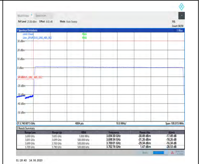
1-N77-3700-3980-PC1.5-30-90-L-6-CP-QPSK-Outer_Full-245@0-Ant1-1-PASS-see graph
