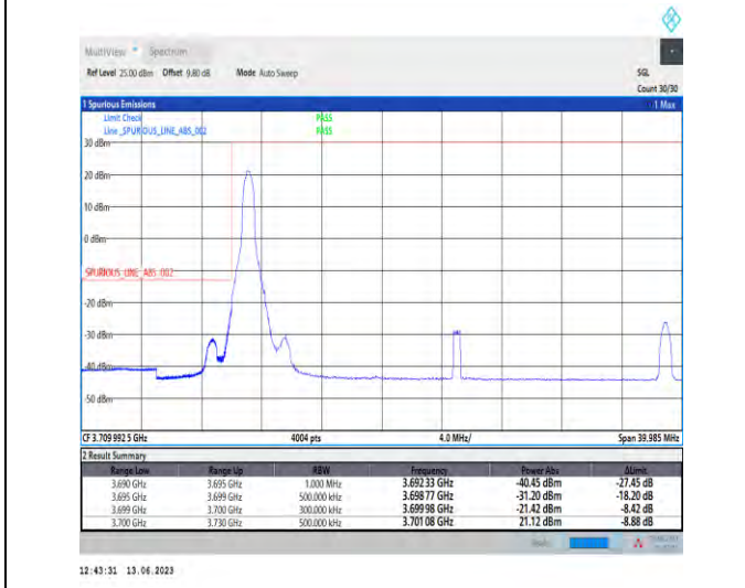
1-N77-3700-3980-PC1.5-30-30-L-4-CP-QPSK-Edge_1RB_Left-1@0-Ant1-1--PASS-see graph
