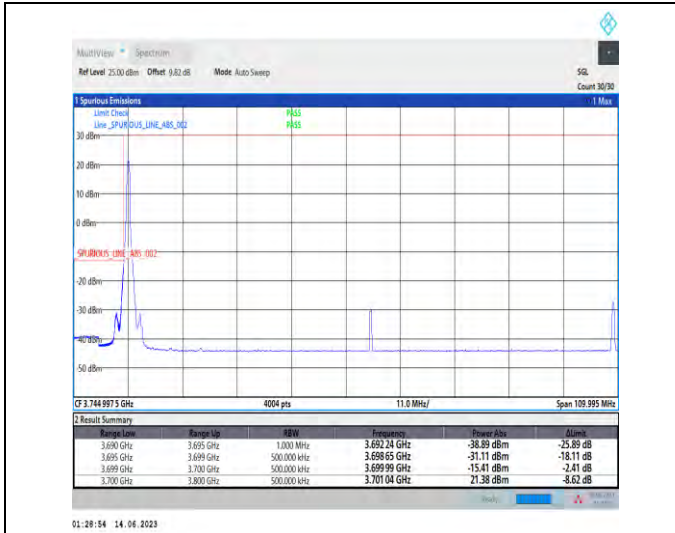
1-N77-3700-3980-PC1.5-30-100-L-1-DFT-PI2BPSK-E dge_1RB_Left-1@0-Ant1-1--PASS-see graph
