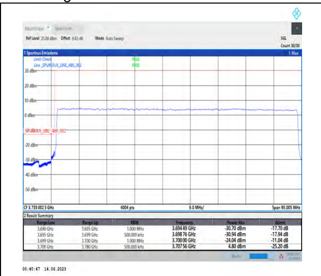
1-N77-3700-3980-PC1.5-30-80-L-3-DFT-PI2BPSK-Outer_Full-216@0-Ant1-1-PASS-see graph
