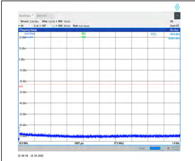
1-N77-3700-3980-PC1.5-30-100-H-1-N/A-DFT-QPS K-Edge_1RB_Left-1@0-30-1000-Ant1-36.60--66.03-23-PASS
