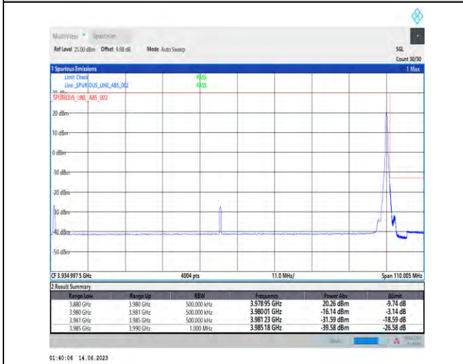
1-N77-3700-3980-PC1.5-30-100-H-5-CP-QPSK-Edge_1RB_Right-1@272-Ant1-1--PASS-see graph
