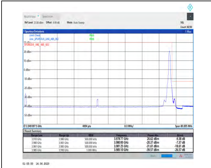
1-N77-3700-3980-PC1.5-30-70-H-2-DFT-PI2BPSK-Edge_1RB_Right-1@188-Ant1-1--PASS-see graph
