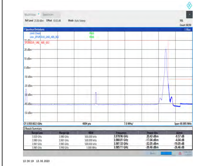
1-N77-3700-3980-PC1.5-30-60-H-5-CP-QPSK-Edge_1RB_Right-1@161-Ant1-1--PASS-see graph
