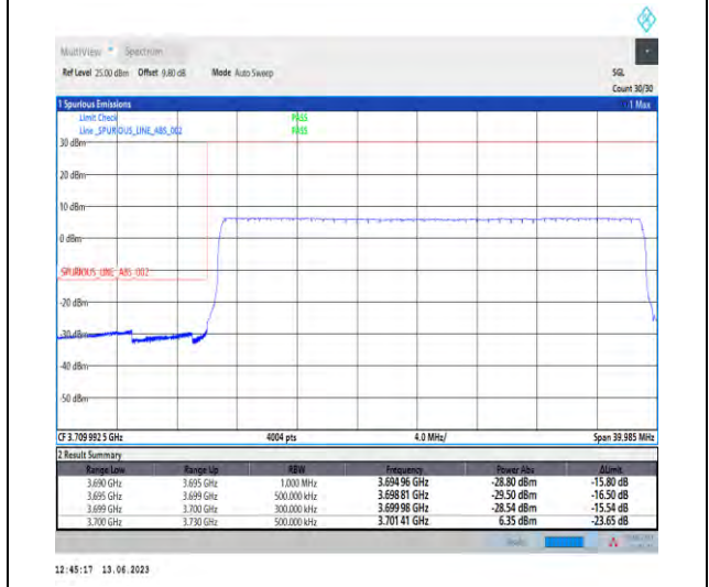
1-N77-3700-3980-PC1.5-30-30-L-6-CP-QPSK-Outer_Full-78@0-Ant1-1--PASS-see graph
