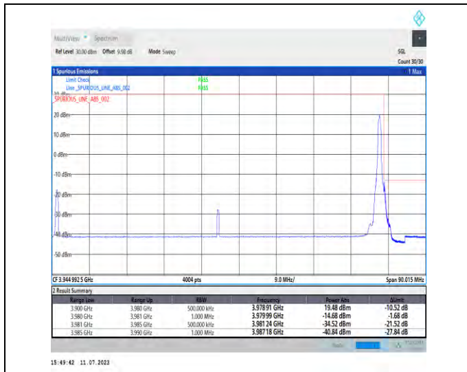
1-N77-3700-3980-PC1.5-30-80-H-2-DFT-PI2BPSK-Edge_1RB_Right-1@216-Ant1-1--PASS-see graph
