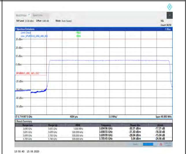
1-N77-3700-3980-PC1.5-30-40-L-6-CP-QPSK-Outer_Full-106@0-Ant1-1-PASS-see graph
