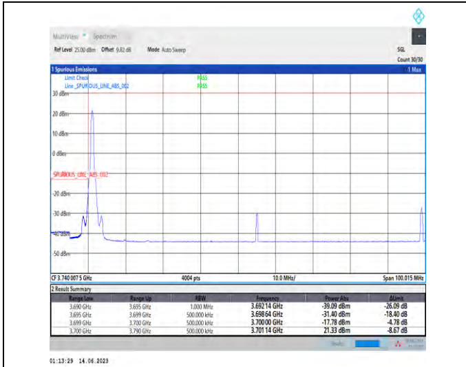
1-N77-3700-3980-PC1.5-30-90-L-1-DFT-PI2BPSK-Edge_1RB_Left-1@0-Ant1-1-PASS-see graph
