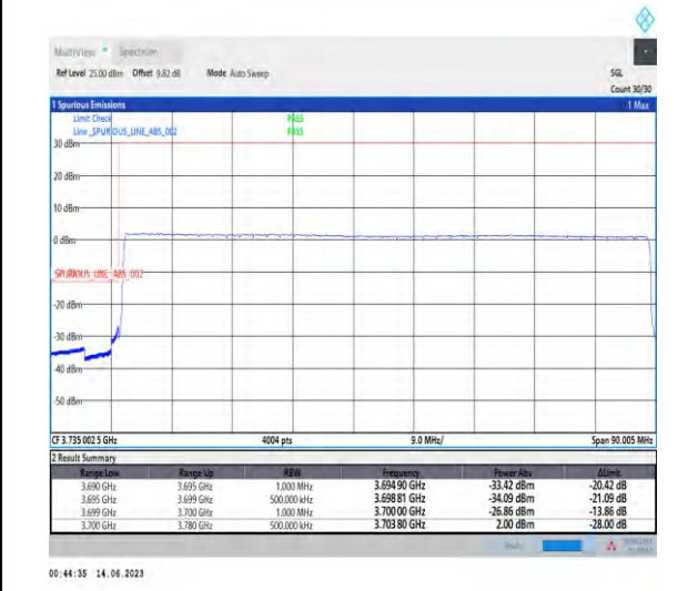
1-N77-3700-3980-PC1.5-30-80-L-6-CP-QPSK-Outer_Full-217@0-Ant1-1-PASS-see graph
