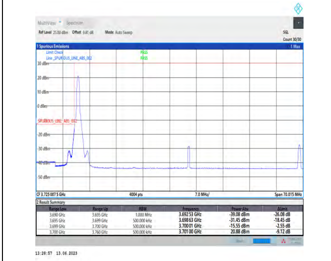
1-N77-3700-3980-PC1.5-30-60-L-4-CP-QPSK-Edge_1RB_Left-1@0-Ant1-1-PASS-see graph
