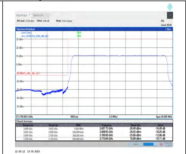
1-N77-3700-3980-PC1.5-30-20-L-3-DFT-PI2BPSK-Outer_Full-50@0-Ant1-1--PASS-see graph
