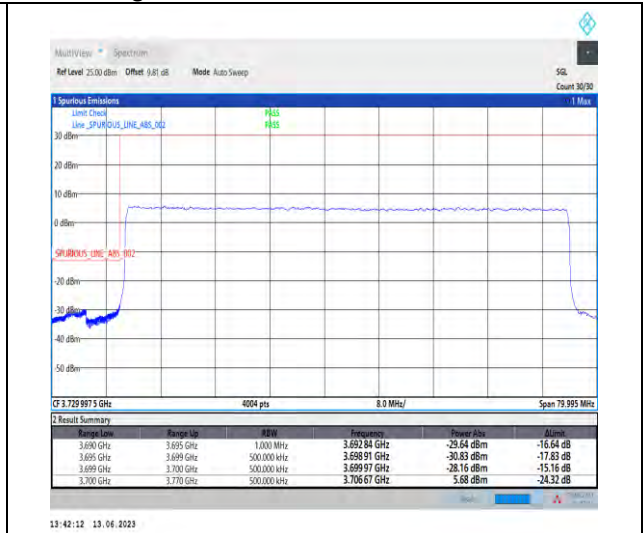
1-N77-3700-3980-PC1.5-30-70-L-3-DFT-PI2BPSK-Outer_Full-180@0-Ant1-1-PASS-see graph
