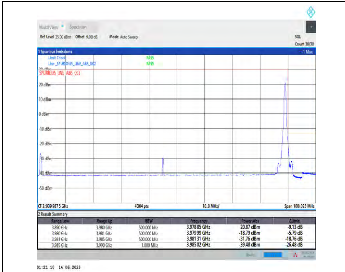
1-N77-3700-3980-PC1.5-30-90-H-2-DFT-PI2BPSK-Edge_1RB_Right-1@244-Ant1-1--PASS-see graph
