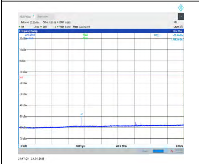
1-N77-3700-3980-PC1.5-30-100-M-1-N/A-DFT-QPS K-Edge_1RB_Left-1@0-1000-3000-Ant1-1764.20--5 1.45--13-PASS
