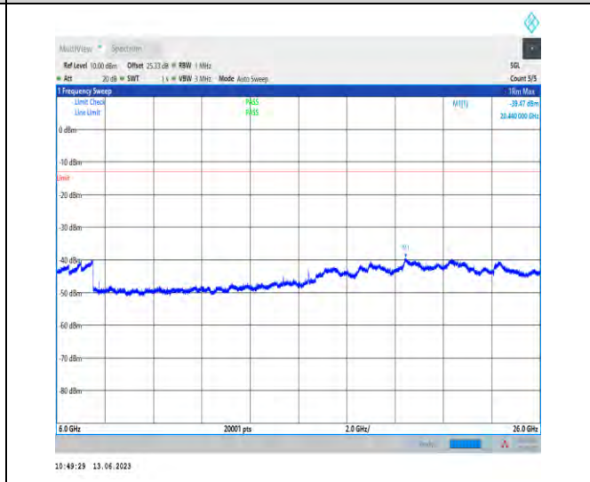
1-N77-3700-3980-PC1.5-30-100-H-1-N/A-DFT-QPS K-Edge_1RB_Left-1@0-6000-26000-Ant1-20440.00--39.47--13-PASS
