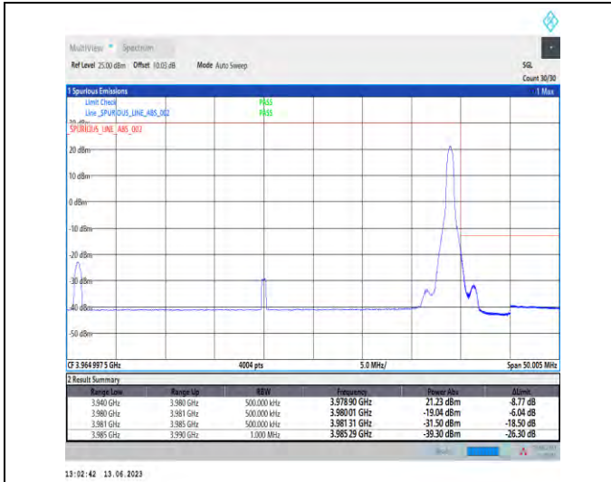
1-N77-3700-3980-PC1.5-30-40-H-2-DFT-PI2BPSK-Edge_1RB_Right-1@105-Ant1-1--PASS-see graph
