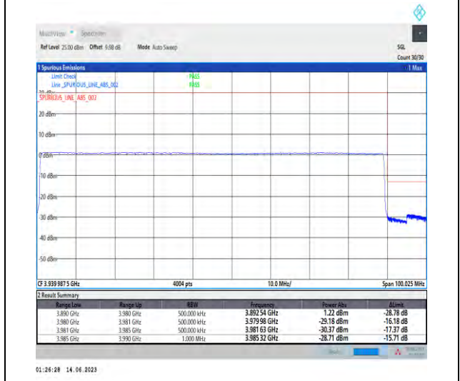
1-N77-3700-3980-PC1.5-30-90-H-6-CP-QPSK-Outer_Full-245@0-Ant1-1--PASS-see graph
