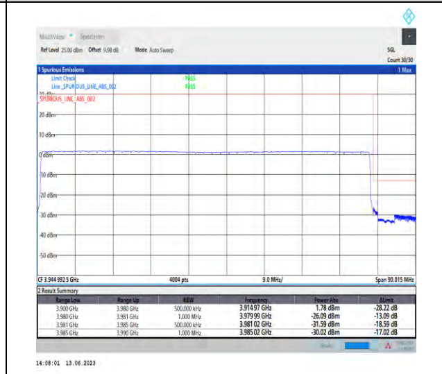
1-N77-3700-3980-PC1.5-30-80-H-6-CP-QPSK-Outer_Full-217@0-Ant1-1--PASS-see graph
