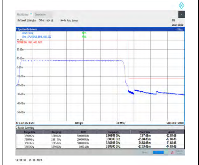
1-N77-3700-3980-PC1.5-30-20-H-6-CP-QPSK-Outer_Full-51@0-Ant1-1--PASS-see graph
