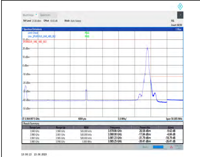
1-N77-3700-3980-PC1.5-30-40-H-5-CP-QPSK-Edge_1RB_Right-1@105-Ant1-1--PASS-see graph
