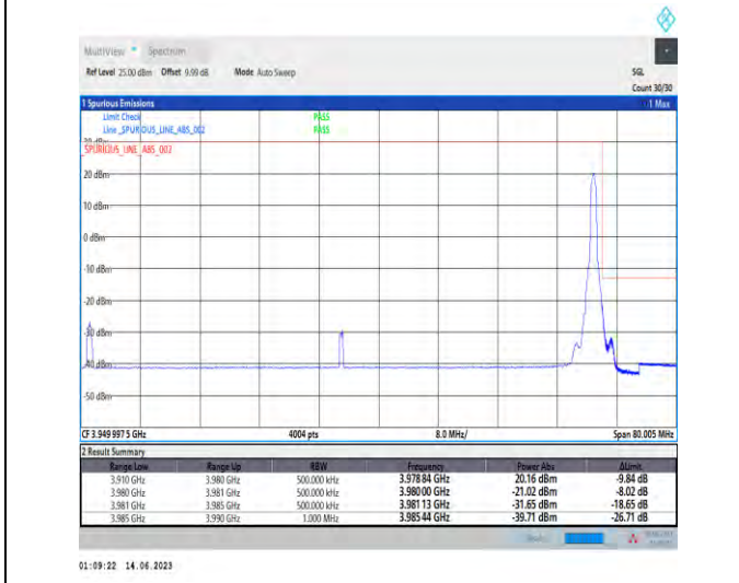
1-N77-3700-3980-PC1.5-30-70-H-5-CP-QPSK-Edge_1RB_Right-1@188-Ant1-1--PASS-see graph
