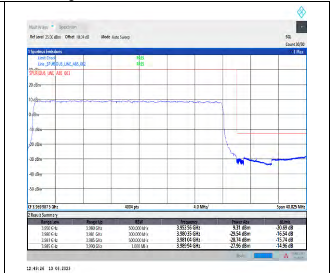
1-N77-3700-3980-PC1.5-30-30-H-3-DFT-PI2BPSK-Outer_Full-75@0-Ant1-1--PASS-see graph
