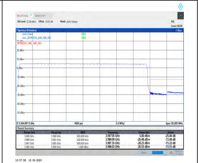
1-N77-3700-3980-PC1.5-30-40-H-6-CP-QPSK-Outer_Full-106@0-Ant1-1--PASS-see graph
