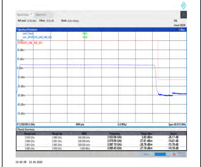
1-N77-3700-3980-PC1.5-30-50-H-6-CP-QPSK-Outer_Full-133@0-Ant1-1--PASS-see graph
