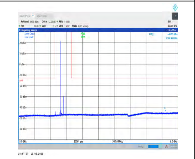
1-N77-3700-3980-PC1.5-30-100-M-1-N/A-DFT-QPS K-Edge_1RB_Left-1@0-3000-6000-Ant1-5760.30--4 3.95--13-PASS
