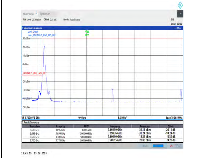
1-N77-3700-3980-PC1.5-30-70-L-4-CP-QPSK-Edge_1RB_Left-1@0-Ant1-1-PASS-see graph
