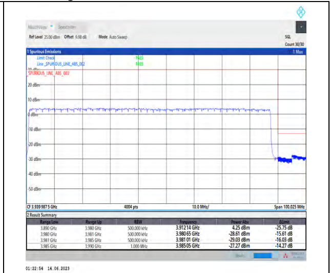
1-N77-3700-3980-PC1.5-30-90-H-3-DFT-PI2BPSK-Outer_Full-240@0-Ant1-1--PASS-see graph
