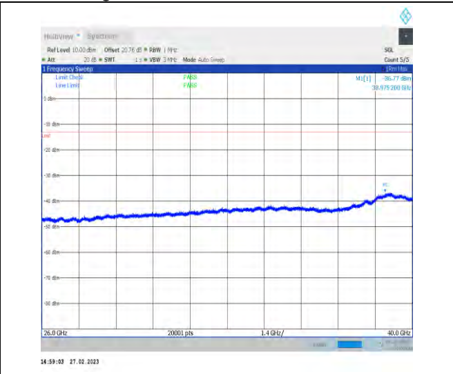
1-N77-3700-3980-PC1.5-30-100-M-1-N/A-DFT-QPS K-Edge_1RB_Left-1@0-26000-40000-Ant1-26000.00-49.68--13-PASS
