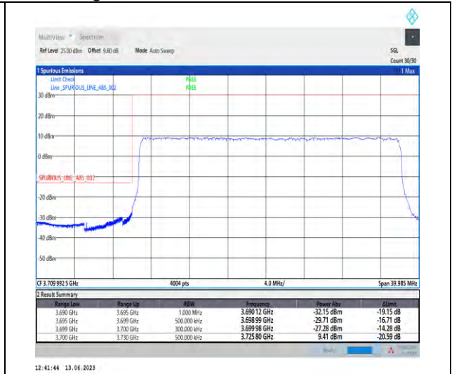
1-N77-3700-3980-PC1.5-30-30-L-3-DFT-PI2BPSK-Outer_Full-75@0-Ant1-1--PASS-see graph
