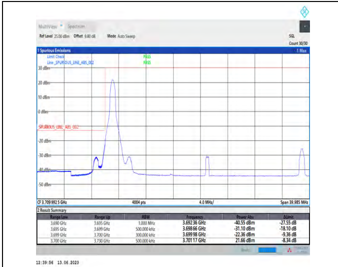
1-N77-3700-3980-PC1.5-30-30-L-1-DFT-PI2BPSK-Edge_1RB_Left-1@0-Ant1-1--PASS-see graph
