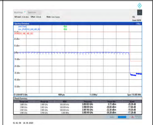
1-N77-3700-3980-PC1.5-30-100-H-6-CP-QPSK-O uter_Full-273@0-Ant1-1--PASS-see graph
