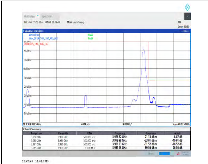
1-N77-3700-3980-PC1.5-30-30-H-2-DFT-PI2BPSK-Edge_1RB_Right-1@77-Ant1-1--PASS-see graph
