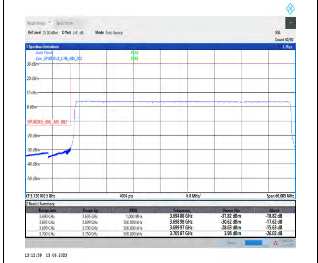
1-N77-3700-3980-PC1.5-30-50-L-6-CP-QPSK-Outer_Full-133@0-Ant1-1-PASS-see graph
