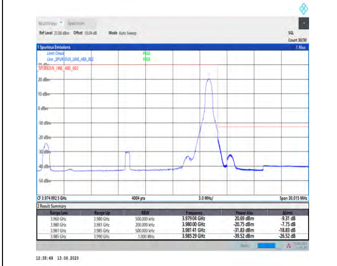
1-N77-3700-3980-PC1.5-30-20-H-5-CP-QPSK-Edge_1RB_Right-1@50-Ant1-1--PASS-see graph
