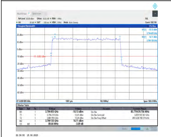
1-N77-3700-3980-PC1.5-30-90-M-3-DFT-16QAM-Outer_Full-240@0-Ant1-85.78-89.640-≤90-PASS
