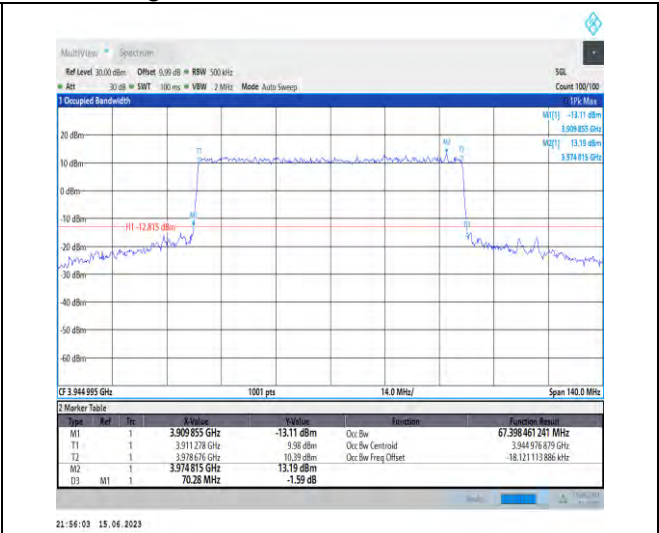
1-N77-3700-3980-PC1.5-30-70-H-7-CP-16QAM-Outer_Full-189@0-Ant1-67.398-70.280-≤70-PASS
