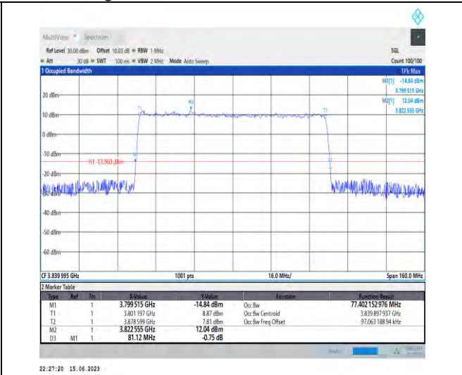
1-N77-3700-3980-PC1.5-30-80-M-9-CP-256QAM-Outer_Full-217@0-Ant1-77.402-81.120-<80-PASS
