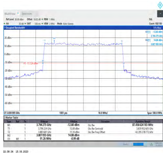
1-N77-3700-3980-PC1.5-30-90-M-8-CP-64QAM-Outer_Full-245@0-Ant1-87.457-91.260-≤90-PASS
