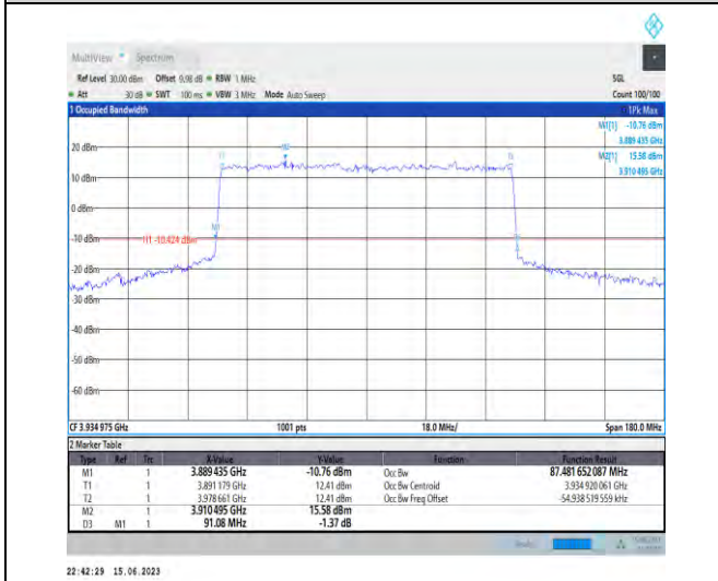
1-N77-3700-3980-PC1.5-30-90-H-6-CP-QPSK-Outer_Full-245@0-Ant1-87.482-91.080-≤90-PASS
