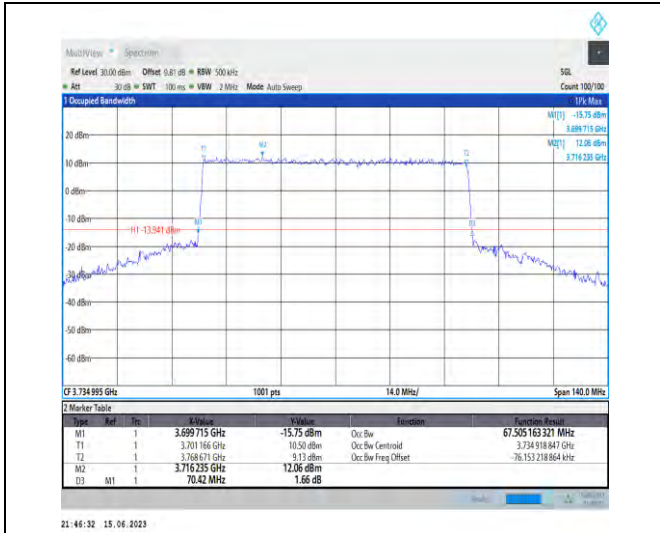
1-N77-3700-3980-PC1.5-30-70-L-8-CP-64QAM-Outer_Full-189@0-Ant1-67.505-70.420-≤70-PASS
