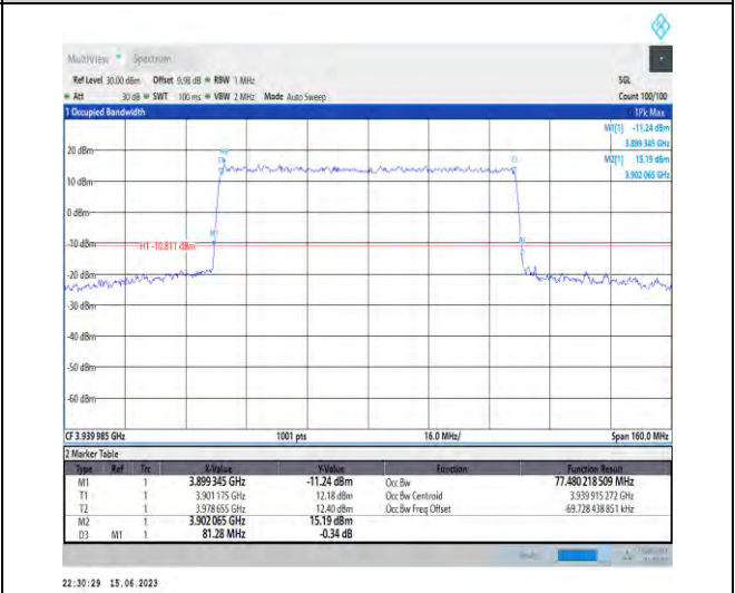
1-N77-3700-3980-PC1.5-30-80-H-6-CP-QPSK-Outer_Full-217@0-Ant1-77.48-81.280-≤80-PASS
