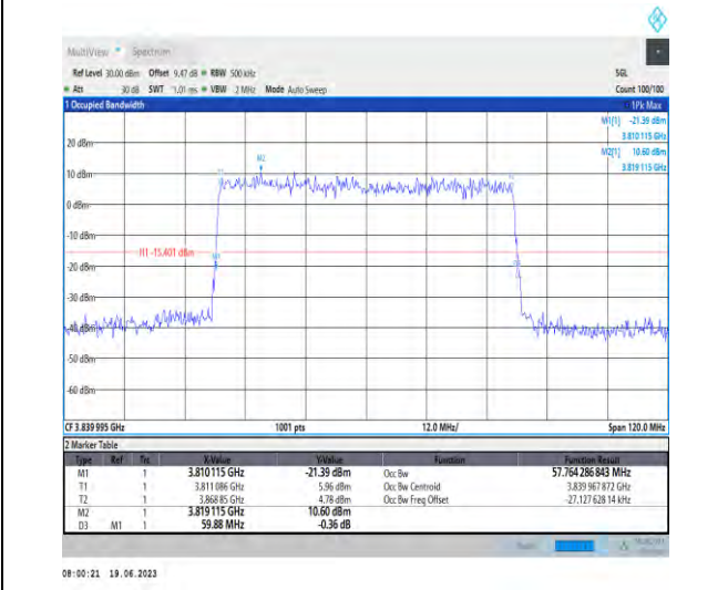
1-N77-3700-3980-PC1.5-30-60-M-5-DFT-256QAM-Outer_Full-162@0-Ant1-57.764-59.88-≤60-PASS
