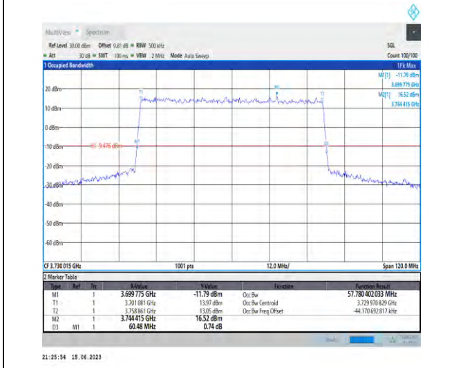
1-N77-3700-3980-PC1.5-30-60-L-1-DFT-QPSK-Out er_Full-162@0-Ant1-57.78-60.480-≤60-PASS
