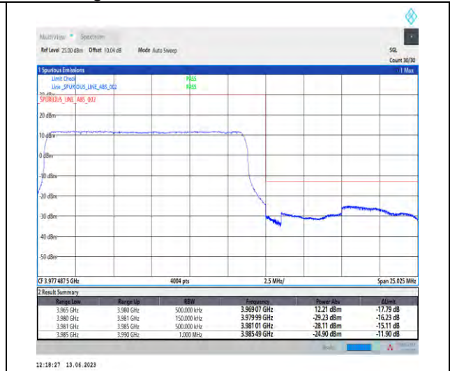
1-N77-3700-3980-PC1.5-30-15-H-3-DFT-PI2BPSK-Outer_Full-36@0-Ant1-1--PASS-see graph
