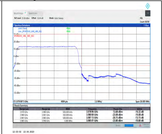
1-N77-3700-3980-PC1.5-30-10-H-3-DFT-PI2BPSK-Outer_Full-24@0-Ant1-1--PASS-see graph
