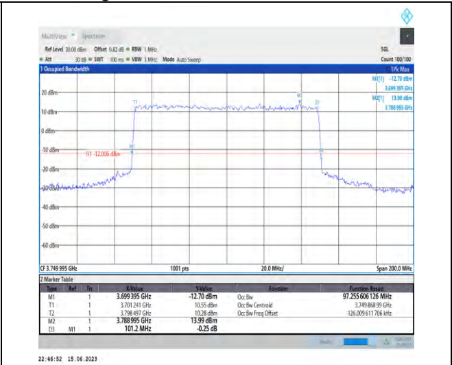
1-N77-3700-3980-PC1.5-30-100-L-8-CP-64QAM-Out_Full-273@0-Ant1-97.256-101.200-≤100-PASS
