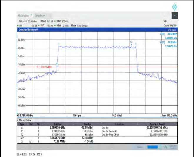
1-N77-3700-3980-PC1.5-30-70-L-7-CP-16QAM-Out er_Full-189@0-Ant1-67.359-70.280-≤70-PASS
