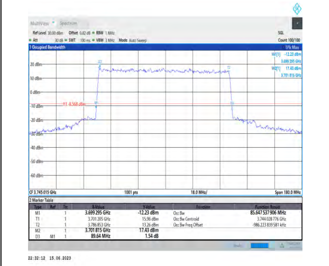
1-N77-3700-3980-PC1.5-30-90-L-1-DFT-QPSK-Outer_Full-240@0-Ant1-85.648-89.640-≤90-PASS
