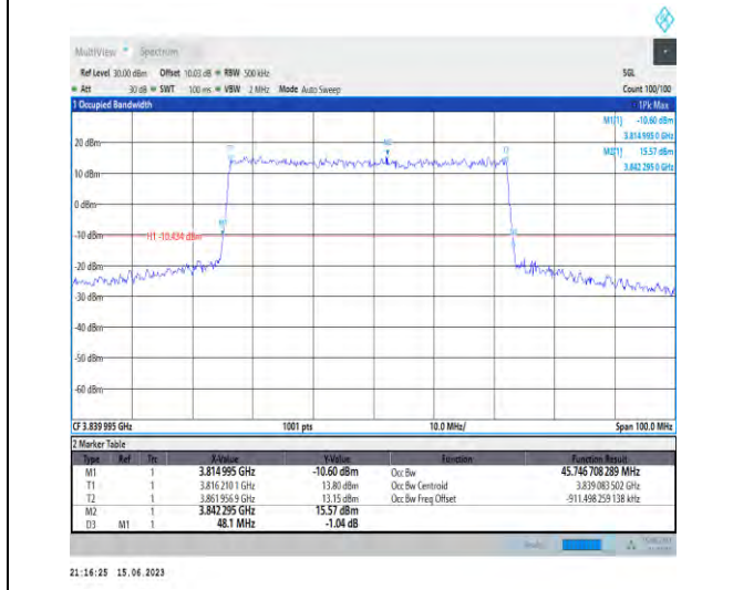
1-N77-3700-3980-PC1.5-30-50-M-3-DFT-16QAM-Outer_Full-128@0-Ant1-45.747-48.100-≤50-PASS
