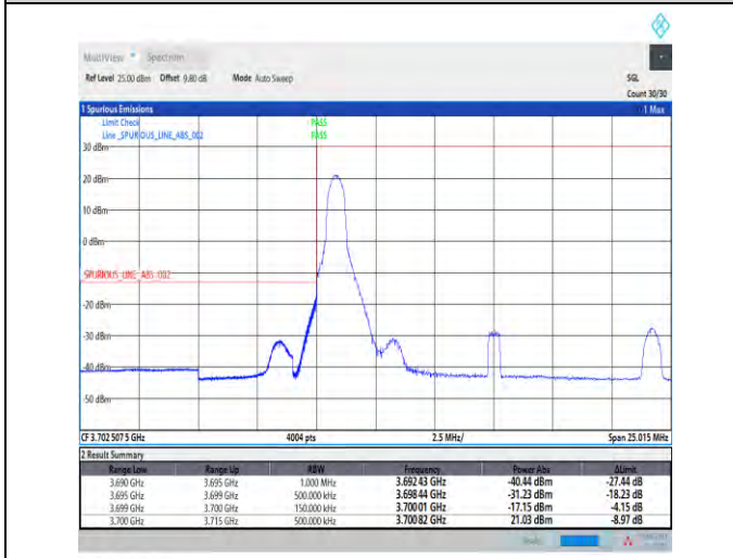
1-N77-3700-3980-PC1.5-30-15-L-1-DFT-PI2BPSK-Edge_1RB_Left-1@0-Ant1-1--PASS-see graph
