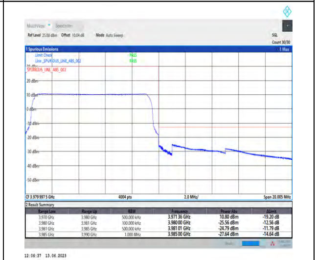
1-N77-3700-3980-PC1.5-30-10-H-6-CP-QPSK-Outer_Full-24@0-Ant1-1--PASS-see graph
