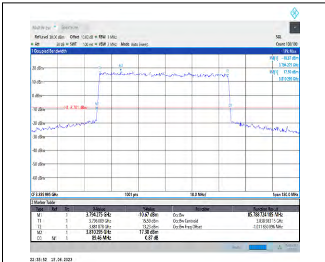
1-N77-3700-3980-PC1.5-30-90-M-1-DFT-QPSK-Out er_Full-240@0-Ant1-85.789-89.460-≤90-PASS
