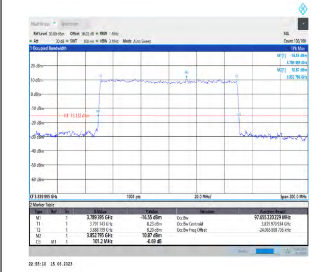
1-N77-3700-3980-PC1.5-30-100-M-9-CP-256QAM-Outer_Full-273@0-Ant1-97.655-101.200-≤100-PASS
