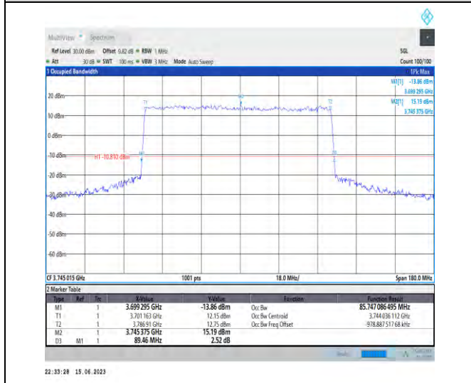
1-N77-3700-3980-PC1.5-30-90-L-4-DFT-64QAM-Outer_Full-240@0-Ant1-85.747-89.460-≤90-PASS
