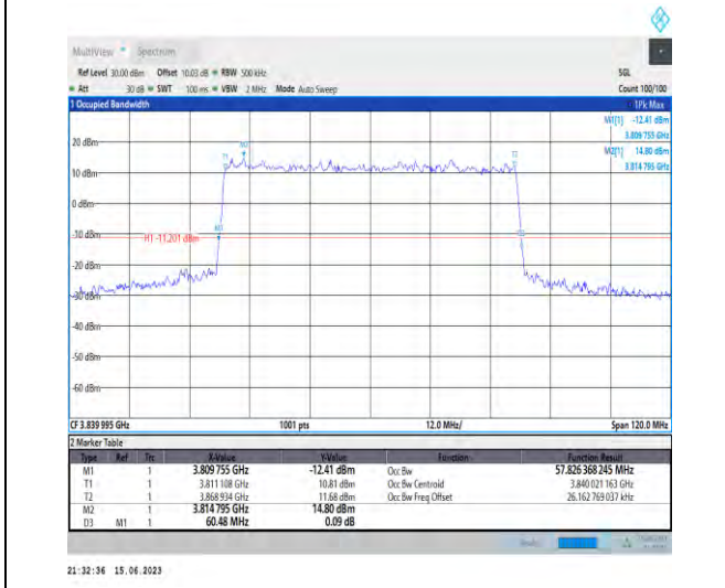
1-N77-3700-3980-PC1.5-30-60-M-4-DFT-64QAM-Outer_Full-162@0-Ant1-57.826-60.480-≤60-PASS
