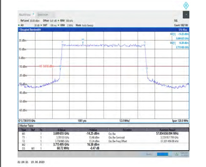
1-N77-3700-3980-PC1.5-30-60-L-2-DFT-PI2BPSK-Out er_Full-162@0-Ant1-57.855-60.720-≤60-PASS
