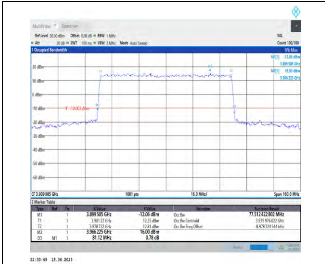
1-N77-3700-3980-PC1.5-30-80-H-7-CP-16QAM-Out er_Full-217@0-Ant1-77.512-81.120-≤80-PASS
