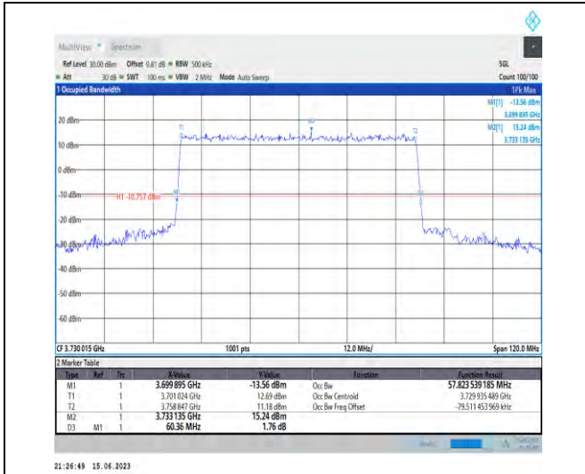
1-N77-3700-3980-PC1.5-30-60-L-3-DFT-16QAM-Out er_Full-162@0-Ant1-57.824-60.360-≤60-PASS
