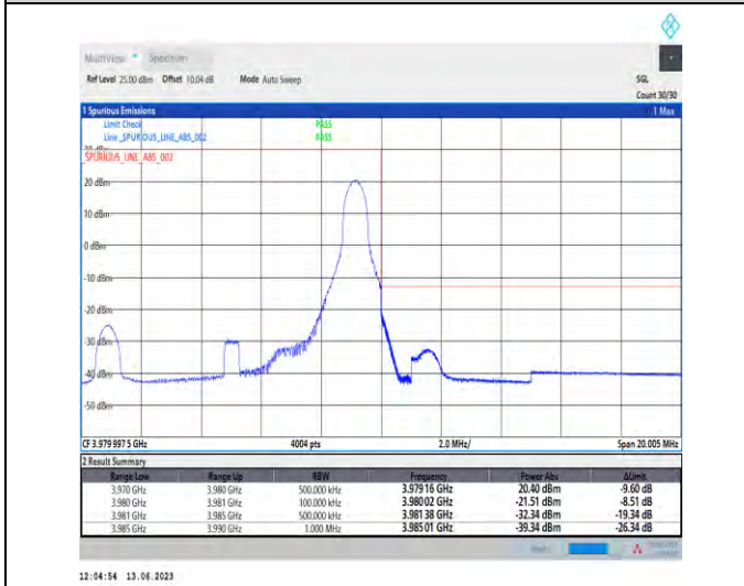
1-N77-3700-3980-PC1.5-30-10-H-5-CP-QPSK-Edge_1RB_Right-1@23-Ant1-1--PASS-see graph
