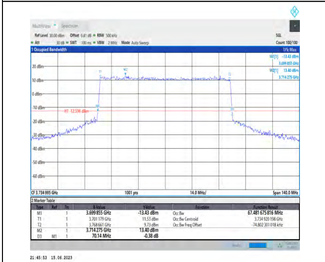
1-N77-3700-3980-PC1.5-30-70-L-6-CP-QPSK-Outer _Full-189@0-Ant1-67.482-70.140-≤70-PASS
