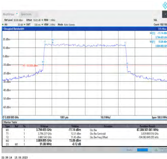
1-N77-3700-3980-PC1.5-30-90-M-7-CP-16QAM-Outer_Full-245@0-Ant1-87.307-91.080-≤90-PASS
