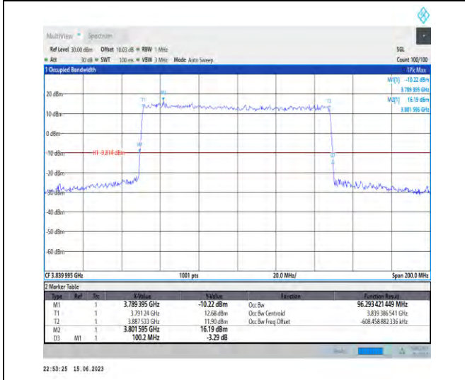
1-N77-3700-3980-PC1.5-30-100-M-4-DFT-64QAM-Outer_Full-270@0-Ant1-96.293-100.200-≤100-PASS
