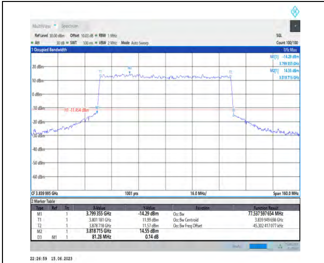
1-N77-3700-3980-PC1.5-30-80-M-8-CP-64QAM-Out er_Full-217@0-Ant1-77.538-81.280-<80-PASS
