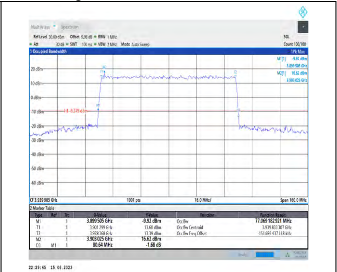
1-N77-3700-3980-PC1.5-30-80-H-4-DFT-64QAM-Outer_Full-216@0-Ant1-77.069-80.640-≤80-PASS
