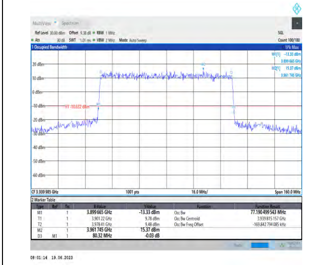
1-N77-3700-3980-PC1.5-30-80-H-1-DFT-QPSK-Outer_Full-216@0-Ant1-77.190-80.32-<80-PASS
