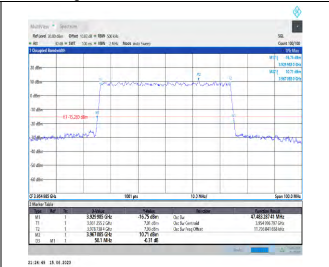
1-N77-3700-3980-PC1.5-30-50-H-9-CP-256QAM-Out er_Full-133@0-Ant1-47.483-50.100-≤50-PASS
