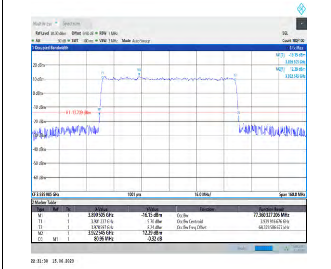
1-N77-3700-3980-PC1.5-30-80-H-9-CP-256QAM-Out er_Full-217@0-Ant1-77.36-80.960-≤80-PASS
