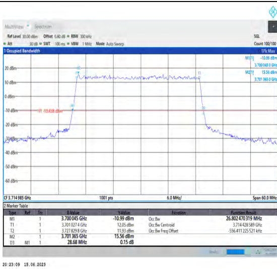
1-N77-3700-3980-PC1.5-30-30-L-4-DFT-64QAM-Out er_Full-75@0-Ant1-26.802-28.680-≤30-PASS
