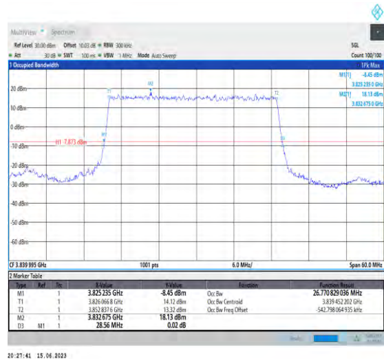
1-N77-3700-3980-PC1.5-30-30-M-2-DFT-PI2BPSK-Outer_Full-75@0-Ant1-26.771-28.560-≤30-PASS
