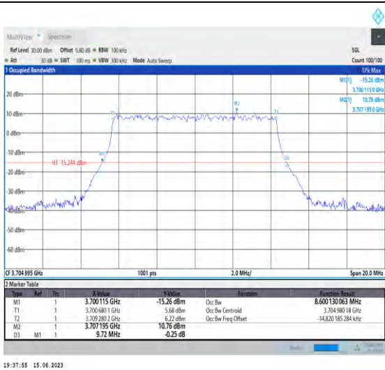
1-N77-3700-3980-PC1.5-30-10-L-9-CP-256QAM-Out er_Full-24@0-Ant1-8.6-9.720-≤10-PASS
