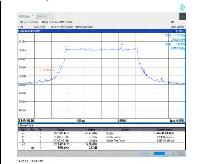
1-N77-3700-3980-PC1.5-30-10-H-8-CP-64QAM-Out er_Full-24@0-Ant1-8.586-9.960-≤10-PASS
