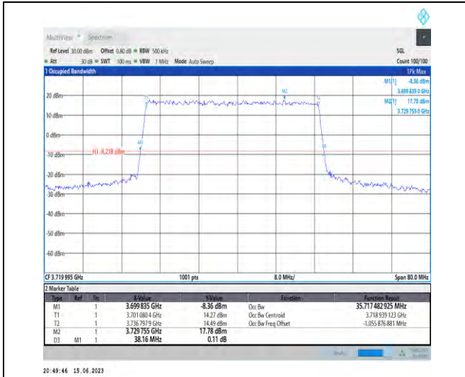
1-N77-3700-3980-PC1.5-30-40-L-1-DFT-QPSK-Outer_Full-100@0-Ant1-35.717-38.160-≤40-PASS
