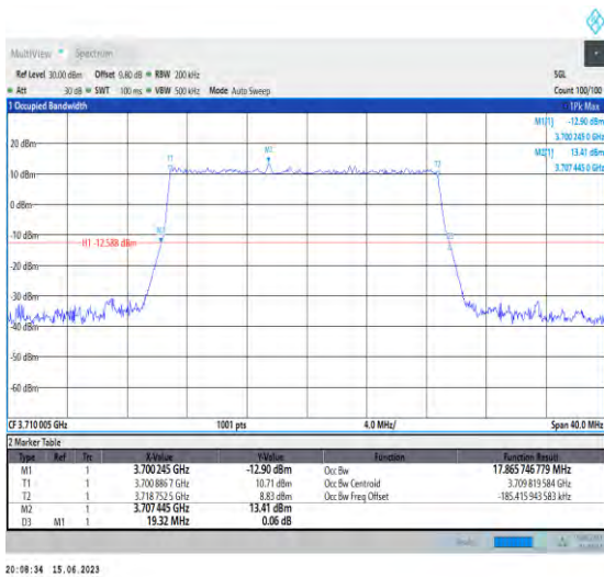
1-N77-3700-3980-PC1.5-30-20-L-5-DFT-256QAM-O uter_Full-50@0-Ant1-17.866-19.320-≤20-PASS
