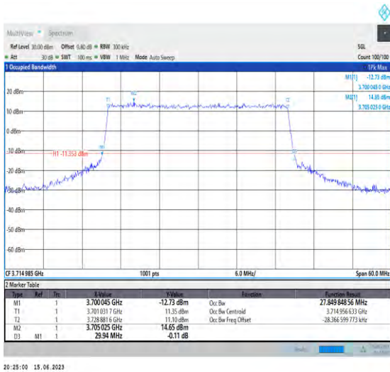
1-N77-3700-3980-PC1.5-30-30-L-6-CP-QPSK-Outer _Full-78@0-Ant1-27.85-29.940-≤30-PASS
