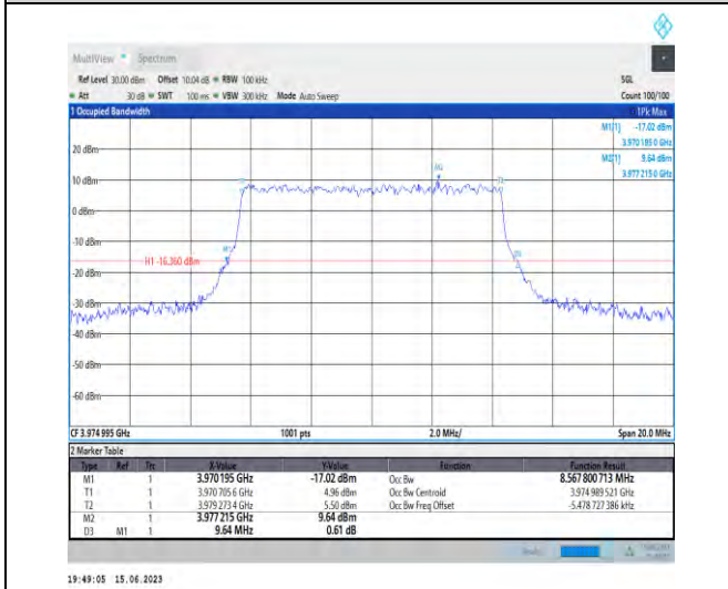
1-N77-3700-3980-PC1.5-30-10-H-9-CP-256QAM-Out er_Full-24@0-Ant1-8.568-9.640-≤10-PASS
