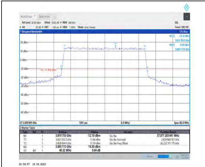
1-N77-3700-3980-PC1.5-30-40-M-8-CP-64QAM-Out er_Full-106@0-Ant1-37.871-40.320-≤40-PASS
