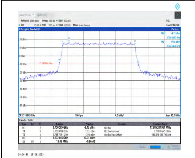
1-N77-3700-3980-PC1.5-30-20-L-1-DFT-QPSK-Oute r_Full-50@0-Ant1-17.885-19.480-≤20-PASS
