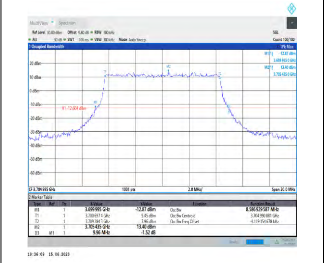
1-N77-3700-3980-PC1.5-30-10-L-8-CP-64QAM-Outer_Full-24@0-Ant1-8.587-9.960-≤10-PASS
