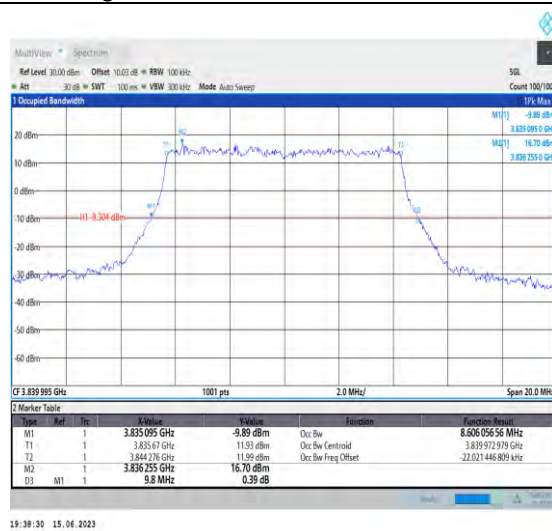
1-N77-3700-3980-PC1.5-30-10-M-1-DFT-QPSK-Out er_Full-24@0-Ant1-8.606-9.800-≤10-PASS
