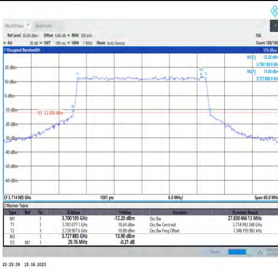
1-N77-3700-3980-PC1.5-30-30-L-8-CP-64QAM-Outer_Full-78@0-Ant1-27.83-29.760-≤30-PASS
