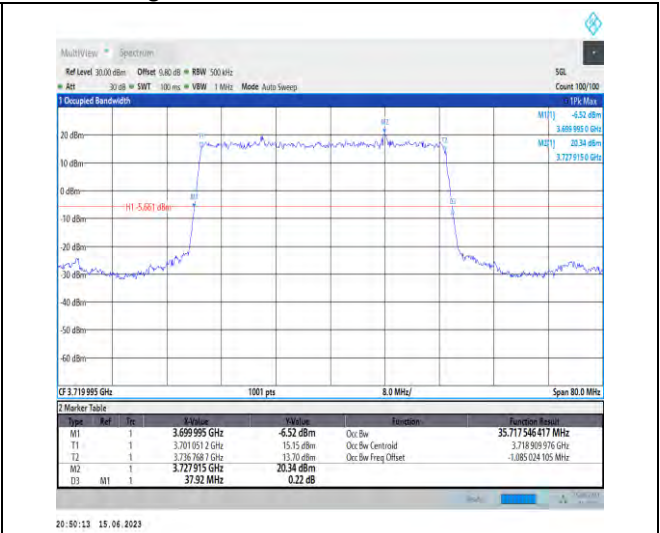
1-N77-3700-3980-PC1.5-30-40-L-2-DFT-PI2BPSK-Outer_Full-100@0-Ant1-35.718-37.920-≤40-PASS
