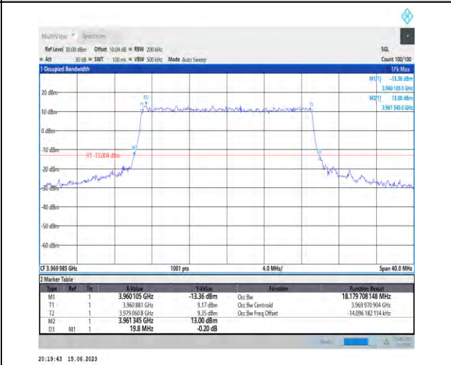
1-N77-3700-3980-PC1.5-30-20-H-8-CP-64QAM-Outer_Full-51@0-Ant1-18.18-19.800-≤20-PASS
