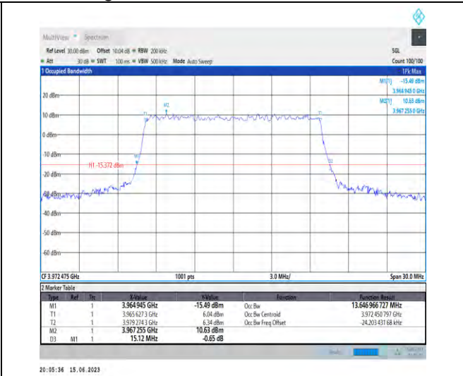
1-N77-3700-3980-PC1.5-30-15-H-9-CP-256QAM-Ou ter_Full-38@0-Ant1-13.647-15.120-≤15-PASS
