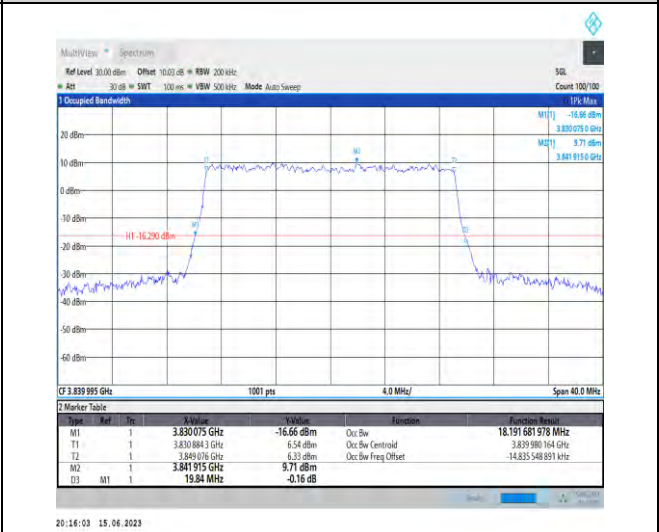
1-N77-3700-3980-PC1.5-30-20-M-9-CP-256QAM-Outer_Full-51@0-Ant1-18.192-19.840-≤20-PASS
