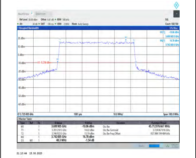
1-N77-3700-3980-PC1.5-30-50-L-1-DFT-QPSK-Outer_Full-128@0-Ant1-45.713-48.300-≤50-PASS
