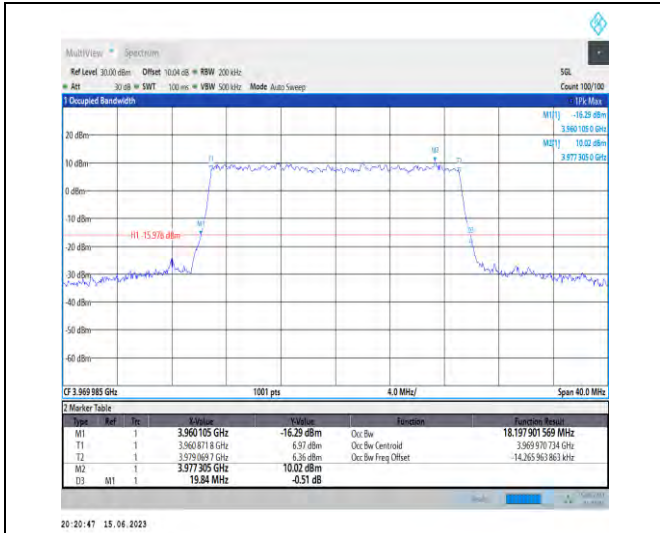
1-N77-3700-3980-PC1.5-30-20-H-9-CP-256QAM-Outer_Full-51@0-Ant1-18.198-19.840-≤20-PASS
