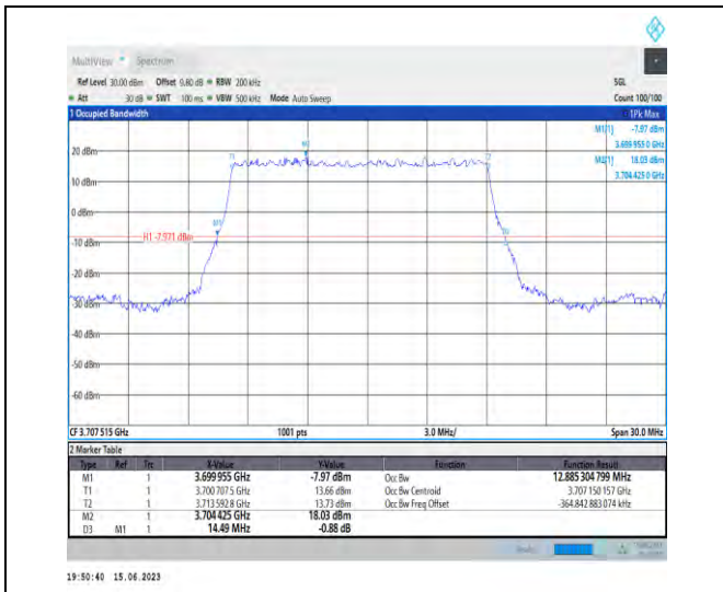
1-N77-3700-3980-PC1.5-30-15-L-2-DFT-PI2BPSK-Outer_Full-36@0-Ant1-12.885-14.490-≤15-PASS
