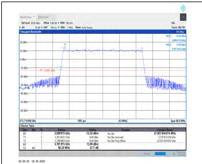
1-N77-3700-3980-PC1.5-30-40-L-9-CP-256QAM-Out er_Full-106@0-Ant1-37.858-40.240-≤40-PASS
