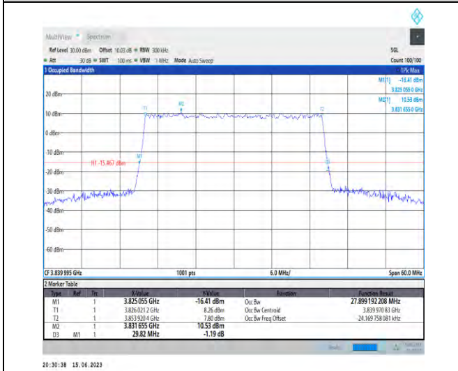
1-N77-3700-3980-PC1.5-30-30-M-9-CP-256QAM-Out er_Full-78@0-Ant1-27.899-29.820-≤30-PASS
