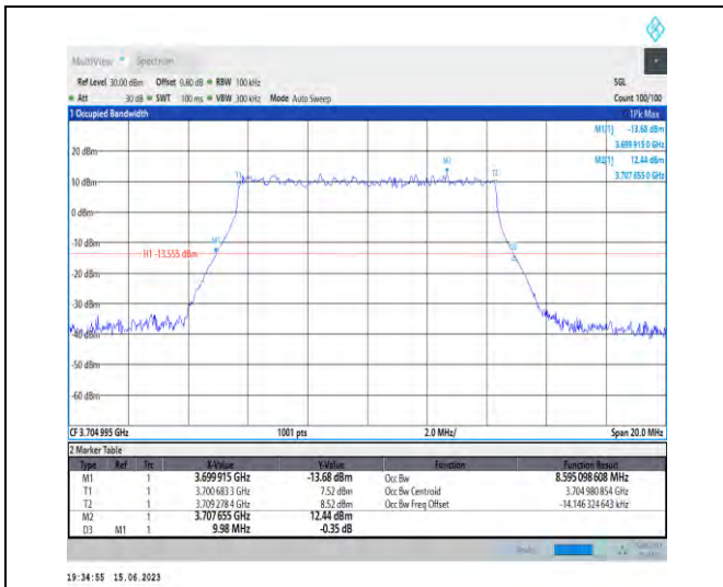
1-N77-3700-3980-PC1.5-30-10-L-5-DFT-256QAM-Outer_Full-24@0-Ant1-8.595-9.980-≤10-PASS
