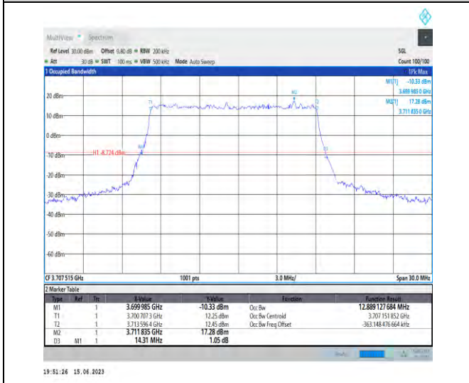
1-N77-3700-3980-PC1.5-30-15-L-4-DFT-64QAM-Out er_Full-36@0-Ant1-12.889-14.310-≤15-PASS
