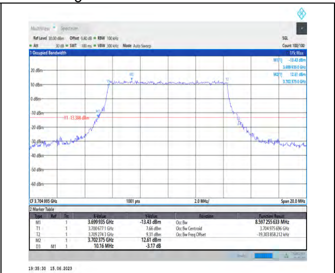
1-N77-3700-3980-PC1.5-30-10-L-6-CP-QPSK-Outer_Full-24@0-Ant1-8.597-10.160-≤10-PASS
