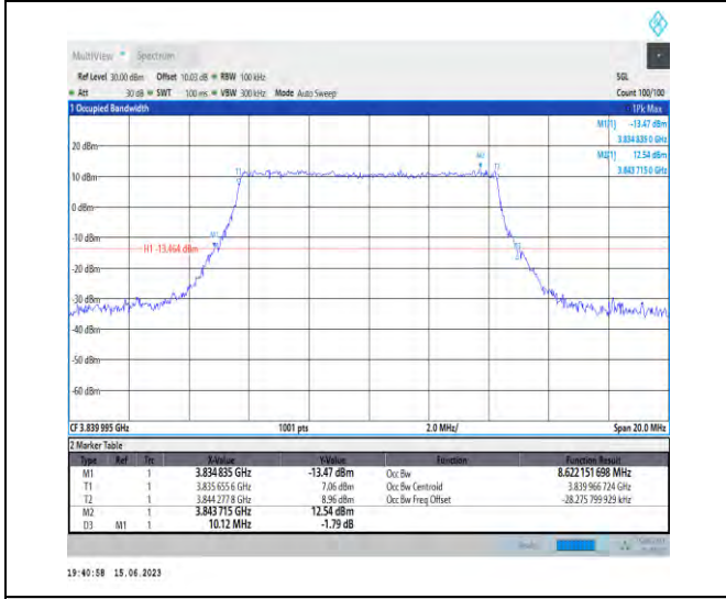
1-N77-3700-3980-PC1.5-30-10-M-6-CP-QPSK-Outer_Full-24@0-Ant1-8.622-10.120-≤10-PASS
