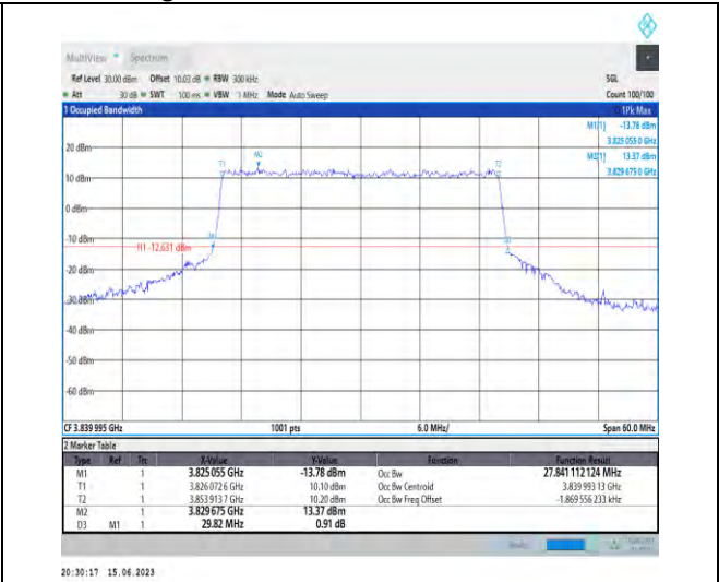
1-N77-3700-3980-PC1.5-30-30-M-8-CP-64QAM-Out er_Full-78@0-Ant1-27.841-29.820-≤30-PASS
