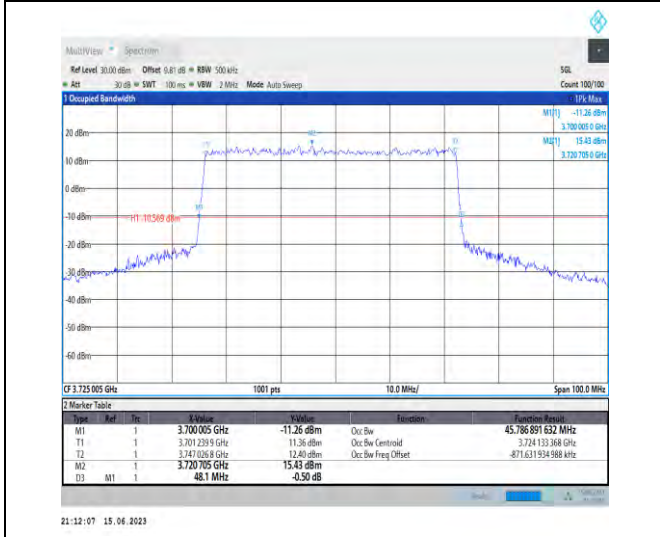
1-N77-3700-3980-PC1.5-30-50-L-4-DFT-64QAM-Out er_Full-128@0-Ant1-45.787-48.100-≤50-PASS
