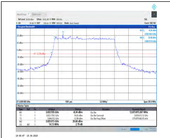
1-N77-3700-3980-PC1.5-30-15-M-1-DFT-QPSK-Out er_Full-36@0-Ant1-12.874-14.130-≤15-PASS
