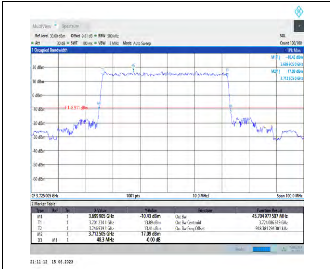
1-N77-3700-3980-PC1.5-30-50-L-2-DFT-PI2BPSK-Outer_Full-128@0-Ant1-45.705-48.300-≤50-PASS
