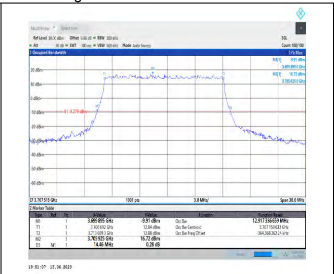
1-N77-3700-3980-PC1.5-30-15-L-3-DFT-16QAM-Outer_Full-36@0-Ant1-12.917-14.460-≤15-PASS
