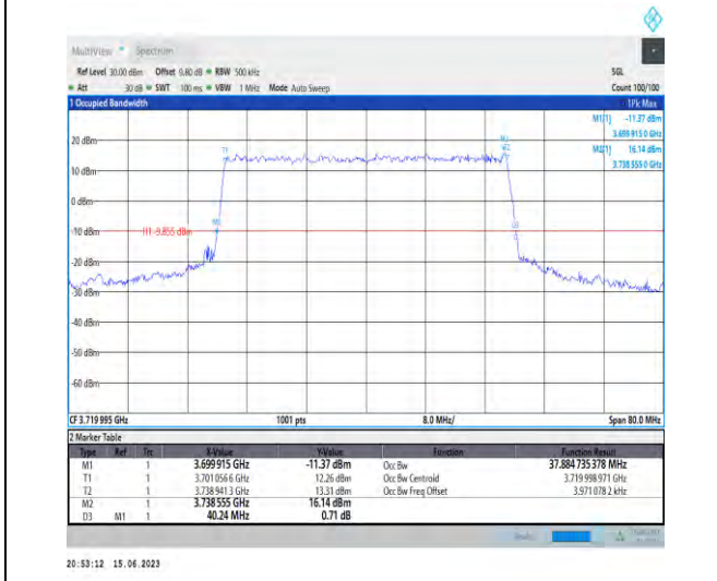
1-N77-3700-3980-PC1.5-30-40-L-7-CP-16QAM-Outer_Full-106@0-Ant1-37.885-40.240-≤40-PASS
