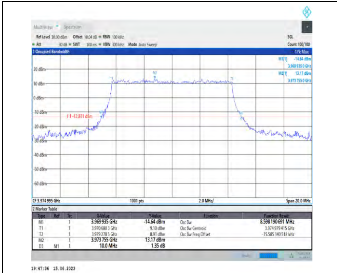
1-N77-3700-3980-PC1.5-30-10-H-7-CP-16QAM-Out er_Full-24@0-Ant1-8.598-10.000-≤10-PASS
