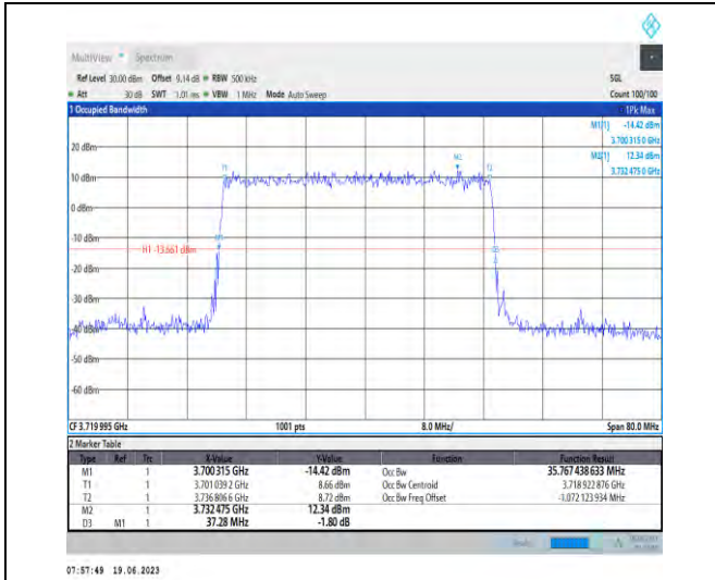
1-N77-3700-3980-PC1.5-30-40-L-5-DFT-256QAM-Outer_Full-100@0-Ant1-35.767-37.280-≤40-PASS
