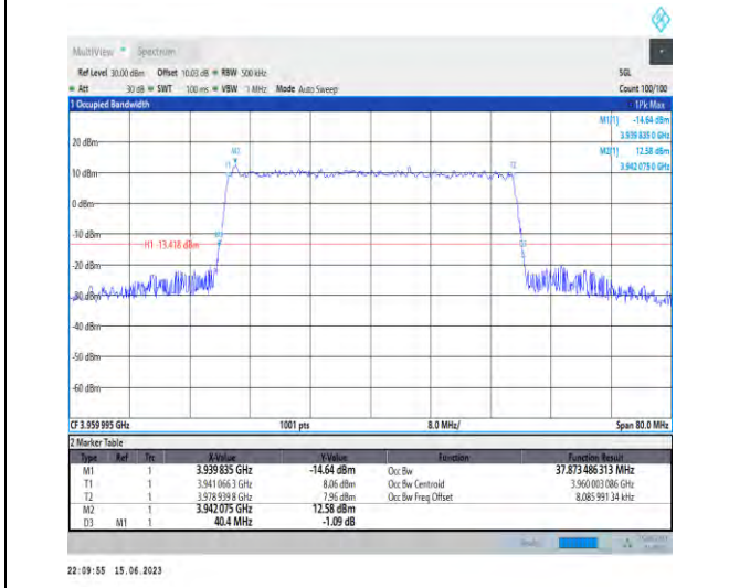
1-N77-3700-3980-PC1.5-30-40-H-9-CP-256QAM-Out er_Full-106@0-Ant1-37.873-40.400-≤40-PASS
