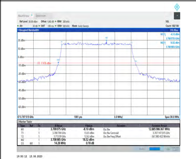
1-N77-3700-3980-PC1.5-30-15-L-1-DFT-QPSK-Outer er_Full-36@0-Ant1-12.886-14.280-≤15-PASS
