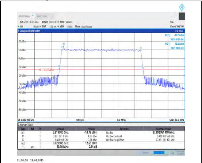
1-N77-3700-3980-PC1.5-30-40-M-9-CP-256QAM-Outer_Full-106@0-Ant1-37.893-40.160-≤40-PASS
