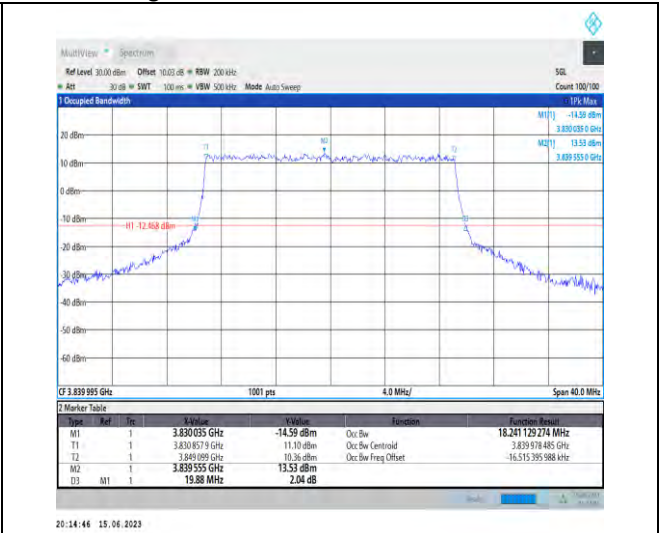
1-N77-3700-3980-PC1.5-30-20-M-7-CP-16QAM-Outer_Full-51@0-Ant1-18.241-19.880-≤20-PASS
