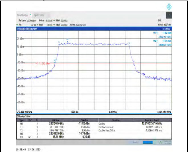
1-N77-3700-3980-PC1.5-30-15-M-6-CP-QPSK-Outer_Full-38@0-Ant1-13.61-15.240-≤15-PASS
