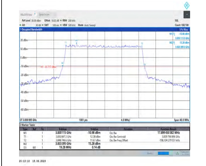
1-N77-3700-3980-PC1.5-30-20-M-4-DFT-64QAM-Outer_Full-50@0-Ant1-17.899-19.280-≤20-PASS
