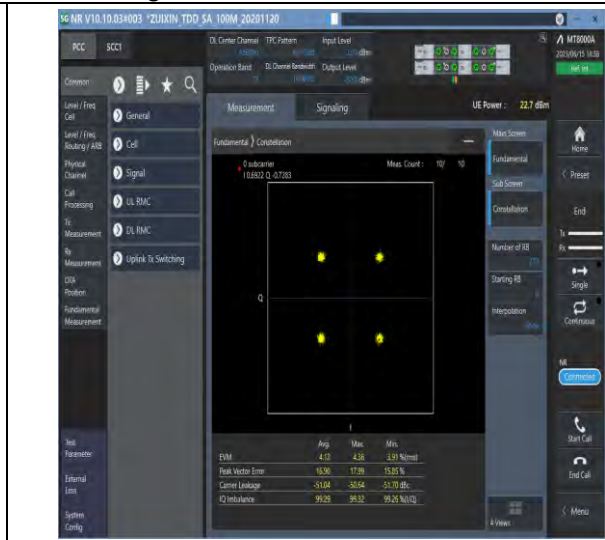
1-N77-3700-3980-PC1.5-30-100-M-6-CP-QPSK-Outer_Full-273@0-Ant1-see graph-PASS
