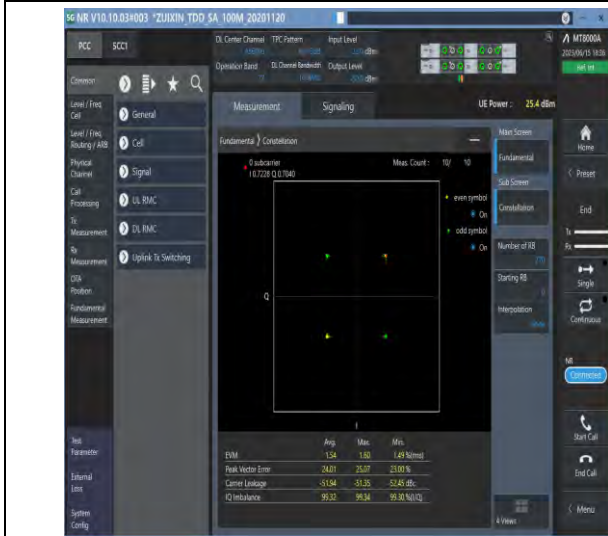
1-N77-3700-3980-PC1.5-30-100-M-1-DFT-PI2BPSK-Outer_Full-270@0-Ant1-see graph-PASS
