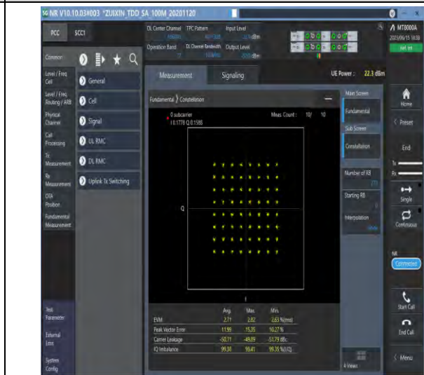
1-N77-3700-3980-PC1.5-30-100-M-8-CP-64QAM-Outer_Full-273@0-Ant1-see graph-PASS
