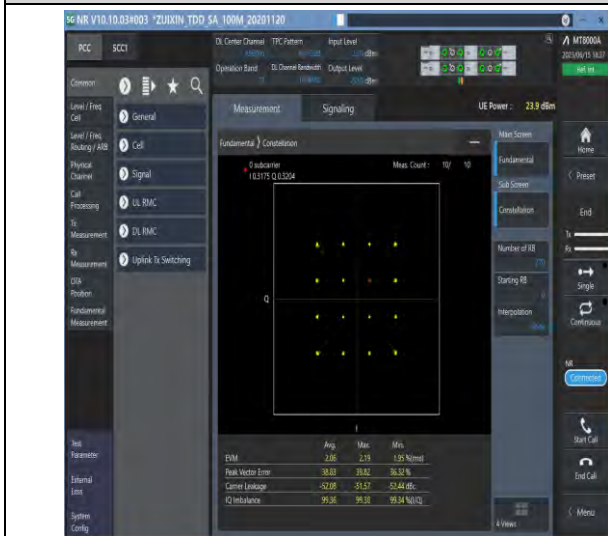
1-N77-3700-3980-PC1.5-30-100-M-3-DFT-16QAM-Outer_Full-270@0-Ant1-see graph-PASS
