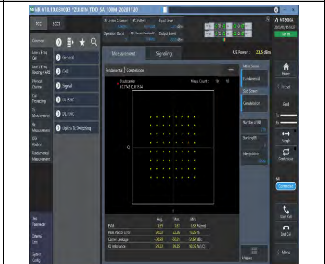
1-N77-3700-3980-PC1.5-30-100-M-4-DFT-64QAM-Outer_Full-270@0-Ant1-see graph-PASS
