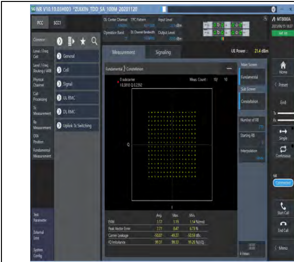
1-N77-3700-3980-PC1.5-30-100-M-5-DFT-256QAM-Outer_Full-270@0-Ant1-see graph-PASS
