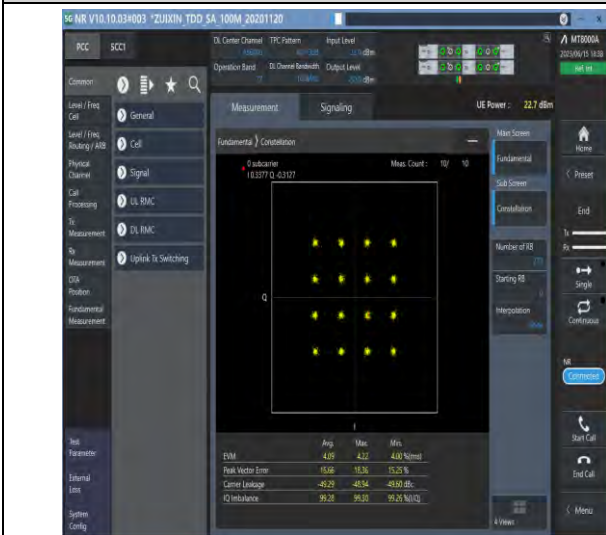
1-N77-3700-3980-PC1.5-30-100-M-7-CP-16QAM-Outer_Full-273@0-Ant1-see graph-PASS
