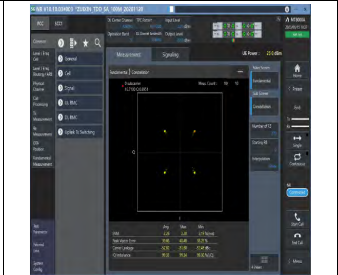
1-N77-3700-3980-PC1.5-30-100-M-2-DFT-QPSK-Outer_Full-270@0-Ant1-see graph-PASS
