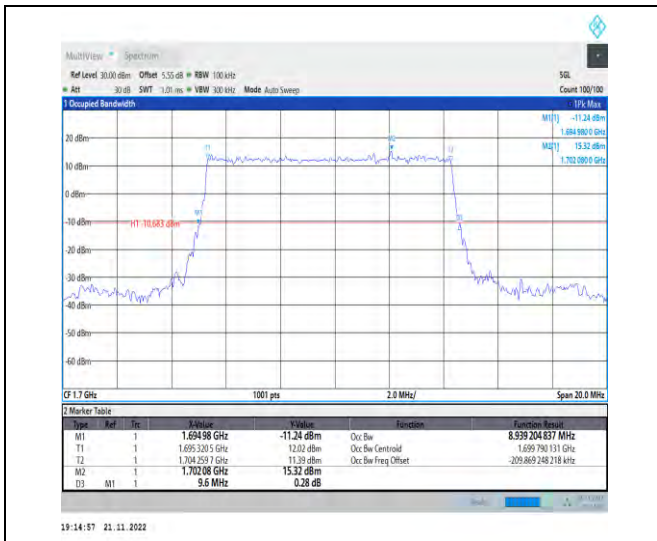
1-N70-PC3-15-10-L-2-DFT-PI2BPSK-Outer_Full-50 @0-Ant1-8.939-9.600-≤10-PASS
