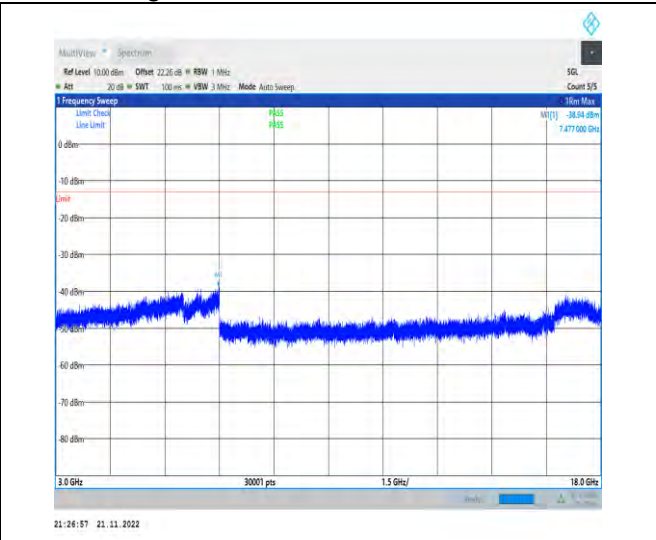
1-N70-PC3-15-15-M-1-DFT-PI2BPSK-Inner_1RB_Le ft-1@1-3000-18000-Ant1-7477.00--38.94--13-PASS
