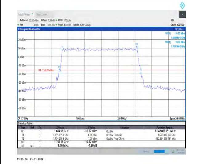
1-N70-PC3-15-10-L-5-DFT-256QAM-Outer_Full-50 @0-Ant1-8.943-9.760-≤10-PASS
