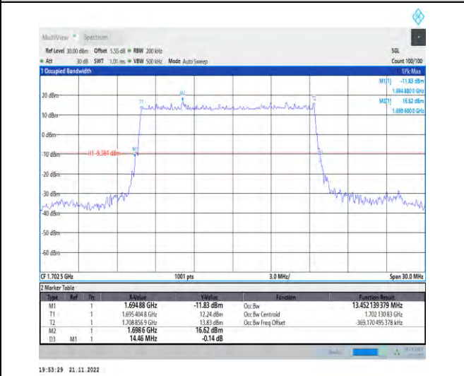
1-N70-PC3-15-15-L-2-DFT-PI2BPSK-Outer_Full-75 @0-Ant1-13.452-14.460-≤15-PASS
