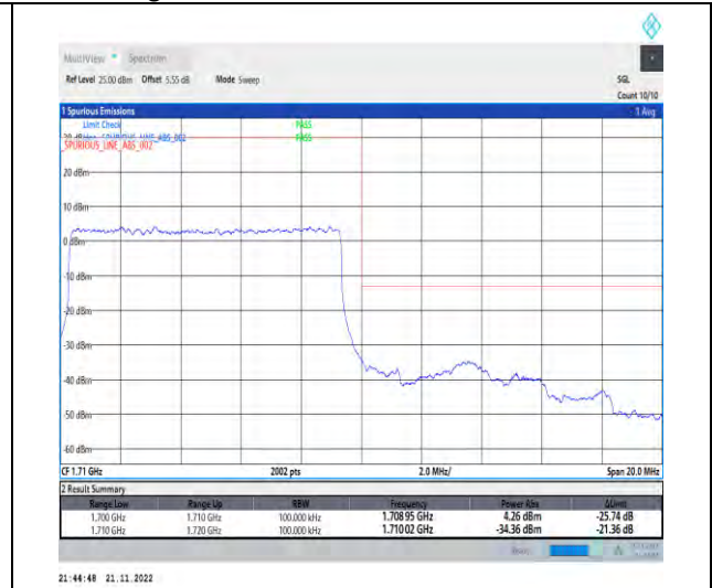
1-N70-PC3-15-10-H-3-DFT-PI2BPSK-Outer_Full-50@0-Ant1-1-seegraph-PASS-see graph
