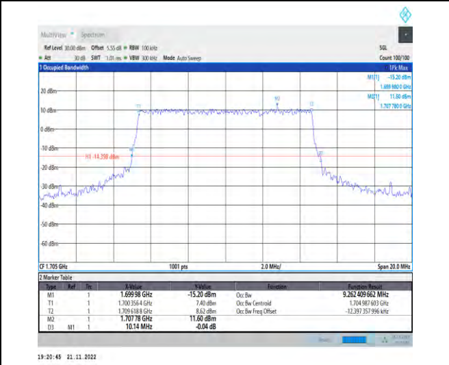
1-N70-PC3-15-10-H-7-CP-16QAM-Outer_Full-52@0 -Ant1-9.262-10.140-≤10-PASS
