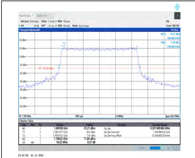
1-N70-PC3-15-10-H-8-CP-64QAM-Outer_Full-52@0 -Ant1-9.297-10.020-≤10-PASS
