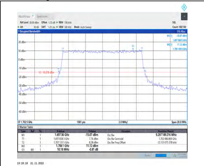
1-N70-PC3-15-10-M-6-CP-QPSK-Outer_Full-52@0-Ant1-9.297-10.180-≤10-PASS
