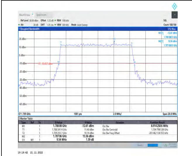
1-N70-PC3-15-10-H-2-DFT-PI2BPSK-Outer_Full-50@ 0-Ant1-8.914-9.540-≤10-PASS
