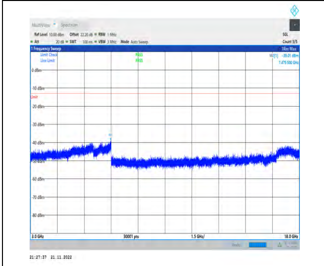
1-N70-PC3-15-15-H-1-DFT-PI2BPSK-Inner_1RB_Le ft-1@1-3000-18000-Ant1-7475.50--39.01--13-PASS
