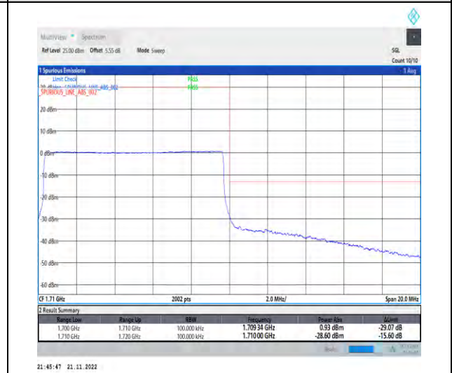
1-N70-PC3-15-10-H-6-CP-QPSK-Outer_Full-52@0-Ant1-1-seegraph-PASS-see graph
