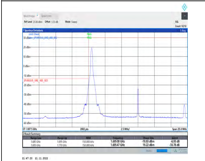
1-N70-PC3-15-15-L-4-CP-QPSK-Edge_1RB_Left-1@0-Ant1-1-seegraph-PASS-see graph
