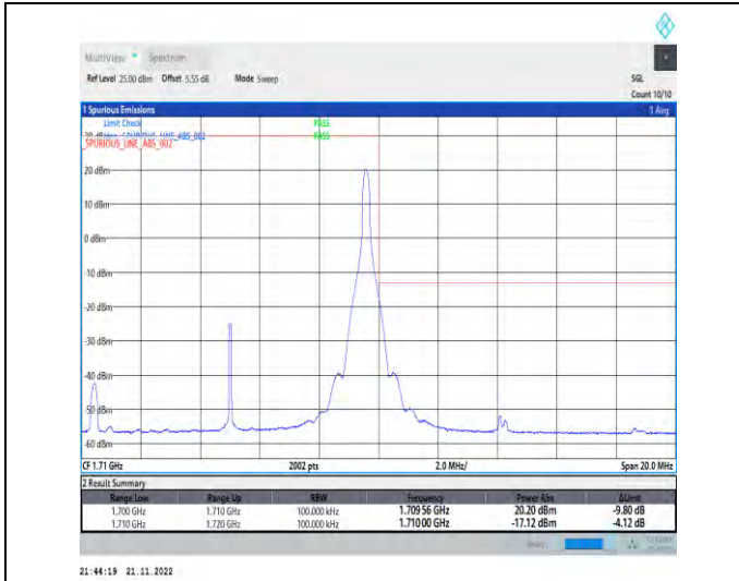
1-N70-PC3-15-10-H-2-DFT-PI2BPSK-Edge_1RB_Right-t@51-Ant1-1-seegraph-PASS-see graph
