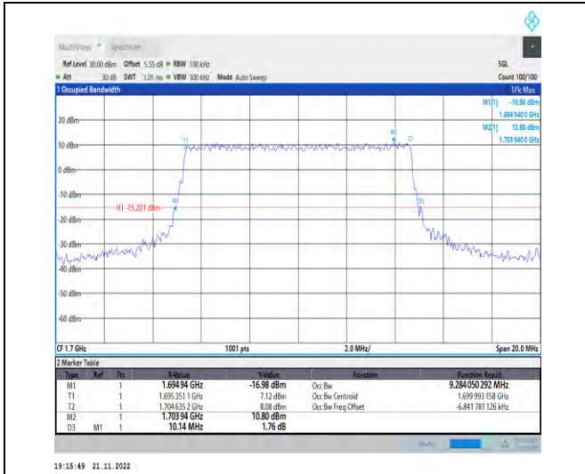
1-N70-PC3-15-10-L-6-CP-QPSK-Outer_Full-52@0-A Ant1-9.284-10.140-≤10-PASS
