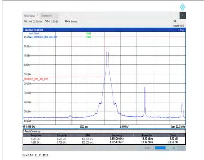
1-N70-PC3-15-10-L-4-CP-QPSK-Edge_1RB_Left-1@0-Ant1-1-seegraph-PASS-see graph
