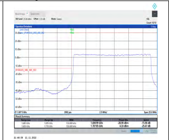
1-N70-PC3-15-15-L-3-DFT-PI2BPSK-Outer_Full-75@0-Ant1-1-seegraph-PASS-see graph
