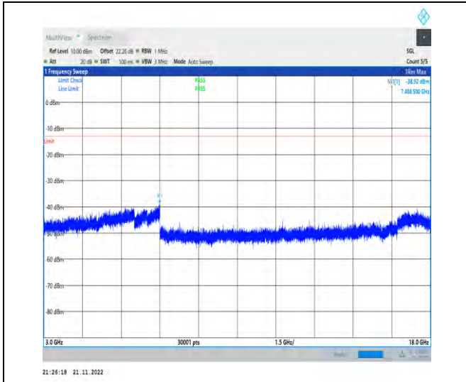
1-N70-PC3-15-15-L-1-DFT-PI2BPSK-Inner_1RB_Lef t-1@1-3000-18000-Ant1-7488.50--38.92--13-PASS
