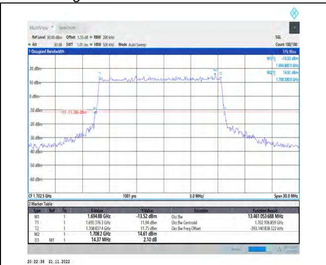
1-N70-PC3-15-15-M-3-DFT-16QAM-Outer_Full-75 @0-Ant1-13.461-14.370-≤15-PASS
