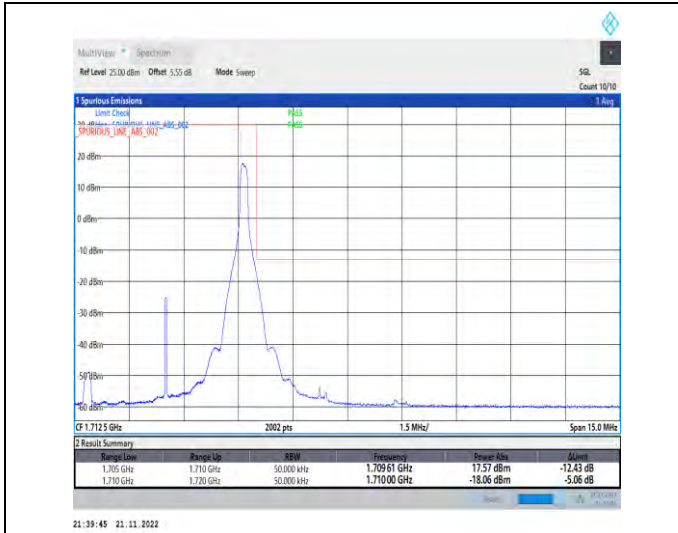
1-N70-PC3-15-5-H-2-DFT-PI2BPSK-Edge_1RB_Right-1@24-Ant1-1-seegraph-PASS-see graph
