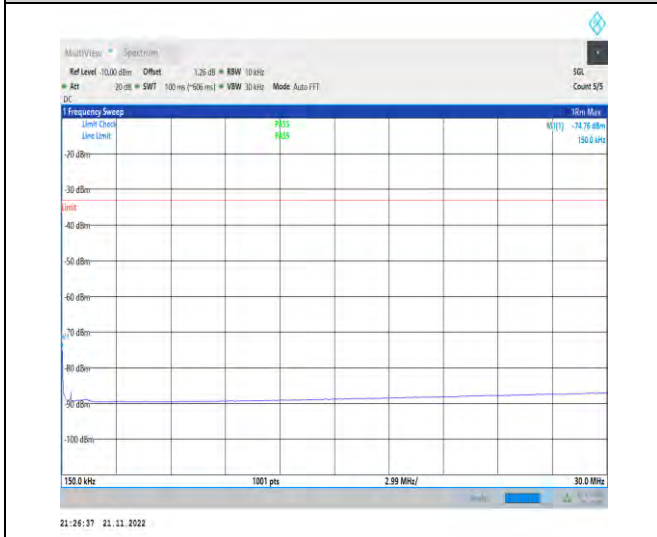
1-N70-PC3-15-15-M-1-DFT-PI2BPSK-Inner_1RB_Le ft-1@1-0.15-30-Ant1-0.15--74.76--33-PASS
