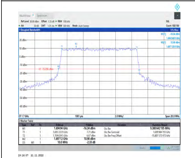
1-N70-PC3-15-10-L-8-CP-64QAM-Outer_Full-52@0- Ant1-9.301-10.000-≤10-PASS
