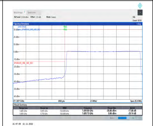
1-N70-PC3-15-15-L-6-CP-QPSK-Outer_Full-79@0-Ant1-1-seegraph-PASS-see graph
