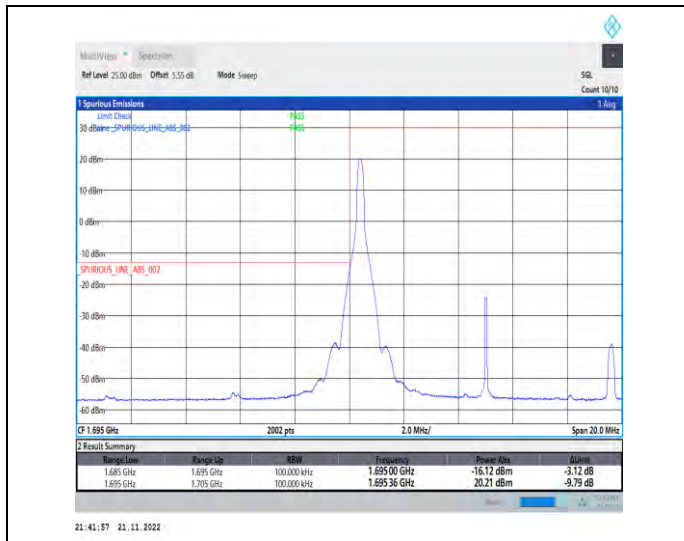
1-N70-PC3-15-10-L-1-DFT-PI2BPSK-Edge_1RB_Left-1@0-Ant1-1-seegraph-PASS-see graph
