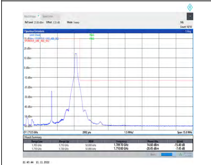
1-N70-PC3-15-5-H-5-CP-QPSK-Edge_1RB_Right-1@24-Ant1-1-seegraph-PASS-see graph
