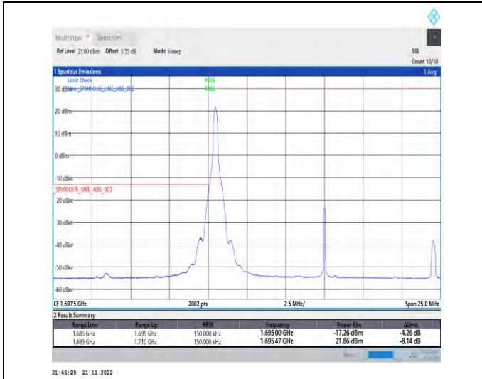
1-N70-PC3-15-15-L-1-DFT-PI2BPSK-Edge_1RB_Left-1@0-Ant1-1-seegraph-PASS-see graph
