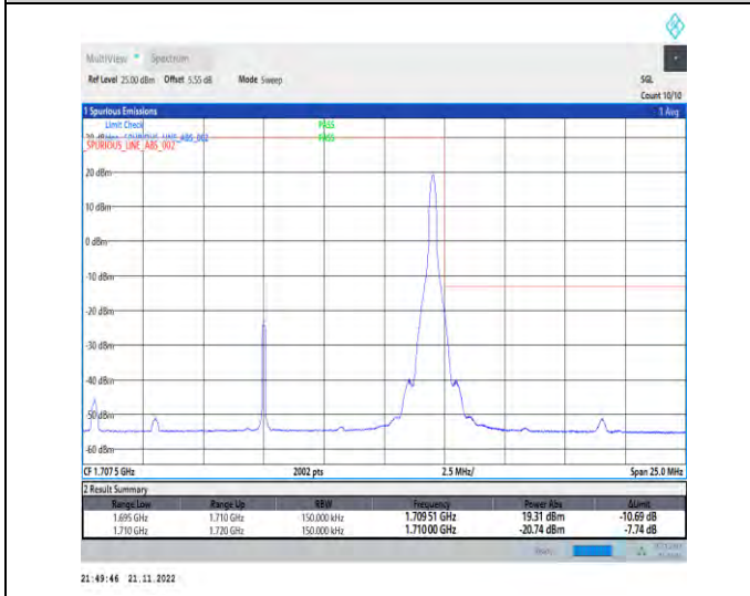
1-N70-PC3-15-15-H-5-CP-QPSK-Edge_1RB_Right-1@78-Ant1-1-seegraph-PASS-see graph
