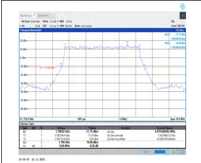
1-N70-PC3-15-5-M-2-DFT-PI2BPSK-Outer_Full-25@0-Ant1-4.479-5.040-≤5-PASS
