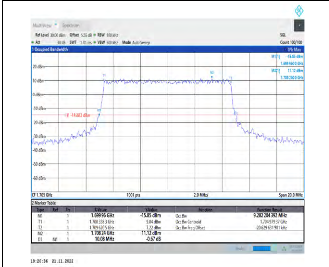
1-N70-PC3-15-10-H-6-CP-QPSK-Outer_Full-52@0- Ant1-9.282-10.080-≤10-PASS
