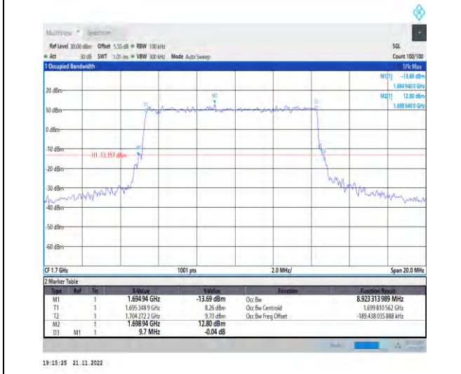
1-N70-PC3-15-10-L-4-DFT-64QAM-Outer_Full-50 @0-Ant1-8.923-9.700-≤10-PASS
