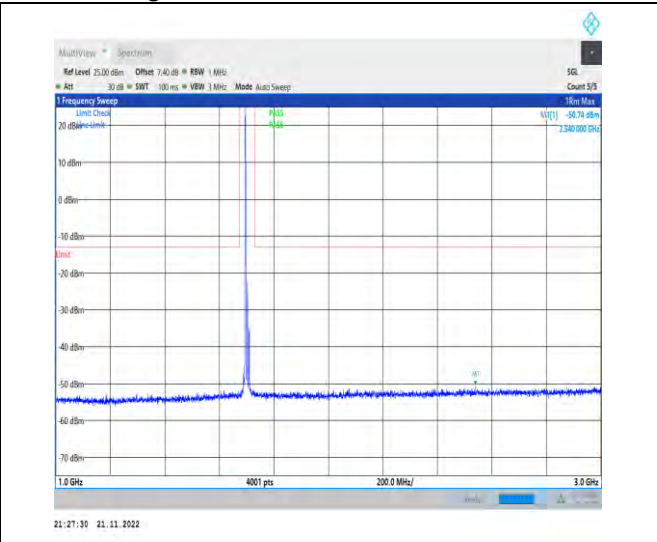
1-N70-PC3-15-15-H-1-DFT-PI2BPSK-Inner_1RB_Le ft-1@1-1000-3000-Ant1-2540.00--50.74--13-PASS
