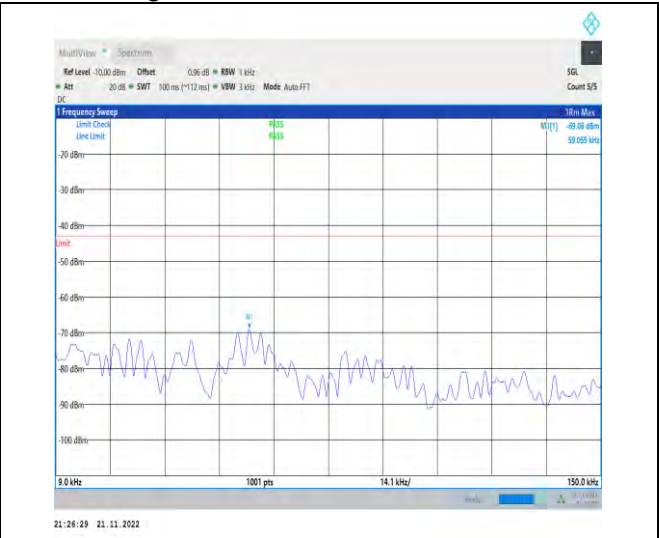
1-N70-PC3-15-15-M-1-DFT-PI2BPSK-Inner_1RB_Le ft-1@1-0.009-0.15-Ant1-0.06--69.06--43-PASS
