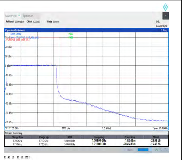
1-N70-PC3-15-5-H-6-CP-QPSK-Outer_Full-25@0-Ant1-1-seegraph-PASS-see graph
