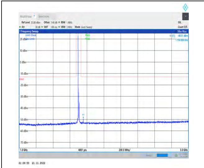
1-N70-PC3-15-15-M-1-DFT-PI2BPSK-Inner_1RB_Le ft-1@1-1000-3000-Ant1-1756.50--49.31--13-PASS
