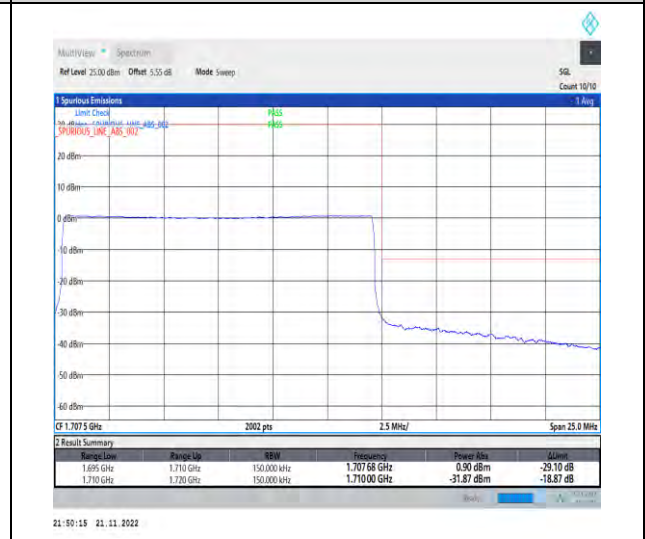
1-N70-PC3-15-15-H-6-CP-QPSK-Outer_Full-79@0-Ant1-1-seegraph-PASS-see graph
