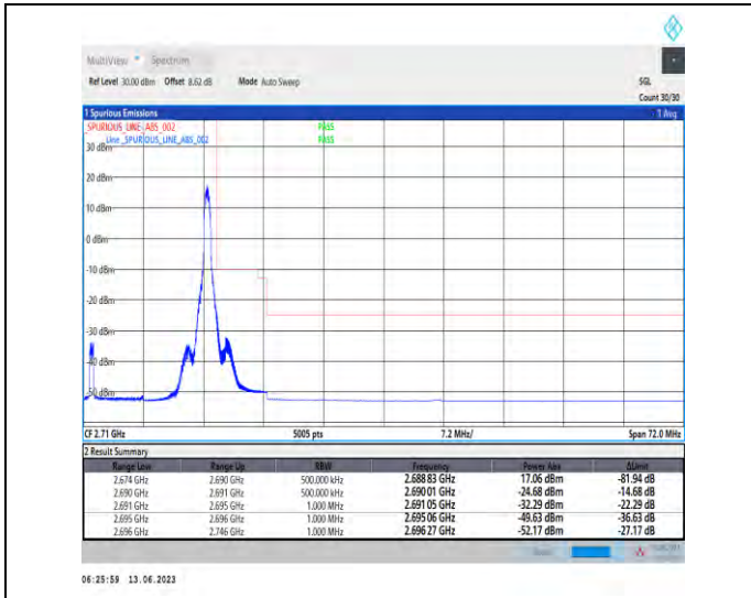
1-N41-PC1.5-30-30-H-2-DFT-PI2BPSK-Edge_1RB_Ri ght-1@77-Ant1-1--PASS-see graph
