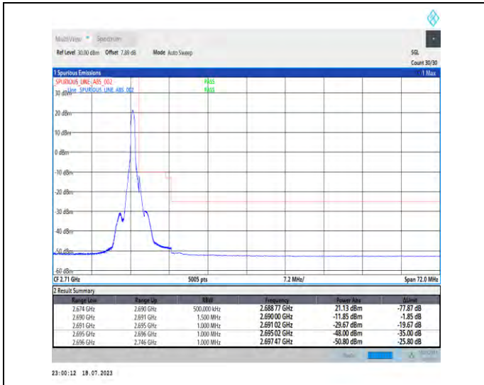
1-N41-PC1.5-30-70-H-2-DFT-PI2BPSK-Edge_1RB_Ri ght-1@188-Ant1-1--PASS-see graph
