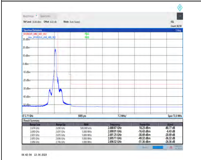
1-N41-PC1.5-30-40-H-5-CP-QPSK-Edge_1RB_Ri ght-1@105-Ant1-1--PASS-see graph
