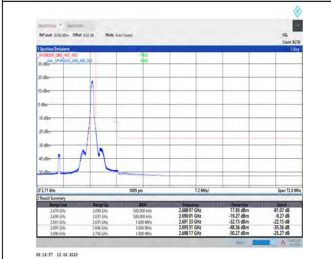
1-N41-PC1.5-30-20-H-5-CP-QPSK-Edge_1RB_Right-1 @50-Ant1-1--PASS-see graph
