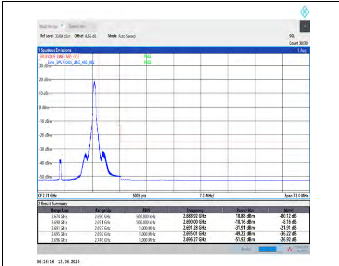
1-N41-PC1.5-30-20-H-2-DFT-PI2BPSK-Edge_1RB_Ri ght-1@50-Ant1-1--PASS-see graph
