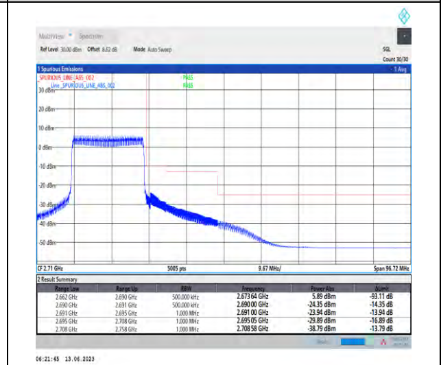
1-N41-PC1.5-30-20-H-6-CP-QPSK-Outer_Full-51 @0-Ant1-1--PASS-see graph
