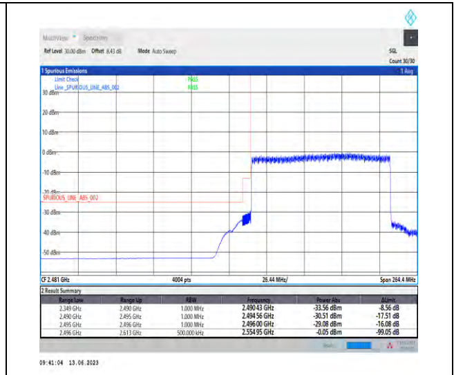
1-N41-PC1.5-30-100-L-3-DFT-PI2BPSK-Outer_Full-270@0-Ant1-1--PASS-see graph
