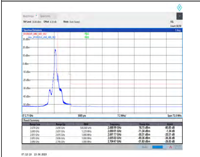
1-N41-PC1.5-30-60-H-5-CP-QPSK-Edge_1RB_Right-1 @161-Ant1-1--PASS-see graph
