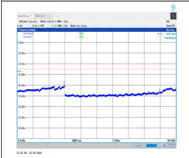
1-N41-PC1.5-30-100-M-1-N/A-DFT-QPSK-Edge_1R B_Left-1@0-3000-18000-Ant1-7475.50--40.01--25-P ASS
