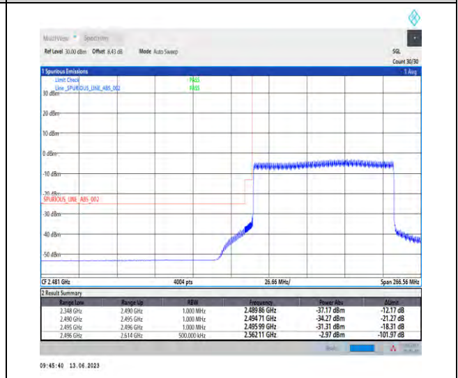
1-N41-PC1.5-30-100-L-6-CP-QPSK-Outer_Full-273@0-Ant1-1--PASS-see graph
