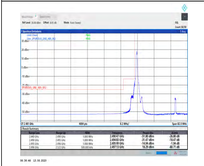
1-N41-PC1.5-30-40-L-4-CP-QPSK-Edge_1RB_Left-1 @0-Ant1-1--PASS-see graph
