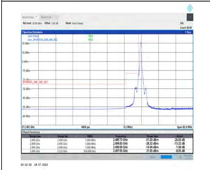
1-N41-PC1.5-30-100-L-4-CP-QPSK-Edge_1RB_Left-1@0-Ant1-1--PASS-see graph
