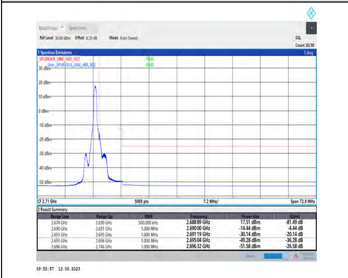
1-N41-PC1.5-30-100-H-5-CP-QPSK-Edge_1RB_Right- 1@272-Ant1-1--PASS-see graph
