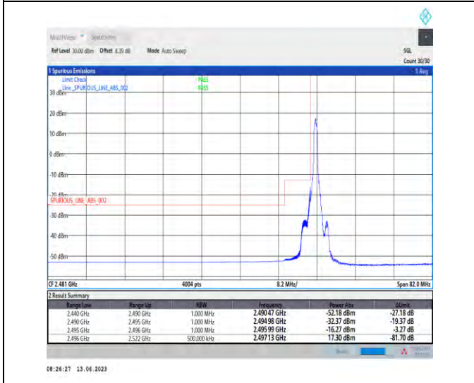
1-N41-PC1.5-30-80-L-4-CP-QPSK-Edge_1RB_Left-1 @0-Ant1-1--PASS-see graph
