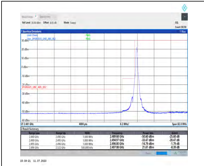
1-N41-PC1.5-30-100-L-1-DFT-PI2BPSK-Edge_1RB_Left-1@0-Ant1-1--PASS-see graph
