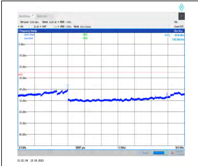
1-N41-PC1.5-30-100-L-1-N/A-DFT-QPSK-Edge_1R B_Left-1@0-3000-18000-Ant1-7479.00--39.98--25-P ASS
