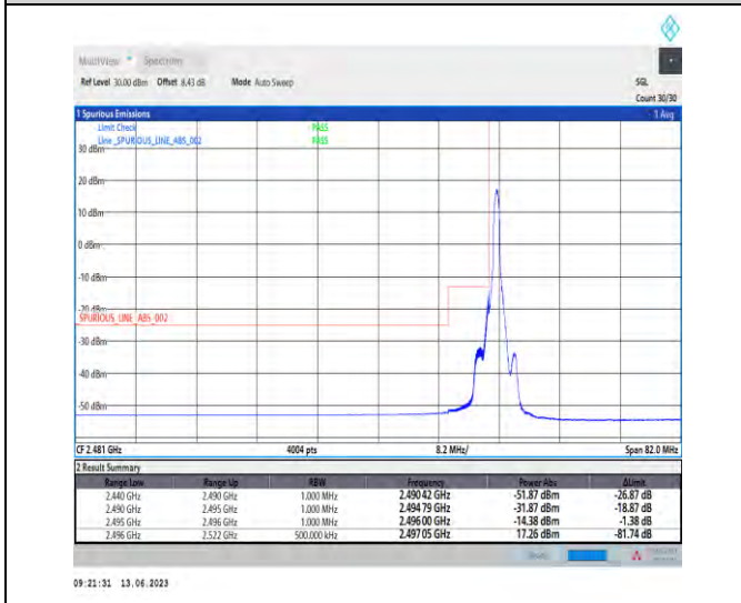
1-N41-PC1.5-30-90-L-4-CP-QPSK-Edge_1RB_Left-1 @0-Ant1-1--PASS-see graph
