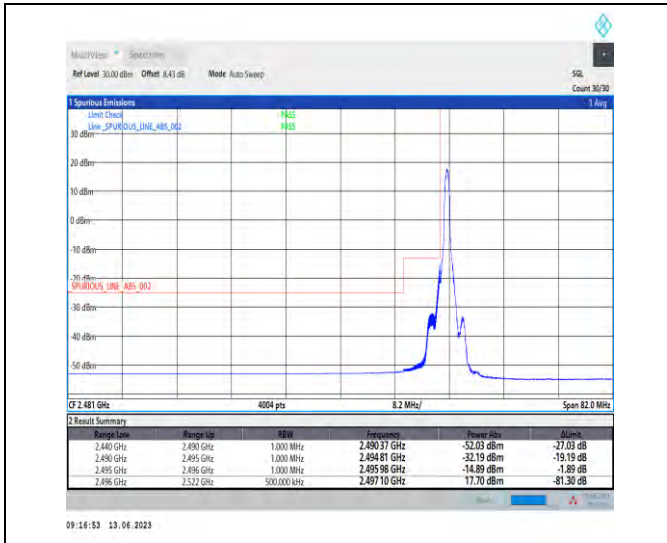
1-N41-PC1.5-30-90-L-1-DFT-PI2BPSK-Edge_1RB_L eft-1@0-Ant1-1--PASS-see graph
