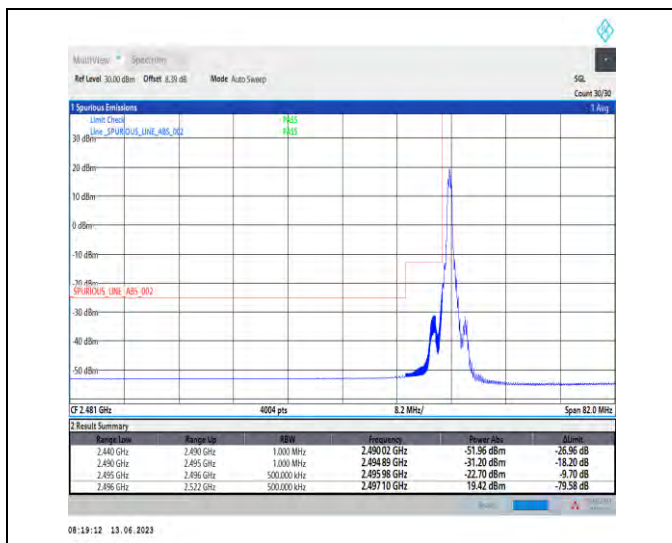
1-N41-PC1.5-30-70-L-1-DFT-PI2BPSK-Edge_1RB_L eft-1@0-Ant1-1--PASS-see graph
