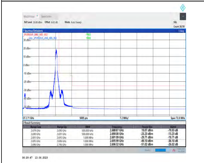
1-N41-PC1.5-30-30-H-5-CP-QPSK-Edge_1RB_R ight-1@77-Ant1-1--PASS-see graph
