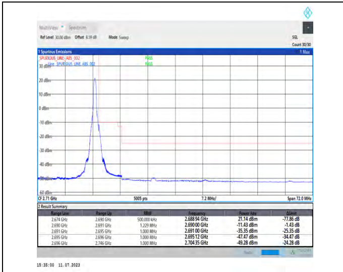
1-N41-PC1.5-30-60-H-2-DFT-PI2BPSK-Edge_1RB_Ri ght-1@161-Ant1-1--PASS-see graph
