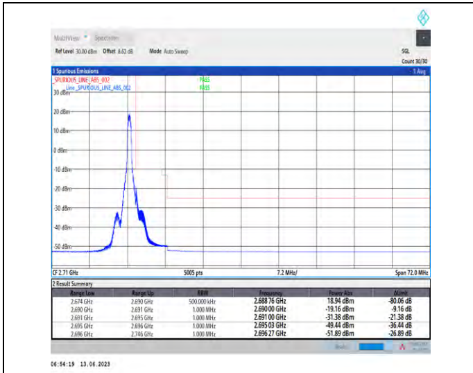
1-N41-PC1.5-30-50-H-2-DFT-PI2BPSK-Edge_1RB_Ri ght-1@132-Ant1-1--PASS-see graph
