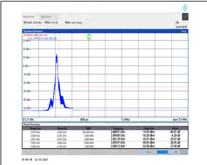
1-N41-PC1.5-30-100-H-2-DFT-PI2BPSK-Edge_1RB_R igt-1@272-Ant1-1--PASS-see graph
