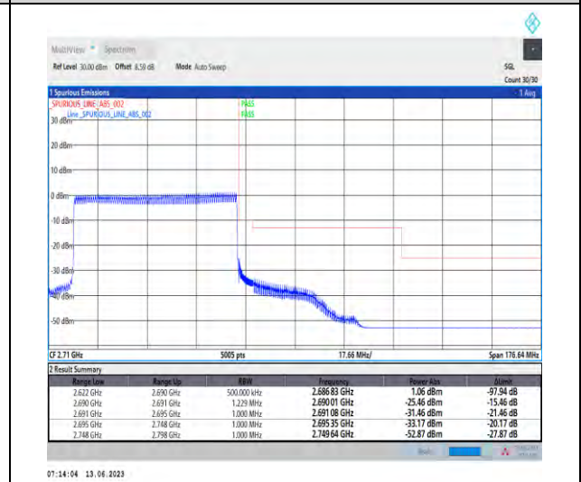
1-N41-PC1.5-30-60-H-6-CP-QPSK-Outer_Full-162 @0-Ant1-1--PASS-see graph
