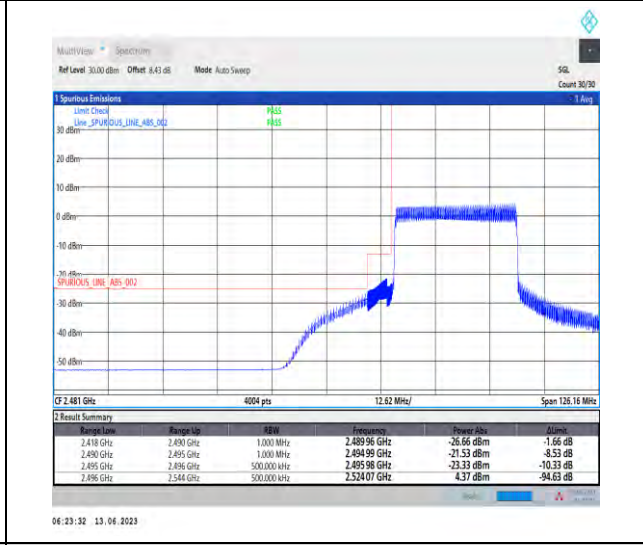
1-N41-PC1.5-30-30-L-6-CP-QPSK-Outer_Full-78@0-Ant1-1--PASS-see graph
