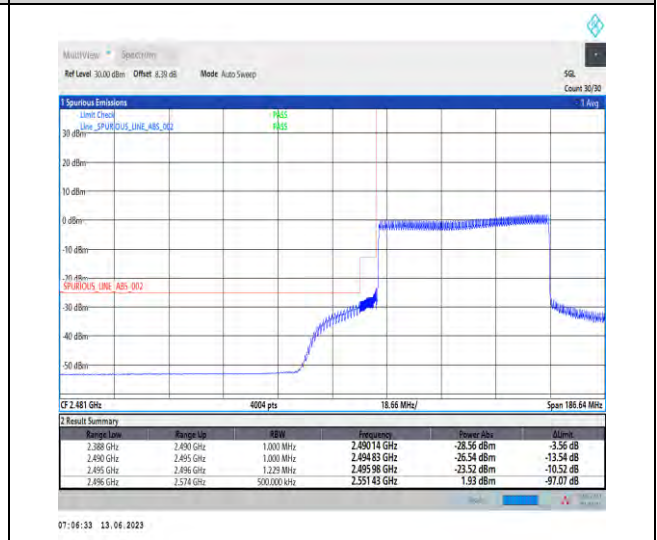
1-N41-PC1.5-30-60-L-6-CP-QPSK-Outer_Full-162 @0-Ant1-1--PASS-see graph
