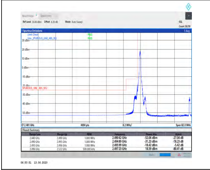
1-N41-PC1.5-30-50-L-4-CP-QPSK-Edge_1RB_Left-1 @0-Ant1-1--PASS-see graph
