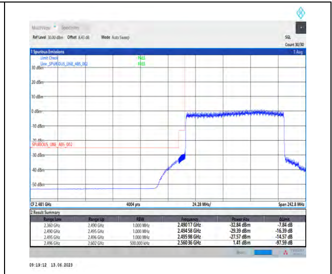
1-N41-PC1.5-30-90-L-3-DFT-PI2BPSK-Outer_Full-2 40@0-Ant1-1--PASS-see graph
