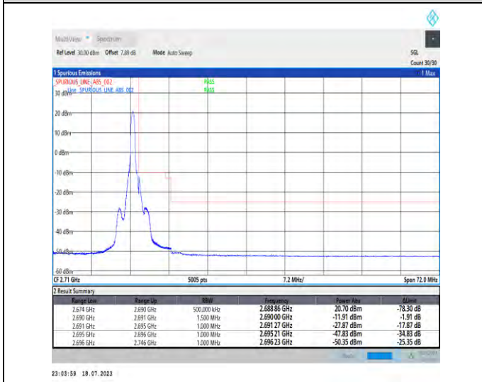
1-N41-PC1.5-30-80-H-5-CP-QPSK-Edge_1RB_Ri ght-1@216-Ant1-1--PASS-see graph
