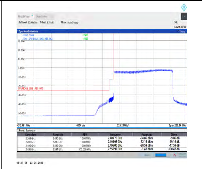
1-N41-PC1.5-30-80-L-6-CP-QPSK-Outer_Full-217 @0-Ant1-1--PASS-see graph
