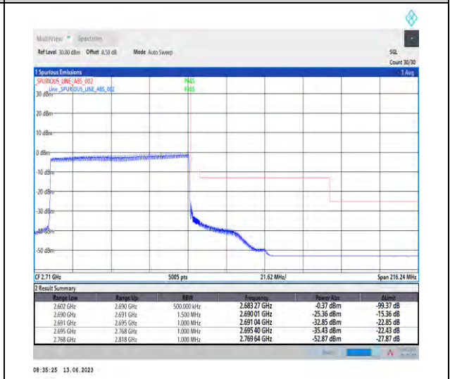
1-N41-PC1.5-30-80-H-6-CP-QPSK-Outer_Full-217 @0-Ant1-1--PASS-see graph
