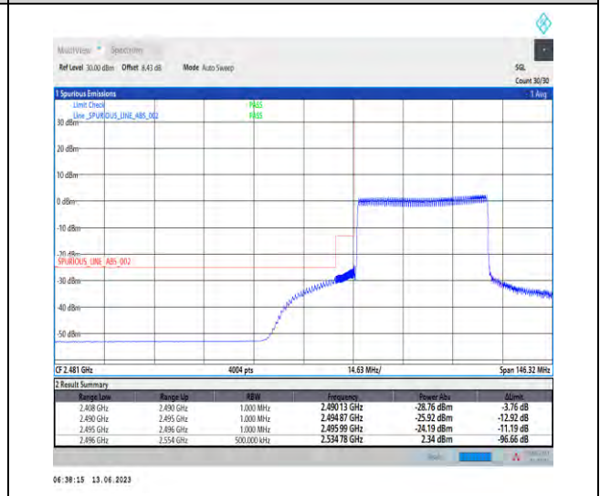
1-N41-PC1.5-30-40-L-6-CP-QPSK-Outer_Full-106 @0-Ant1-1--PASS-see graph
