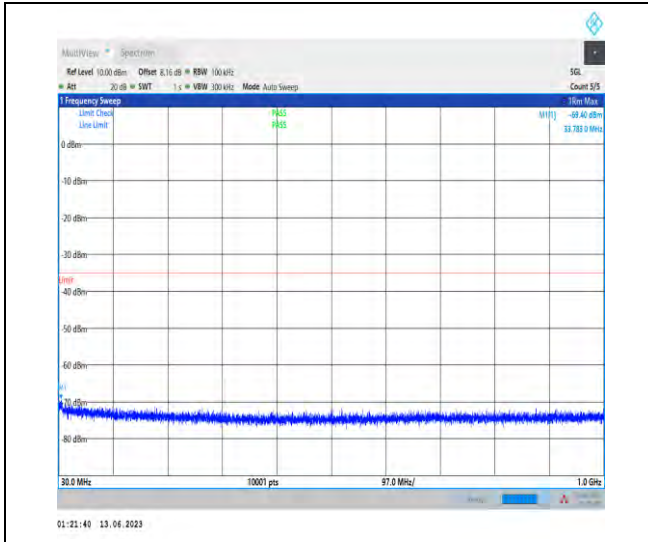
1-N41-PC1.5-30-100-M-1-N/A-DFT-QPSK-Edge_1R B_Left-1@0-30-1000-Ant1-35.34--69.40--35-PASS
