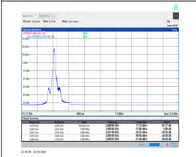
1-N41-PC1.5-30-90-H-5-CP-QPSK-Edge_1RB_Ri ght-1 @244-Ant1-1--PASS-see graph
