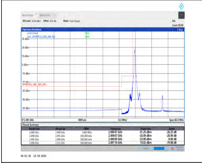
1-N41-PC1.5-30-30-L-4-CP-QPSK-Edge_1RB_Left-1 @0-Ant1-1--PASS-see graph
