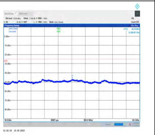
1-N41-PC1.5-30-100-M-1-N/A-DFT-QPSK-Edge_1R B_Left-1@0-18000-26500-Ant1-20443.75--46.18--25- PASS
