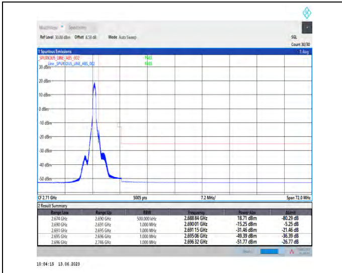
1-N41-PC1.5-30-90-H-2-DFT-PI2BPSK-Edge_1RB_Ri ght-1@244-Ant1-1--PASS-see graph
