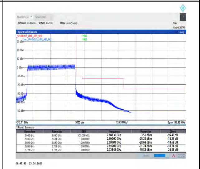
1-N41-PC1.5-30-40-H-6-CP-QPSK-Outer_Full-106 @0-Ant1-1--PASS-see graph
