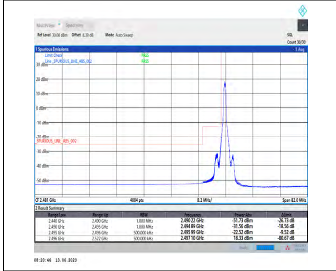
1-N41-PC1.5-30-70-L-4-CP-QPSK-Edge_1RB_Left-1 @0-Ant1-1--PASS-see graph
