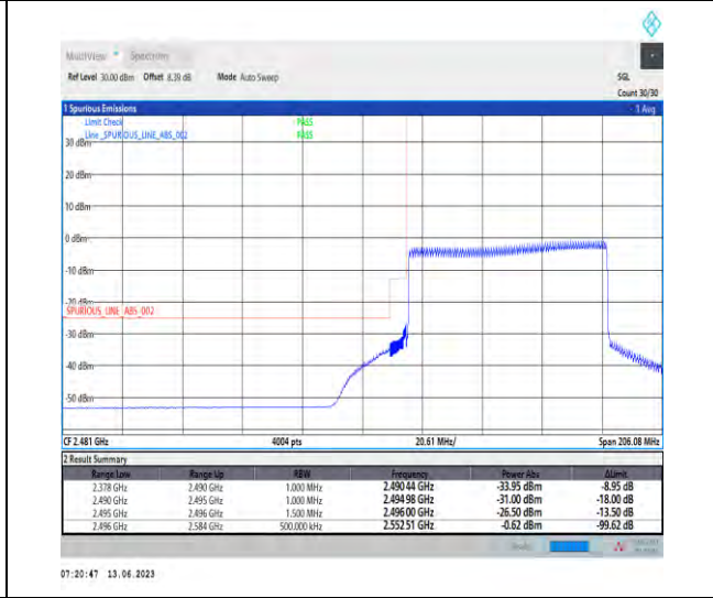
1-N41-PC1.5-30-70-L-6-CP-QPSK-Outer_Full-189 @0-Ant1-1--PASS-see graph
