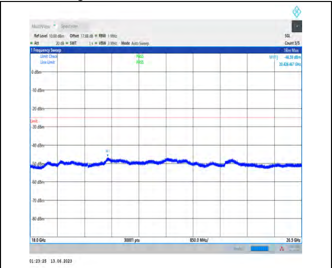
1-N41-PC1.5-30-100-H-1-N/A-DFT-QPSK-Edge_1RB _Left-1@0-18000-26500-Ant1-20425.90--46.59--25-P ASS
