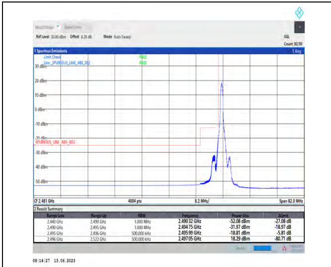
1-N41-PC1.5-30-60-L-1-DFT-PI2BPSK-Edge_1RB_L eft-1@0-Ant1-1--PASS-see graph
