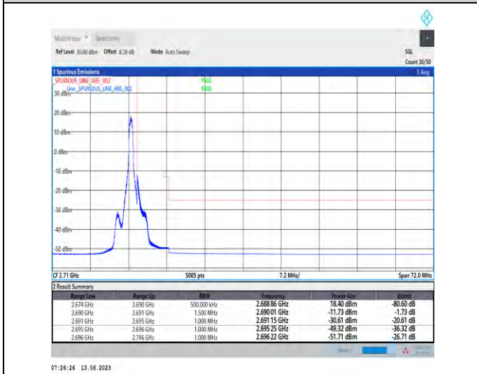
1-N41-PC1.5-30-70-H-5-CP-QPSK-Edge_1RB_Ri ght-1@188-Ant1-1--PASS-see graph
