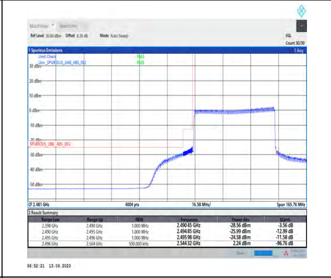
1-N41-PC1.5-30-50-L-6-CP-QPSK-Outer_Full-133 @0-Ant1-1--PASS-see graph
