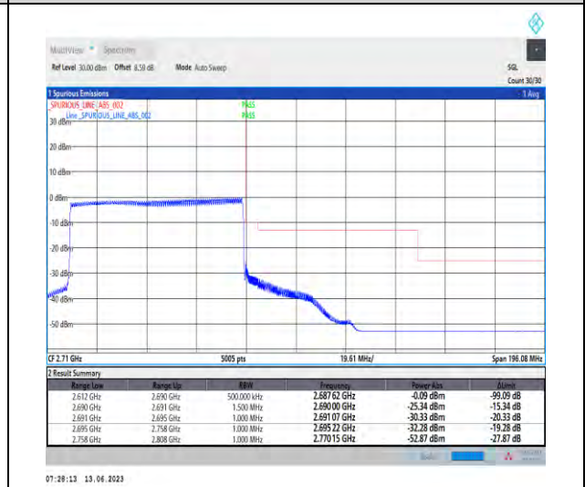
1-N41-PC1.5-30-70-H-6-CP-QPSK-Outer_Full-189 @0-Ant1-1--PASS-see graph
