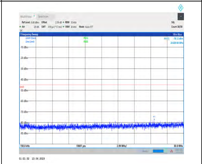
1-N41-PC1.5-30-100-M-1-N/A-DFT-QPSK-Edge_1R B_Left-1@0.15-30-Ant1-0.46--78.12--45-PASS
