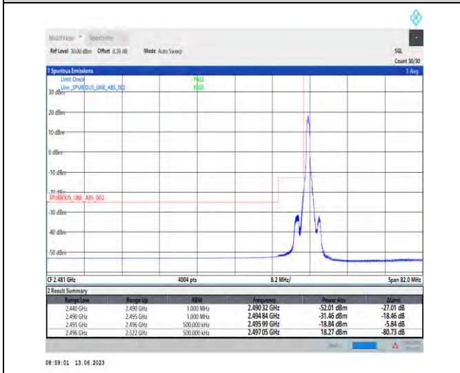
1-N41-PC1.5-30-60-L-4-CP-QPSK-Edge_1RB_Left-1 @0-Ant1-1--PASS-see graph
