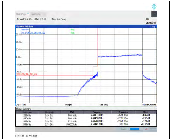
1-N41-PC1.5-30-60-L-3-DFT-PI2BPSK-Outer_Full-1 62@0-Ant1-1--PASS-see graph
