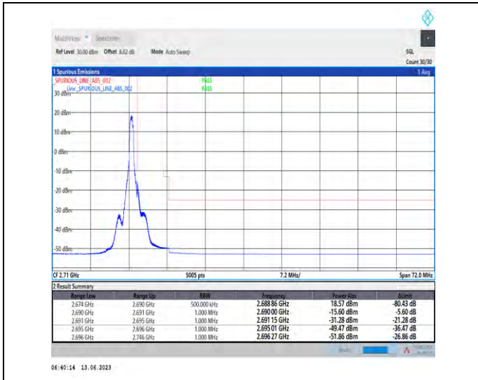
1-N41-PC1.5-30-40-H-2-DFT-PI2BPSK-Edge_1RB_Ri ght-1@105-Ant1-1--PASS-see graph
