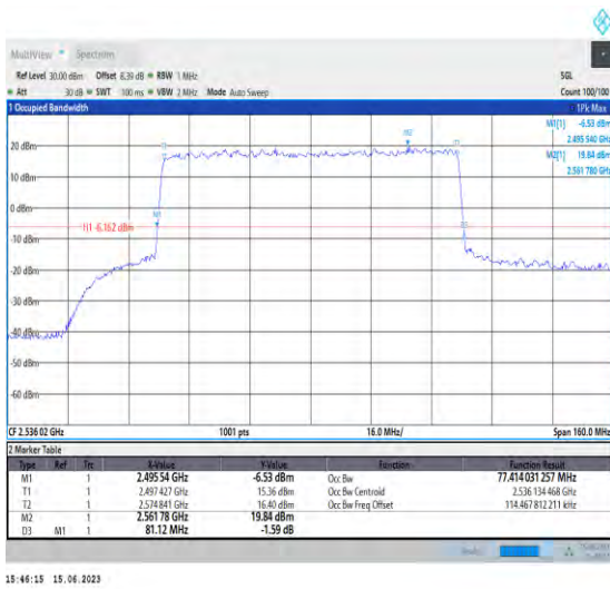
1-N41-PC1.5-30-80-L-7-CP-16QAM-Outer_Full-217 @0-Ant1-77.414-81.120-≤80-PASS
