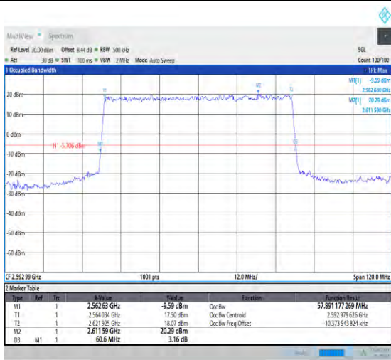
1-N41-PC1.5-30-60-L-9-CP-256QAM-Outer_Full-162 @0-Ant1-57.727-60.360-≤60-PASS
