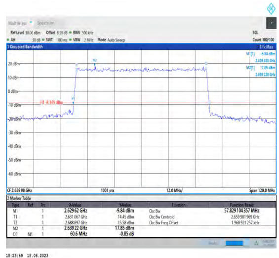
1-N41-PC1.5-30-60-H-6-CP-QPSK-Outer_Full-162@ 0-Ant1-57.829-60.600-≤60-PASS
