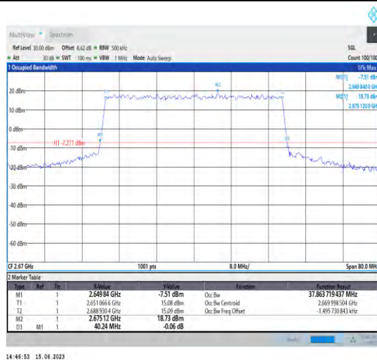
1-N41-PC1.5-30-40-H-8-CP-64QAM-Outer_Full-106@0-Ant1-37.864-40.240-≤40-PASS
