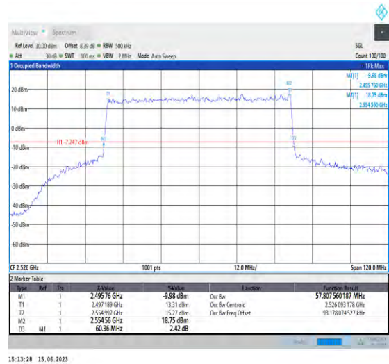
1-N41-PC1.5-30-60-L-8-CP-64QAM-Outer_Full-162 @0-Ant1-57.808-60.360-≤60-PASS
