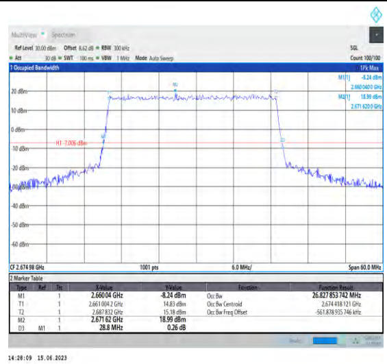
1-N41-PC1.5-30-30-H-1-DFT-QPSK-Outer_Full-75 @0-Ant1-26.828-28.800-≤30-PASS
