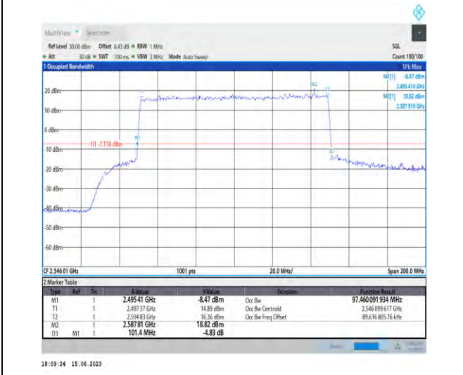
1-N41-PC1.5-30-100-L-7-CP-16QAM-Outer_Full-273@0-Ant1-97.46-101.400-≤100-PASS
