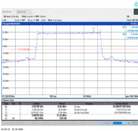
1-N41-PC1.5-30-50-M-1-DFT-QPSK-Outer_Full-128 @0-Ant1-45.698-48.200-≤50-PASS
