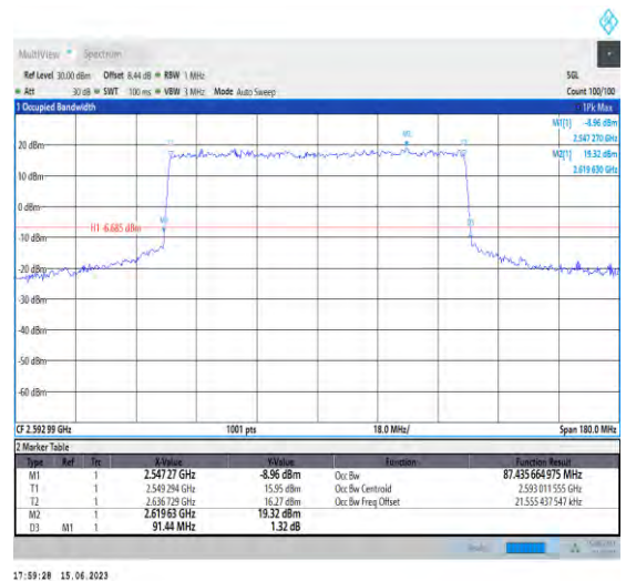
1-N41-PC1.5-30-90-M-6-CP-QPSK-Outer_Full-245@0-Ant1-87.436-91.440-≤90-PASS
