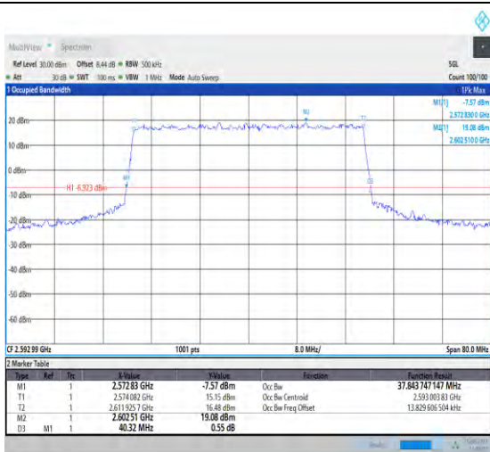
1-N41-PC1.5-30-40-M-6-CP-QPSK-Outer_Full-106 @0-Ant1-37.844-40.320-≤40-PASS
