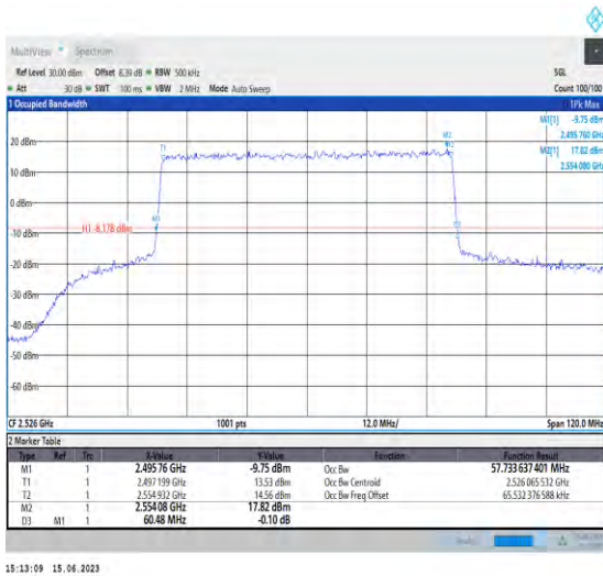
1-N41-PC1.5-30-60-L-7-CP-16QAM-Outer_Full-162 @0-Ant1-57.734-60.480-≤60-PASS
