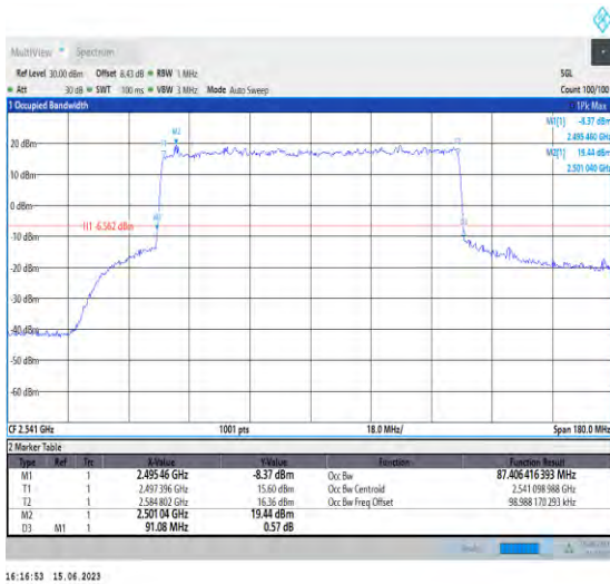
1-N41-PC1.5-30-90-L-6-CP-QPSK-Outer_Full-245 @0-Ant1-87.406-91.080-≤90-PASS
