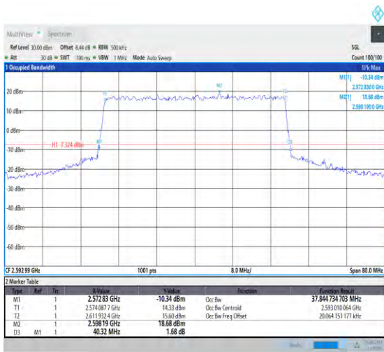
1-N41-PC1.5-30-40-M-6-CP-QPSK-Outer_Full-106 @0-Ant1-37.844-40.320-≤40-PASS
