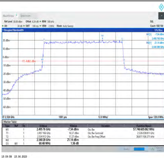
1-N41-PC1.5-30-60-L-1-DFT-QPSK-Outer_Full-162 @0-Ant1-57.747-60.480-≤60-PASS
