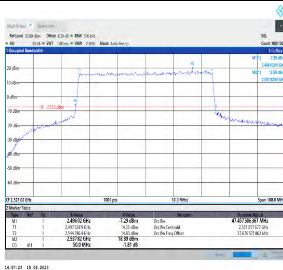
1-N41-PC1.5-30-50-L-7-CP-16QAM-Outer_Full-133 @0-Ant1-47.458-50.000-≤50-PASS
