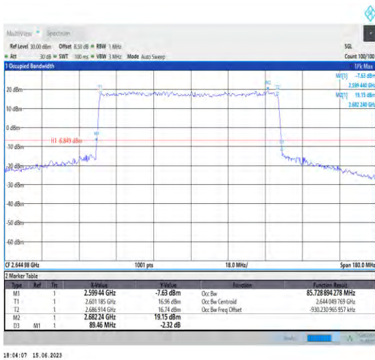
1-N41-PC1.5-30-90-H-4-DFT-64QAM-Outer_Full-24 0@0-Ant1-85.729-89.460-≤90-PASS
