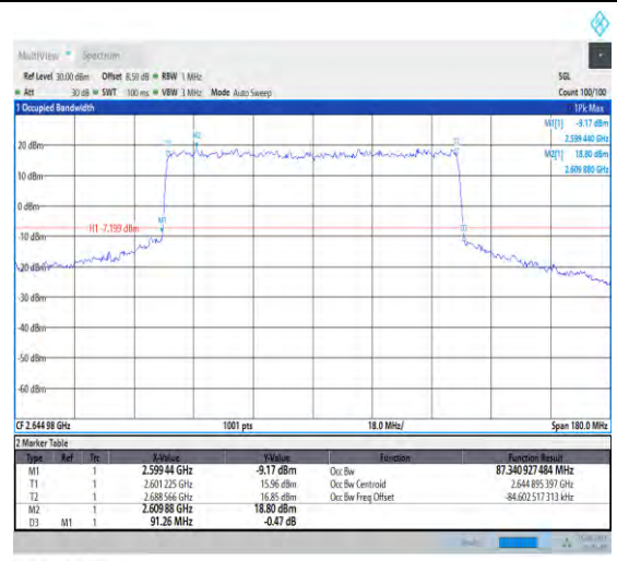
1-N41-PC1.5-30-90-H-7-CP-16QAM-Outer_Full-245 @0-Ant1-87.341-91.260-≤90-PASS
