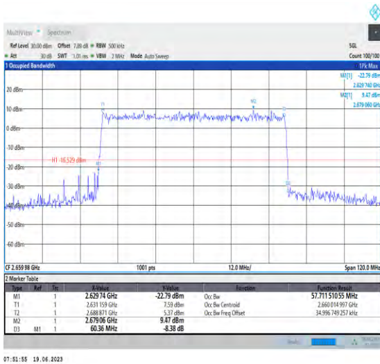
1-N41-PC1.5-30-60-H-9-CP-256QAM-Outer_Full-16 2@0-Ant1-57.712-60.360-≤60-PASS
