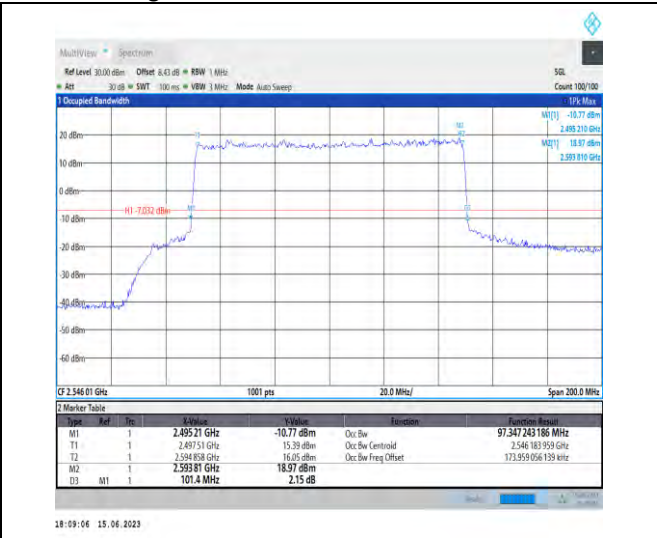
1-N41-PC1.5-30-100-L-6-CP-QPSK-Outer_Full-273@0-Ant1-97.347-101.400-≤100-PASS
