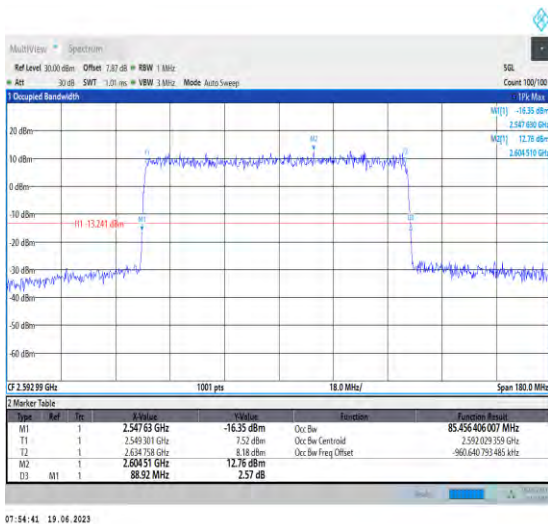
1-N41-PC1.5-30-90-M-5-DFT-256QAM-Outer_Full-240@0-Ant1-85.456-88.920-≤90-PASS
