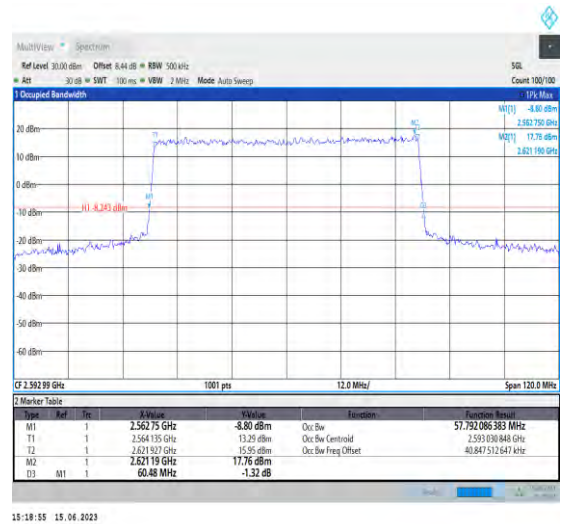
1-N41-PC1.5-30-60-M-7-CP-16QAM-Outer_Full-162 @0-Ant1-57.792-60.480-≤60-PASS
