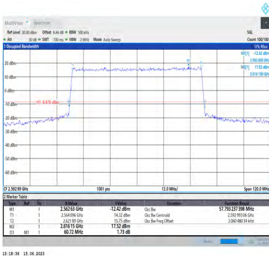
1-N41-PC1.5-30-60-M-6-CP-QPSK-Outer_Full-162 @0-Ant1-57.793-60.720-≤60-PASS
