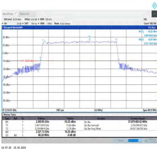
1-N41-PC1.5-30-40-L-9-CP-256QAM-Outer_Full-106 @0-Ant1-37.879-40.240-≤40-PASS
