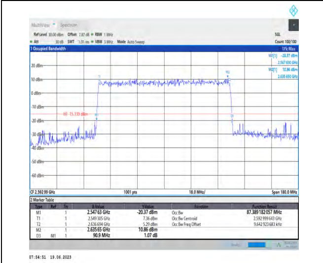
1-N41-PC1.5-30-90-M-9-CP-256QAM-Outer_Full-245 @0-Ant1-87.389-90.900-<math>\leq</math>90-PASS
