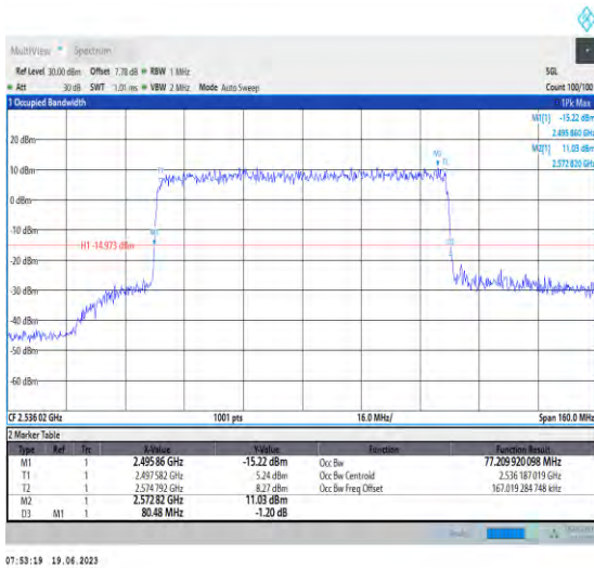
1-N41-PC1.5-30-80-L-9-CP-256QAM-Outer_Full-217 @0-Ant1-77.21-80.480-≤80-PASS
