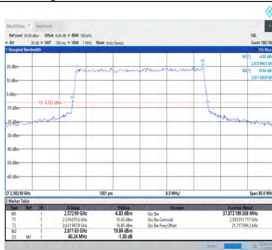
1-N41-PC1.5-30-40-M-7-CP-16QAM-Outer_Full-106 @0-Ant1-37.872-40.240-≤40-PASS
