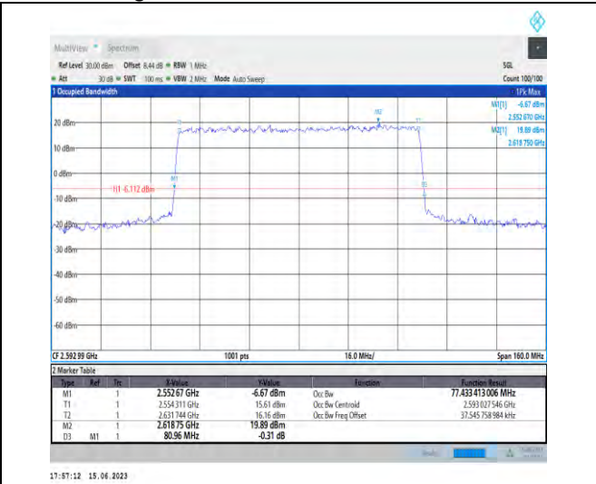
1-N41-PC1.5-30-80-M-7-CP-16QAM-Outer_Full-217 @0-Ant1-77.433-80.960-≤80-PASS
