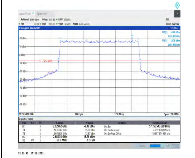
1-N41-PC1.5-30-60-H-1-DFT-QPSK-Outer_Full-162 @0-Ant1-57.756-60.600-≤60-PASS
