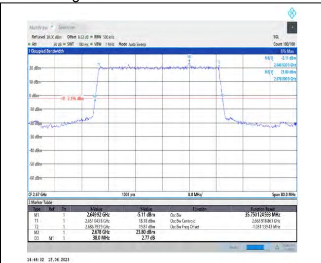
1-N41-PC1.5-30-40-H-2-DFT-PI2BPSK-Outer_Full-100 @0-Ant1-35.75-38.000-≤40-PASS
