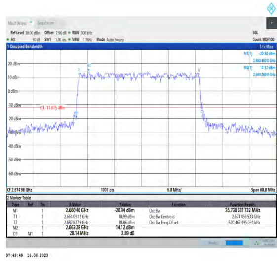
1-N41-PC1.5-30-30-H-3-DFT-16QAM-Outer_Full-75 @0-Ant1-26.737-28.140-≤30-PASS
