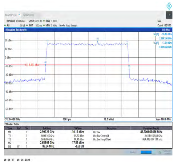
1-N41-PC1.5-30-90-H-5-DFT-256QAM-Outer_Full-2 40@0-Ant1-85.701-89.640-≤90-PASS
