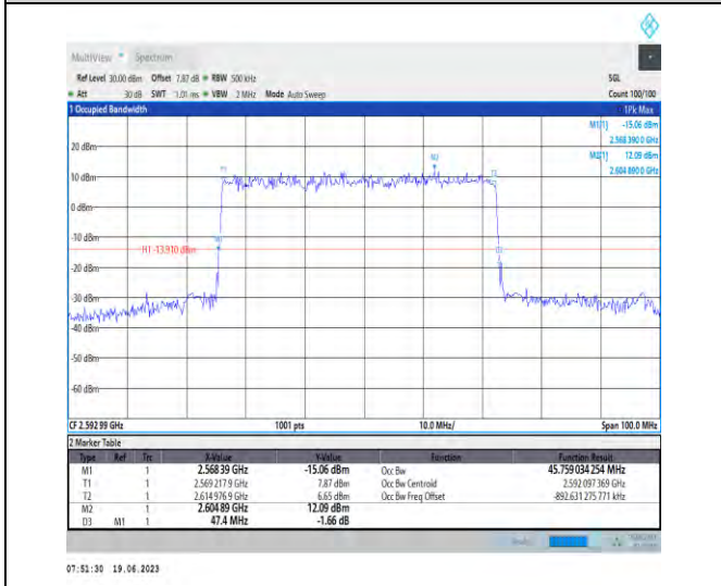
1-N41-PC1.5-30-50-M-5-DFT-256QAM-Outer_Full-1 28@0-Ant1-45.759-47.400-≤50-PASS
