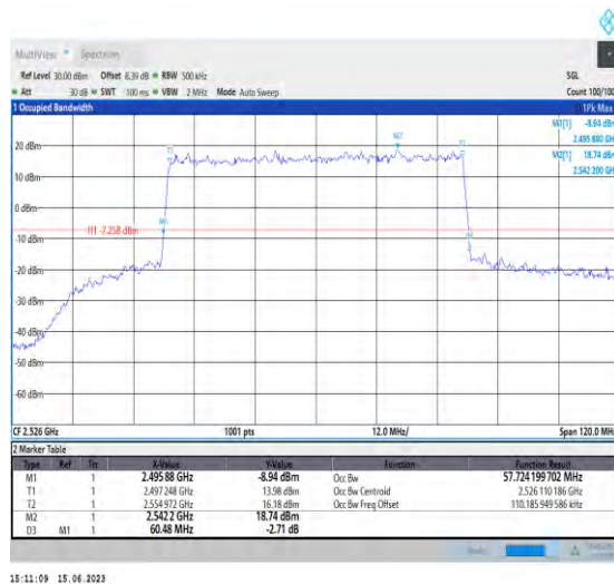
1-N41-PC1.5-30-60-L-4-DFT-64QAM-Outer_Full-162 @0-Ant1-57.724-60.480-≤60-PASS
