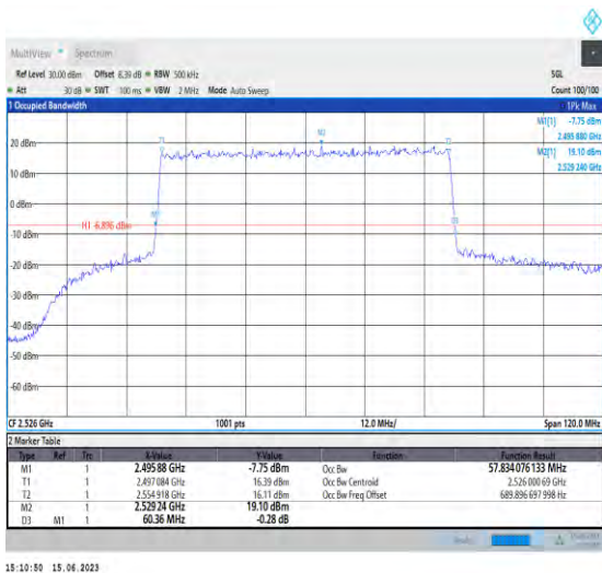
1-N41-PC1.5-30-60-L-3-DFT-16QAM-Outer_Full-162 @0-Ant1-57.834-60.360-≤60-PASS
