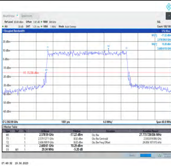
1-N41-PC1.5-30-30-M-9-CP-256QAM-Outer_Full-78 @0-Ant1-27.774-29.340-≤30-PASS
