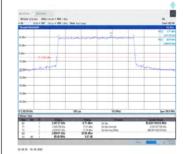
1-N41-PC1.5-30-90-M-1-DFT-QPSK-Outer_Full-240 @0-Ant1-85.659-89.460-≤90-PASS
