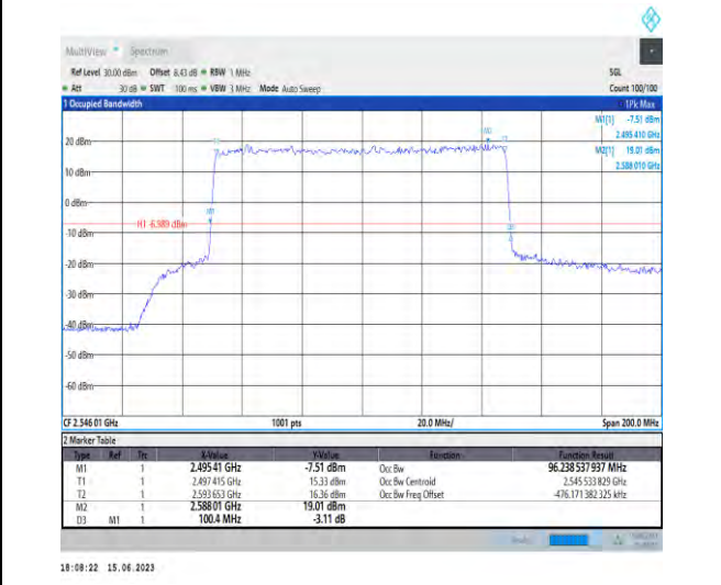
1-N41-PC1.5-30-100-L-4-DFT-64QAM-Outer_Full-270 @0-Ant1-96.239-100.400-≤100-PASS
