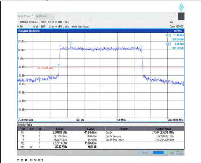
1-N41-PC1.5-30-80-H-6-CP-QPSK-Outer_Full-217@ 0-Ant1-77.574-80.320-≤80-PASS
