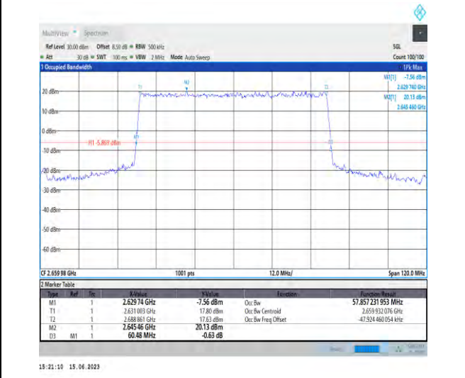
1-N41-PC1.5-30-60-H-2-DFT-PI2BPSK-Outer_Full-1 62@0-Ant1-57.857-60.480-≤60-PASS
