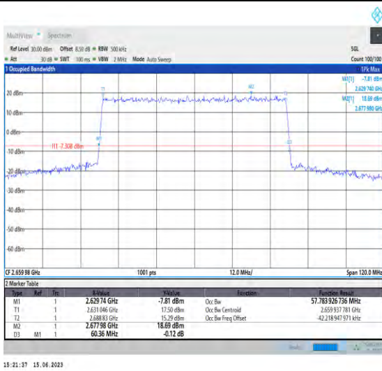
1-N41-PC1.5-30-60-H-3-DFT-16QAM-Outer_Full-16 2@0-Ant1-57.784-60.360-≤60-PASS
