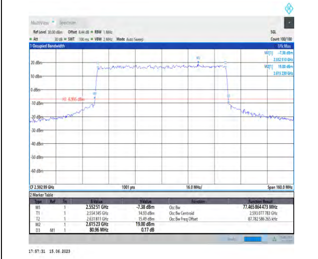
1-N41-PC1.5-30-80-M-8-CP-64QAM-Outer_Full-217 @0-Ant1-77.466-80.960-≤80-PASS
