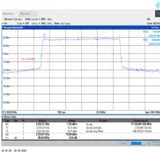
1-N41-PC1.5-30-80-M-4-DFT-64QAM-Outer_Full-21 6@0-Ant1-77.102-80.640-≤80-PASS
