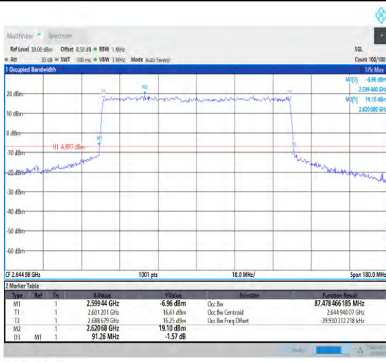
1-N41-PC1.5-30-90-H-6-CP-QPSK-Outer_Full-245@ 0-Ant1-87.478-91.260-≤90-PASS
