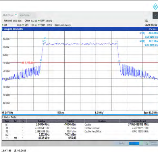
1-N41-PC1.5-30-40-H-9-CP-256QAM-Outer_Full-106@0-Ant1-37.866-40.320-≤40-PASS
