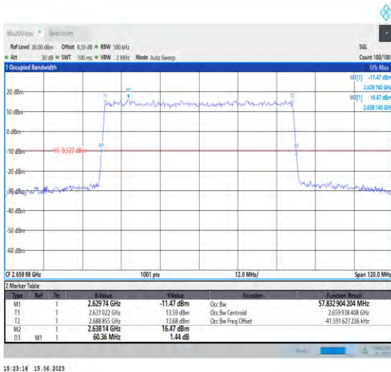
1-N41-PC1.5-30-60-H-5-DFT-256QAM-Outer_Full-1 62@0-Ant1-57.833-60.360-≤60-PASS
