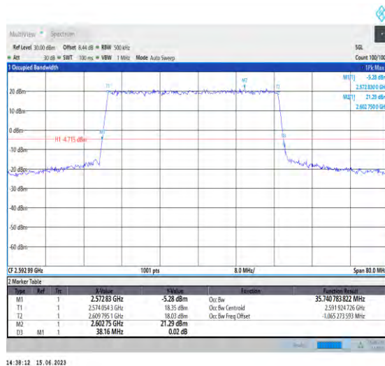
1-N41-PC1.5-30-40-M-1-DFT-QPSK-Outer_Full-100 @0-Ant1-35.741-38.160-≤40-PASS
