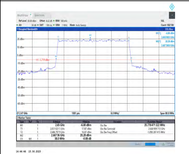
1-N41-PC1.5-30-40-H-4-DFT-64QAM-Outer_Full-100 @0-Ant1-35.776-38.000-≤40-PASS
