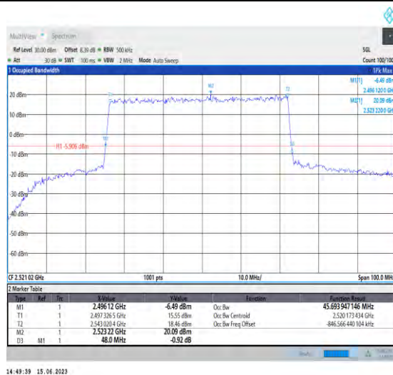
1-N41-PC1.5-30-50-L-3-DFT-16QAM-Outer_Full-128@0-Ant1-45.694-48.000-≤50-PASS
