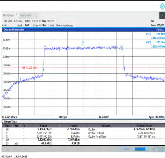
1-N41-PC1.5-30-50-L-6-CP-QPSK-Outer_Full-133@ 0-Ant1-47.421-49.800-≤50-PASS
