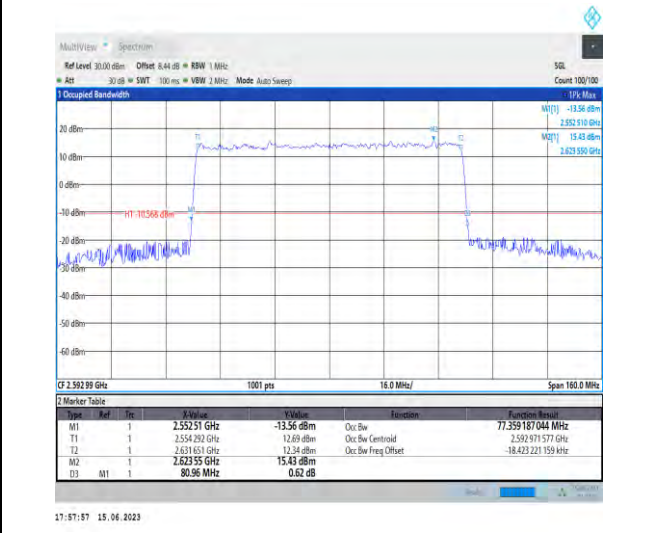
1-N41-PC1.5-30-80-M-9-CP-256QAM-Outer_Full-217 @0-Ant1-77.359-80.960-≤80-PASS
