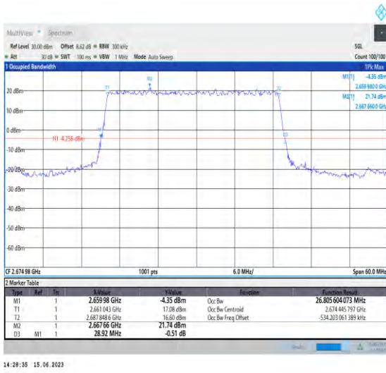
1-N41-PC1.5-30-30-H-2-DFT-PI2BPSK-Outer_Full-75 @0-Ant1-26.806-28.920-≤30-PASS
