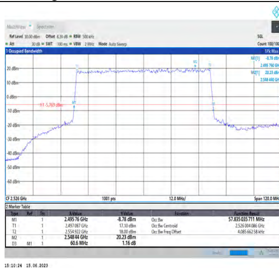
1-N41-PC1.5-30-60-L-2-DFT-PI2BPSK-Outer_Full-162 @0-Ant1-57.835-60.600-≤60-PASS
