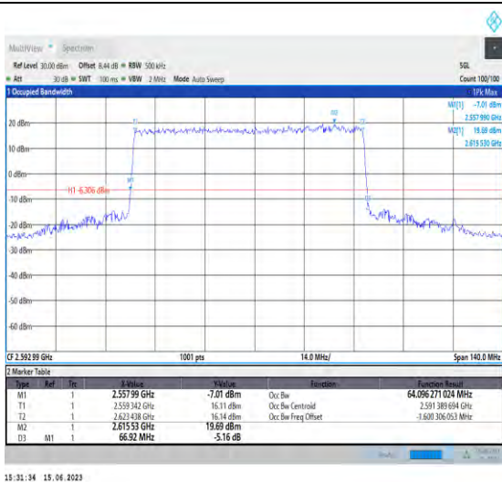
1-N41-PC1.5-30-70-M-1-DFT-QPSK-Outer_Full-180 @0-Ant1-64.096-66.920-≤70-PASS
