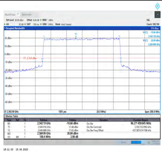
1-N41-PC1.5-30-100-M-1-DFT-QPSK-Outer_Full-27 0@0-Ant1-96.271-100.400-≤100-PASS
