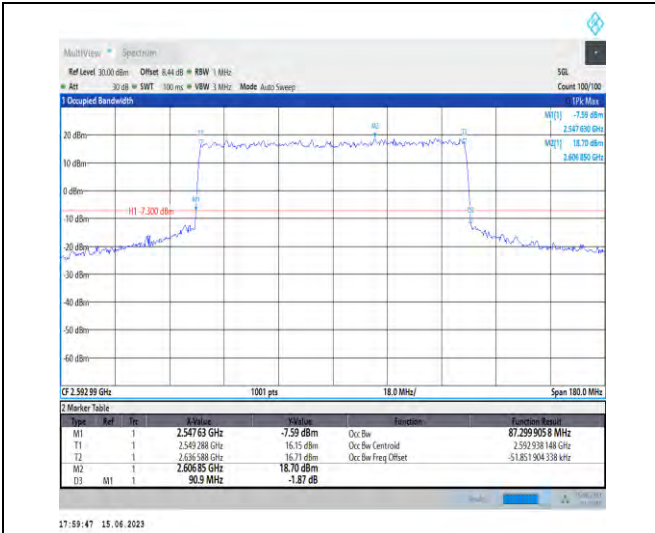
1-N41-PC1.5-30-90-M-7-CP-16QAM-Outer_Full-245 @0-Ant1-87.3-90.900-<math>\leq</math>90-PASS
