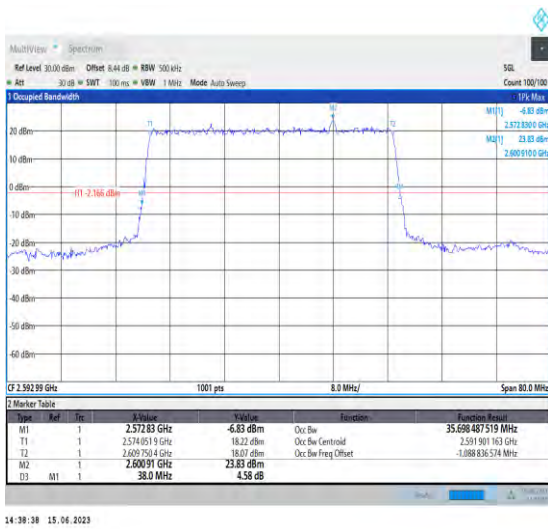
1-N41-PC1.5-30-40-M-2-DFT-PI2BPSK-Outer_Full-100@0-Ant1-35.698-38.000-≤40-PASS
