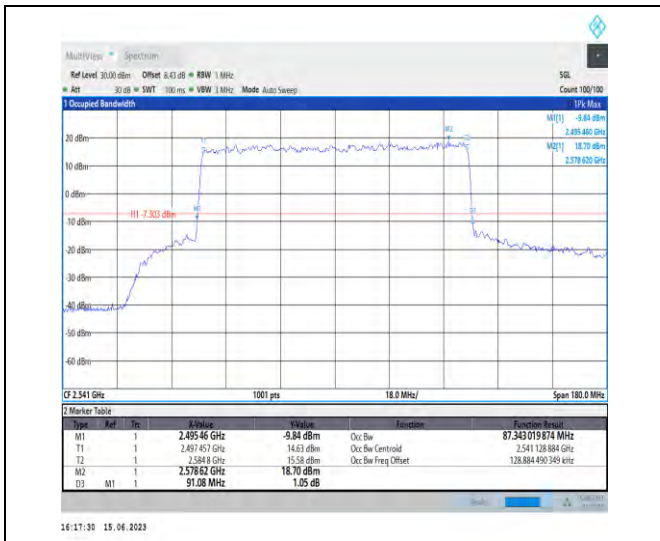
1-N41-PC1.5-30-90-L-8-CP-64QAM-Outer_Full-245 @0-Ant1-87.343-91.080-≤90-PASS
