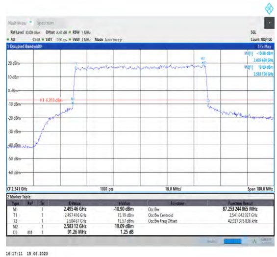
1-N41-PC1.5-30-90-L-7-CP-16QAM-Outer_Full-245 @0-Ant1-87.253-91.260-≤90-PASS
