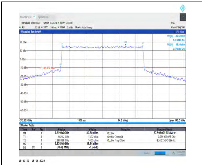
1-N41-PC1.5-30-70-H-8-CP-64QAM-Outer_Full-189 @0-Ant1-67.598-70.420-<=70-PASS
