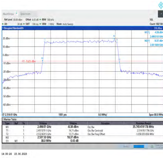
1-N41-PC1.5-30-40-L-5-DFT-256QAM-Outer_Full-100 @0-Ant1-35.745-38.000-≤40-PASS
