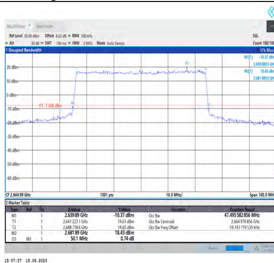
1-N41-PC1.5-30-50-H-7-CP-16QAM-Outer_Full-133 @0-Ant1-47.496-50.100-≤50-PASS
