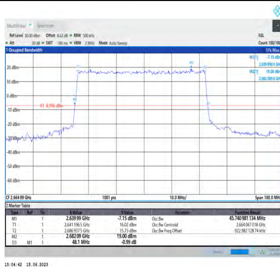
1-N41-PC1.5-30-50-H-1-DFT-QPSK-Outer_Full-128 @0-Ant1-45.741-48.100-≤50-PASS
