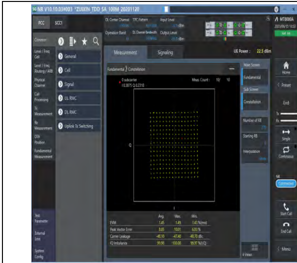
1-N41-PC1.5-30-100-M-5-DFT-256QAM-Outer_Full-2 70@0-Ant1-see graph-PASS
