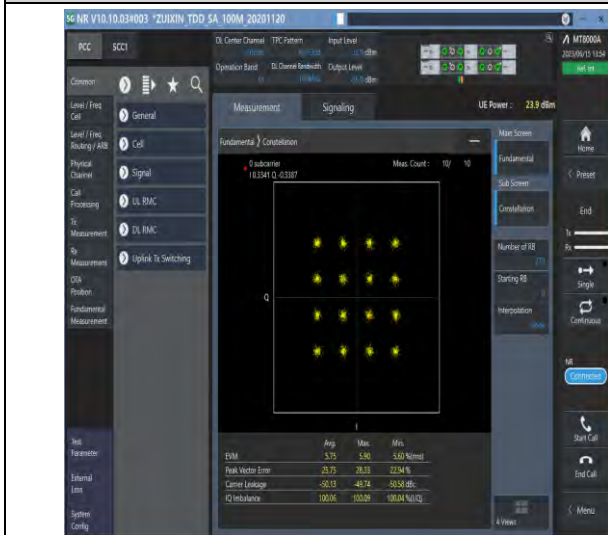
1-N41-PC1.5-30-100-M-7-CP-16QAM-Outer_Full-273 @0-Ant1-see graph-PASS
