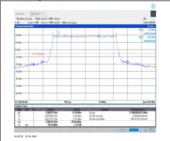
1-N41-PC1.5-30-20-M-1-DFT-QPSK-Outer_Full-50 @0-Ant1-17.91-19.520-<math>\leq 20</math>-PASS
