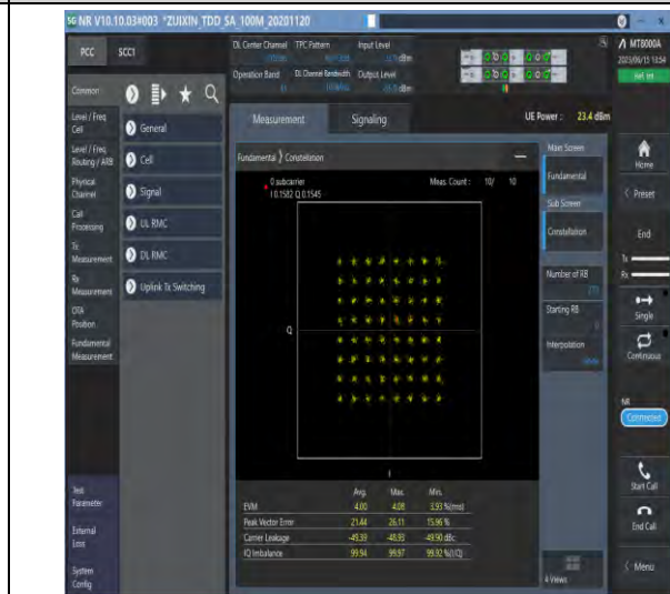
1-N41-PC1.5-30-100-M-8-CP-64QAM-Outer_Full-27 3@0-Ant1-see graph-PASS
