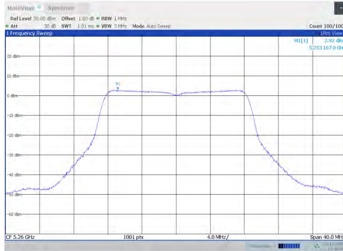
11a-CDD Ant4 5260
