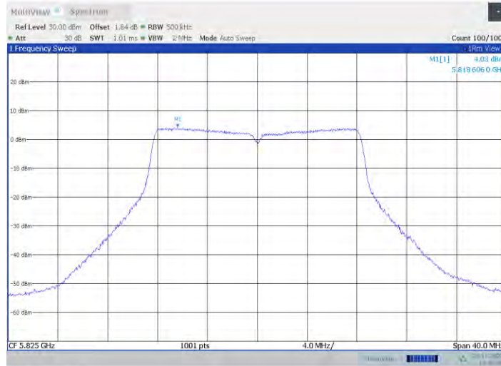
11a-CDD Ant4 5825
