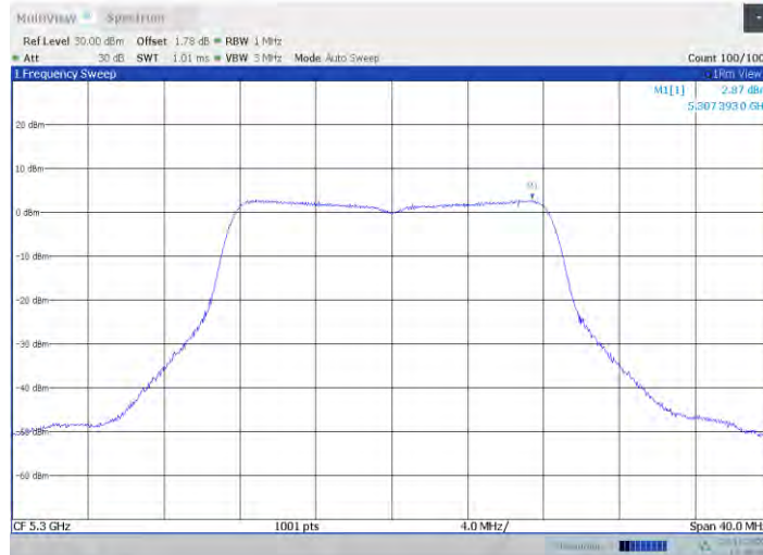
11a-CDD Ant4 5300
