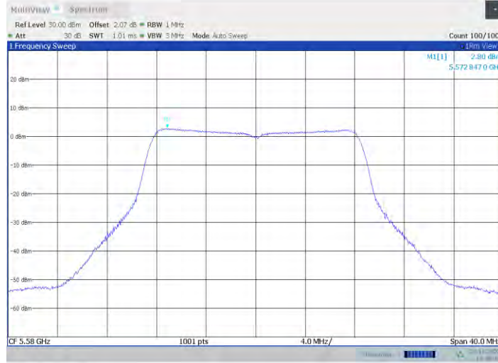
11a-CDD Ant6 5580
