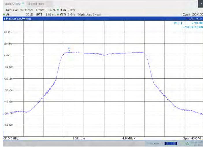
11a-CDD Ant6 5300
