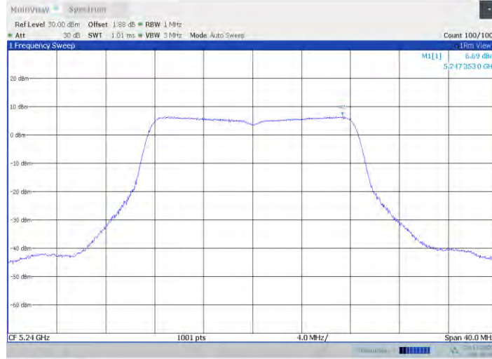
11a-CDD Ant6 5240
