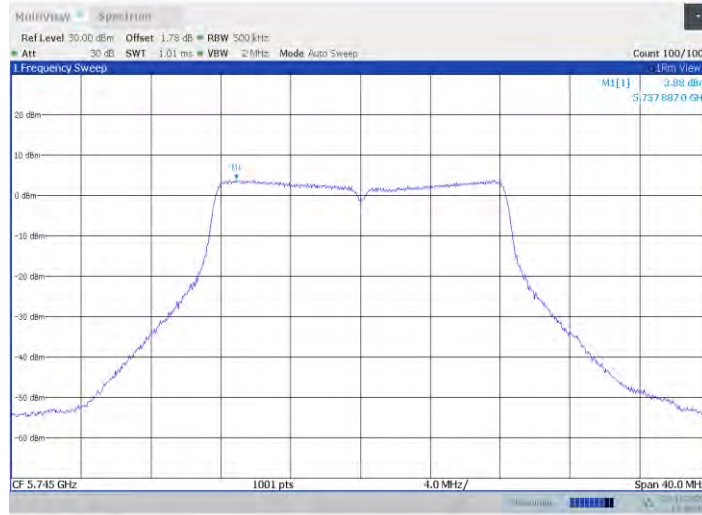
11a-CDD Ant4 5745
