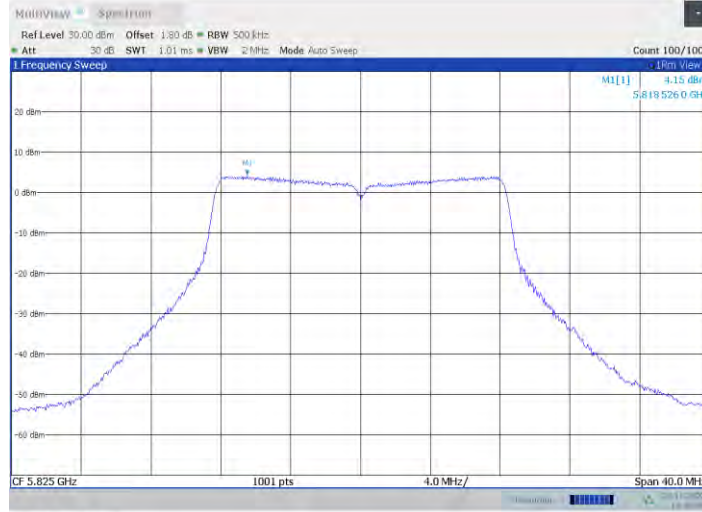
11a-CDD Ant6 5825
