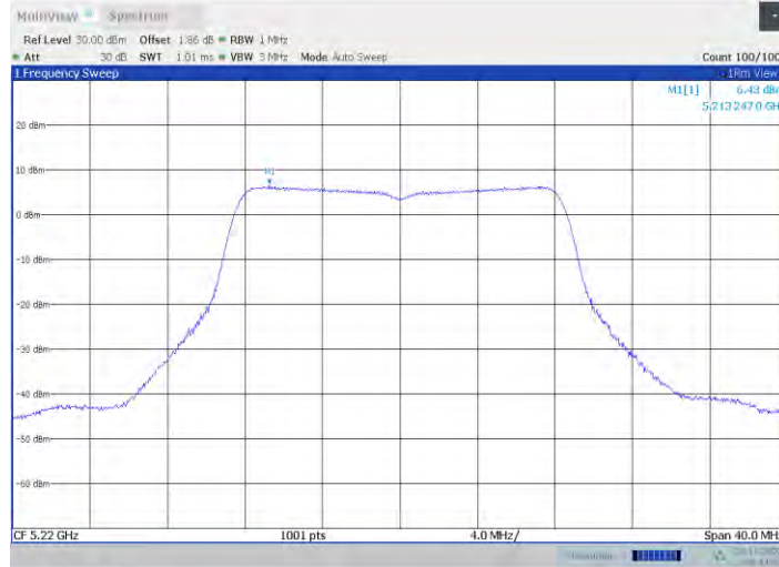
11a-CDD Ant4 5220
