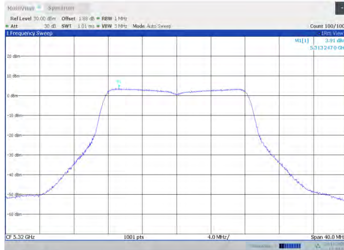
11a-CDD Ant4 5320
