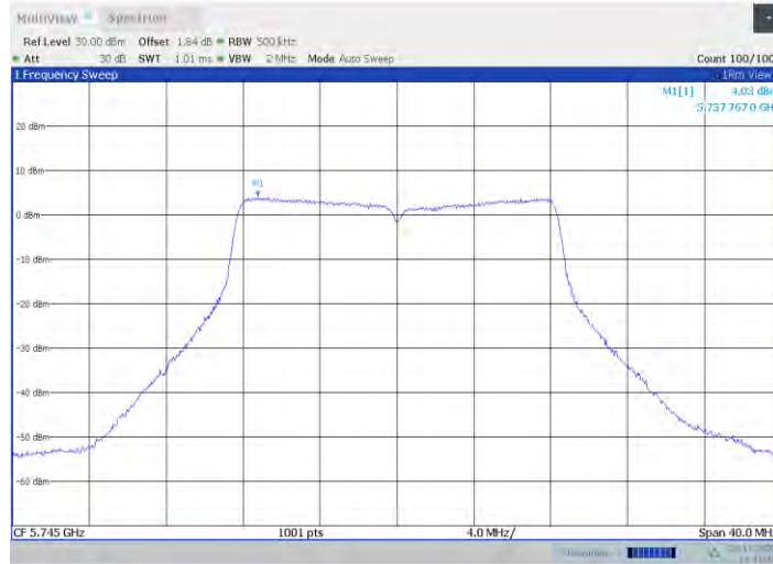
11a-CDD Ant4 5745
