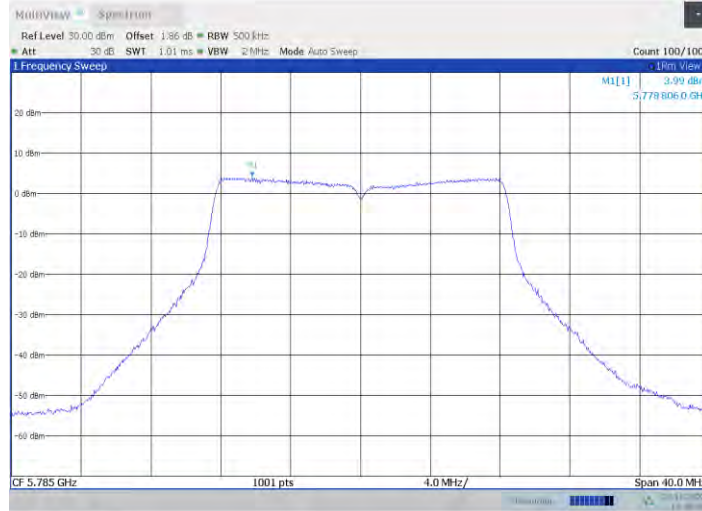
11a-CDD Ant6 5785
