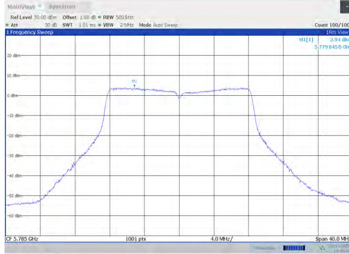
11a-CDD Ant4 5785
