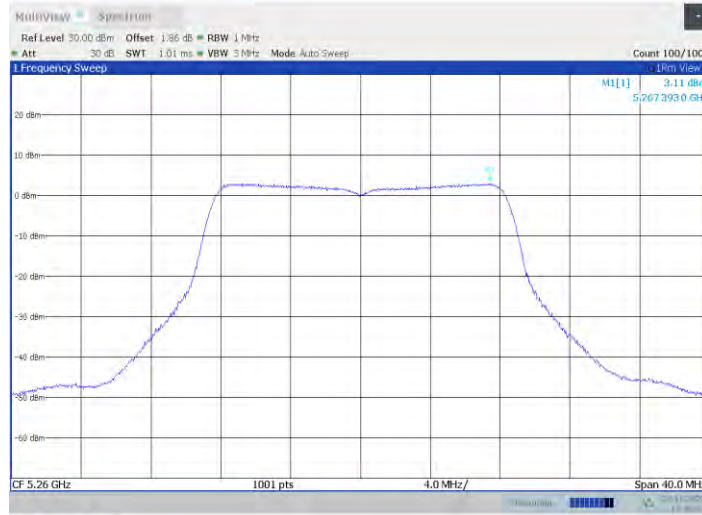
11a-CDD Ant4 5260
