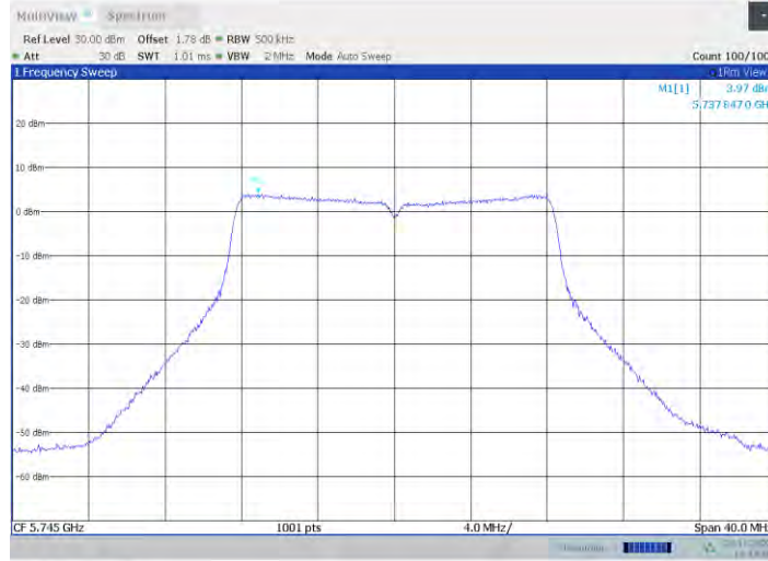
11a-CDD Ant6 5745
