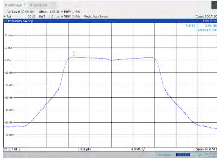
11a-CDD Ant4 5700
