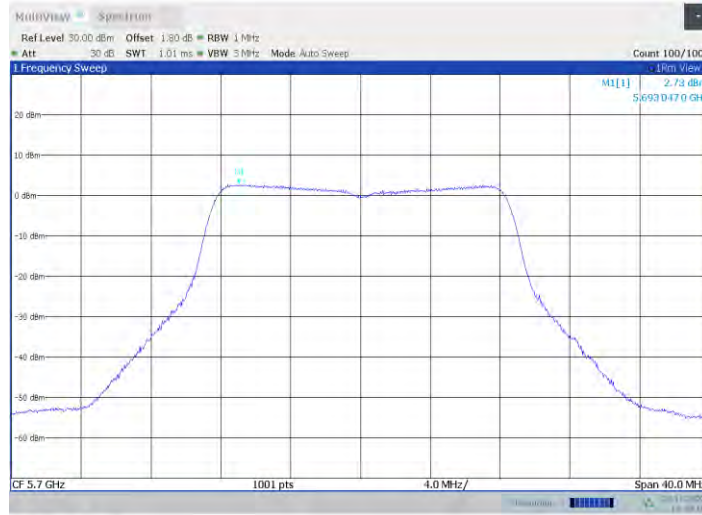
11a-CDD Ant4 5700
