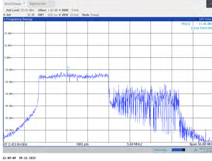
11ax40MIMO Ant2_2422_106RU+26RU+106R_Left
