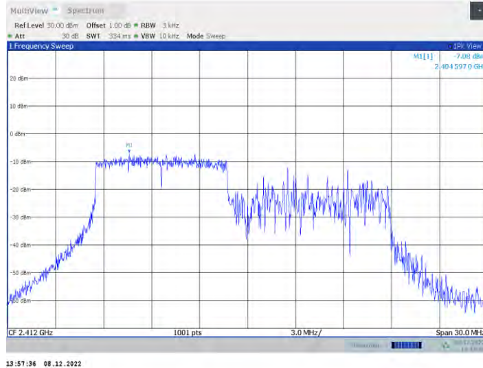
11ax20MIMO_Ant1_2412_26RU+26RU+26RU+26RU_Left
