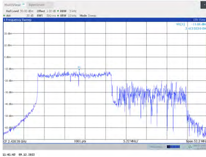
11ax40MIMO Ant2_2422_106RU+26RU+106R_Left
