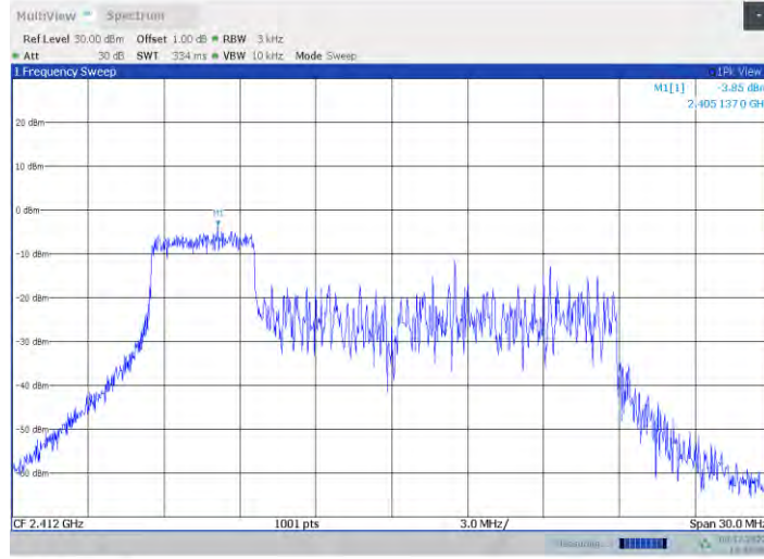
11ax20MIMO_Ant1_2412_26RU+26RU+26RU+26RU_Left
