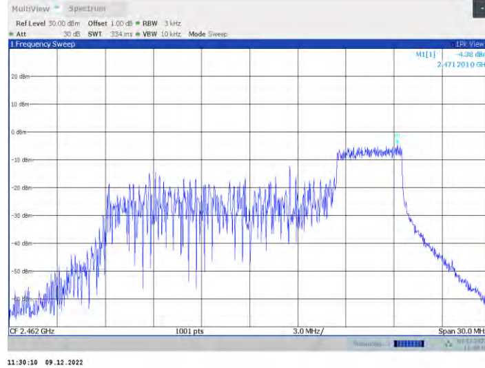
11ax20MIMO_Ant2_2462_26RU+26RU+26RU+26RU_Right
