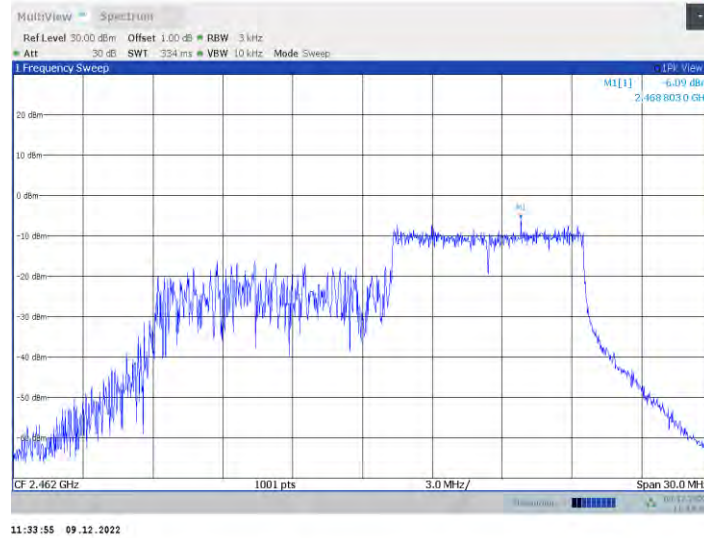
11ax20MIMO_Ant2_2462_26RU+26RU+26RU+26RU_Right
