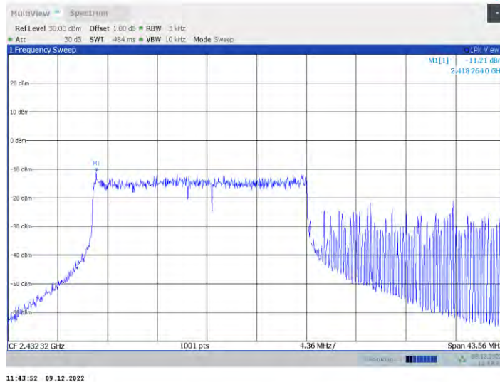
11ax40MIMO Ant2_2437_106RU+26RU+106R_Left
