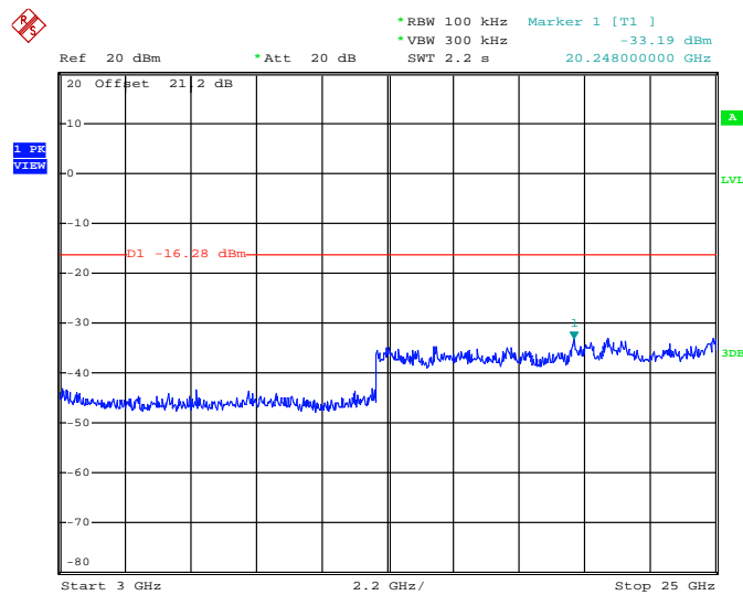
Mode 1: Conducted Spurious Emission Plot on 802.11b between 3 GHz~25 GHz - Chain A
