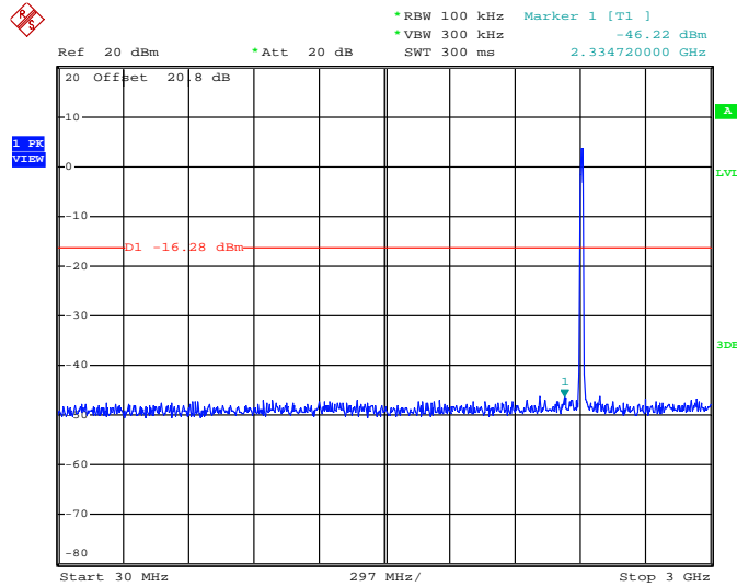
Mode 1:Conducted Spurious Emission Plot on 802.11b between 30 MHz~3 GHz - Chain A
