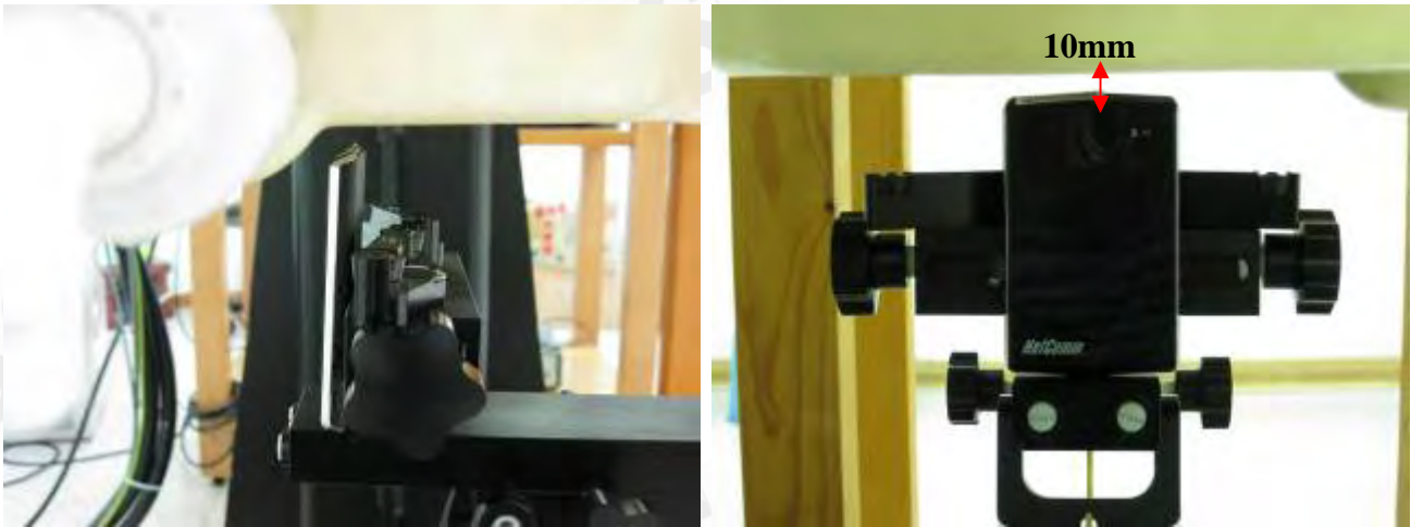
Fig.5 Top side of EUT is paralleled with flat phantom and spacing between EUT and Phantom is 10mm.
