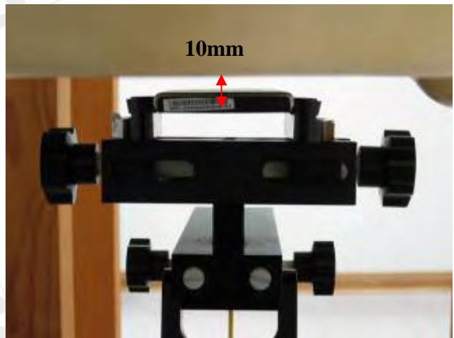
Fig.4 Back side of EUT is paralleled with flat phantom and spacing between EUT and Phantom is 10mm.
