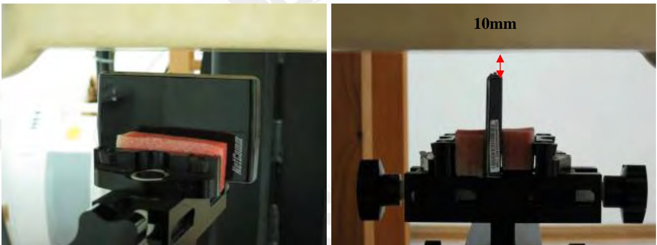
Fig.6 Right side of EUT is paralleled with flat phantom and spacing between EUT and Phantom is 10mm.
