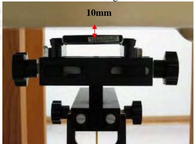
Fig.3 Front side of EUT is paralleled with flat phantom and spacing between EUT and Phantom is 10mm.
