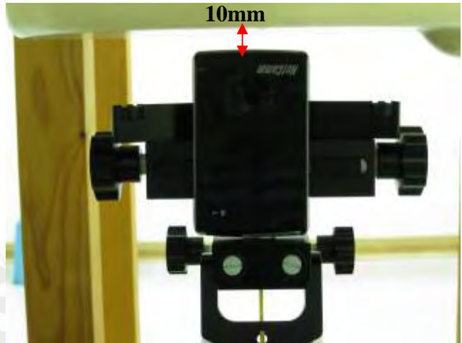
Fig.8 Bottom side of EUT is paralleled with flat phantom and spacing between EUT and Phantom is 10mm.
