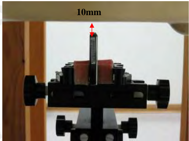
Fig.7 Left side of EUT is paralleled with flat phantom and spacing between EUT and Phantom is 10mm.
