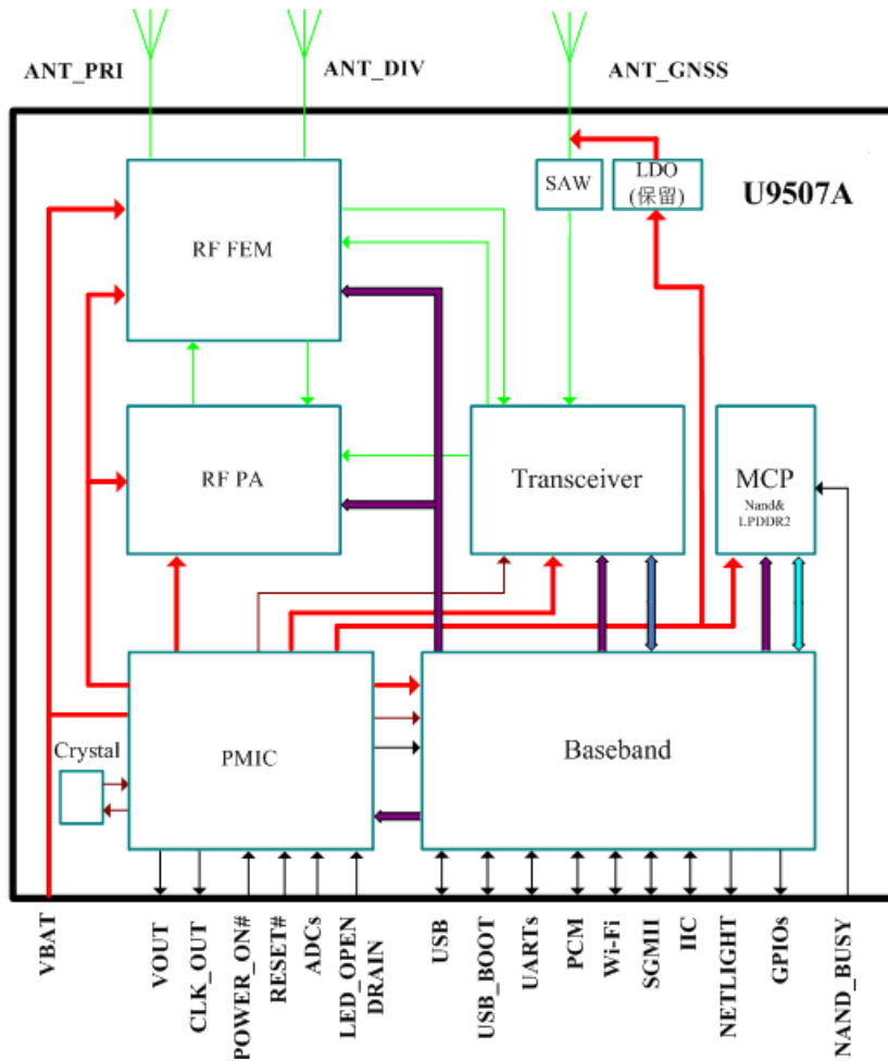
Figure1-1 U9507A application scenario
