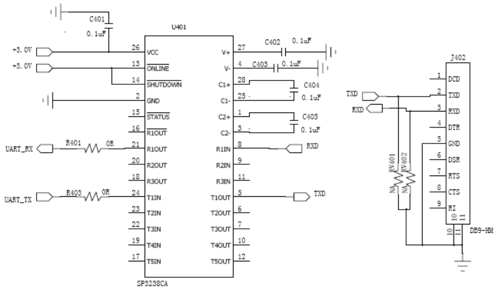
Figure 2-17 The reference circuit of UART interface
