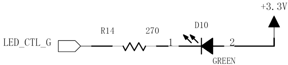
Figure 2-18 The reference circuit of LED control
