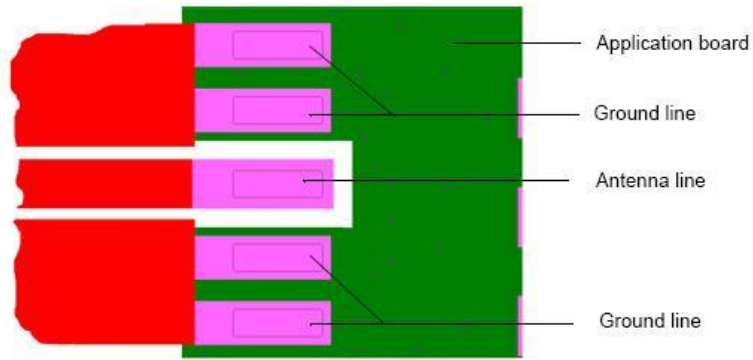
Figure 2-7 Micro-Stripline on 1.0mm standard FR4 2-layer PCB-example 1
