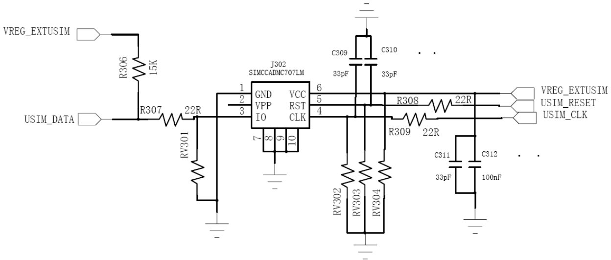
Figure 2-15 The reference circuit of USIM interface
