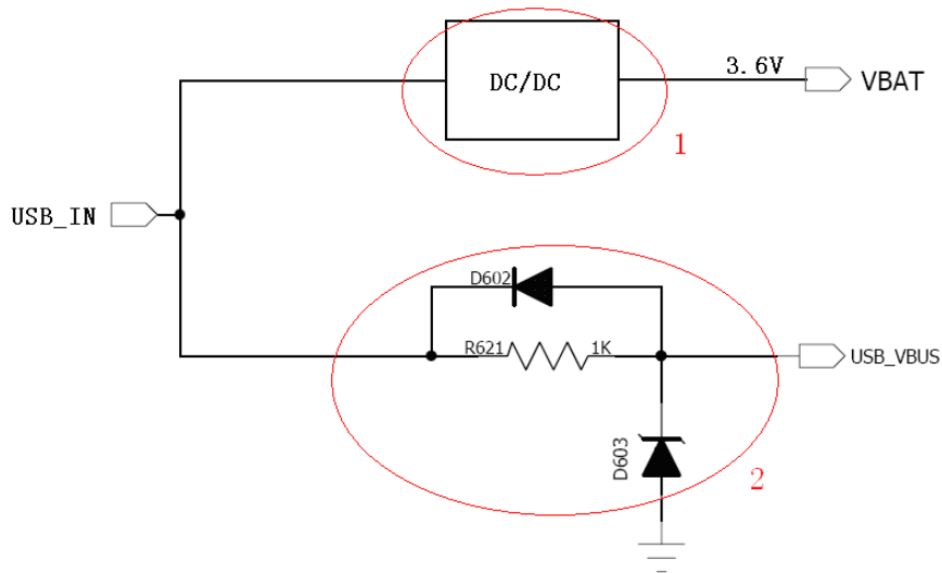
Figure2-14 The reference of voltage protection circuit
