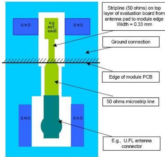
Figure 2-11 Routing to application's RF connector
