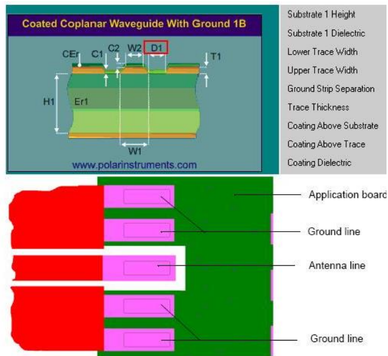
Figure 2-9 Micro-Stripline on 1.5mm standard FR4 2-layer PCB-example 1
