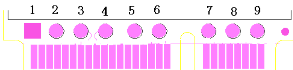
Figure 2-3 Test points of U9507A
