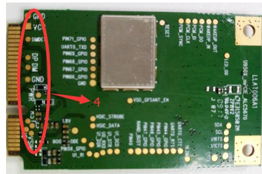
Figure 2-2 The rear view of U9507A
