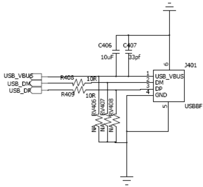
Figure 2-13 The reference circuit of USB interface
