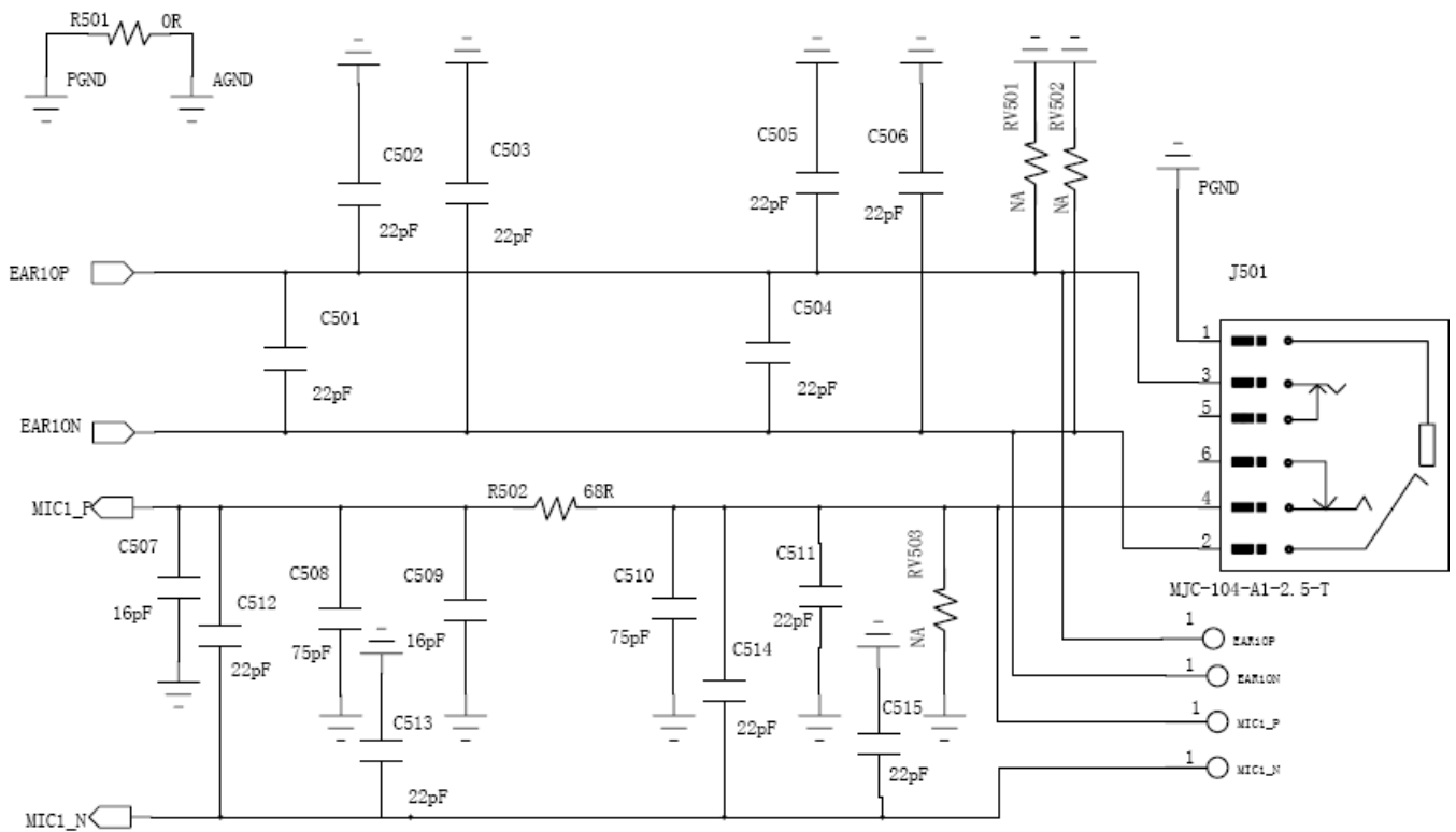
Figure 2-16 The reference circuit of audio interface
