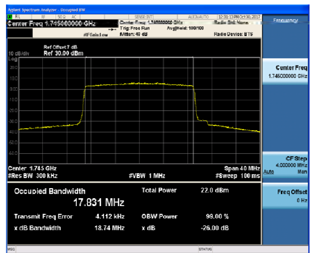
LTE Band 4 QPSK 20MHz CH-High
