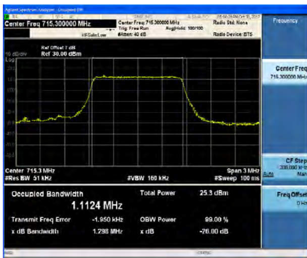
LTE Band 12 QPSK 1.4MHz CH-High
