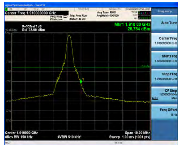
LTE Band 2 15MHz QPSK 1RB CH-High
