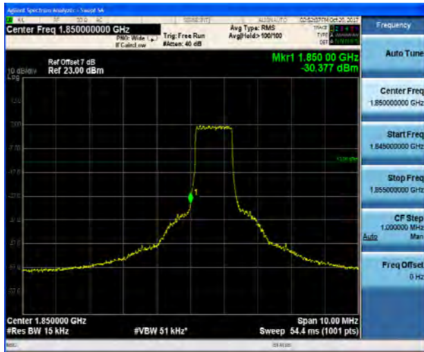
LTE Band 2 3MHz 16QAM 1RB CH-Low
