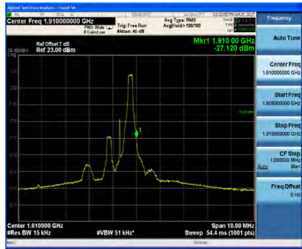
LTE Band 2 1.4MHz 16QAM 100%RB CH-High
