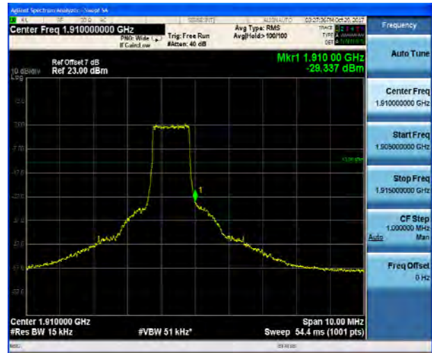
LTE Band 2 3MHz 16QAM 1RB CH-High
