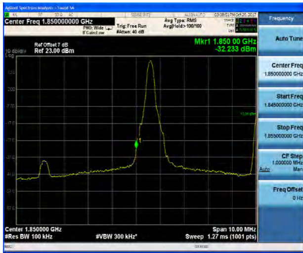
LTE Band 2 10MHz QPSK 100%RB CH-Low
