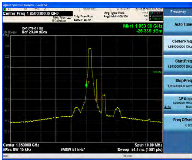
LTE Band 2 1.4MHz 16QAM 100%RB CH-Low
