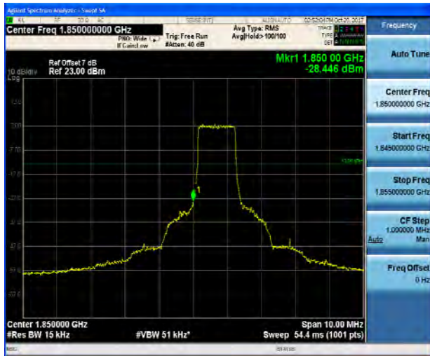
LTE Band 2 3MHz QPSK 1RB CH-Low
