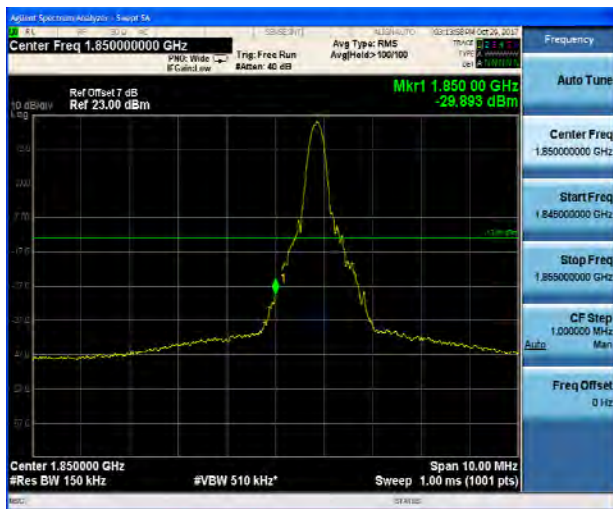
LTE Band 2 15MHz QPSK 1RB CH-Low
