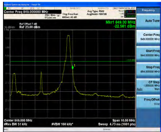
LTE Band 5 QPSK 5MHz CH-High 1RB
