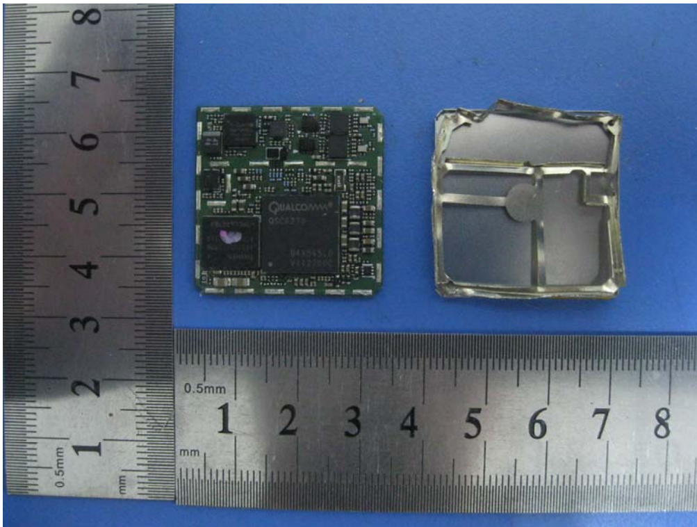
Uncover Without Shielding - Top View 1
