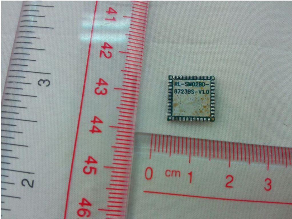
RF BOARD 1
