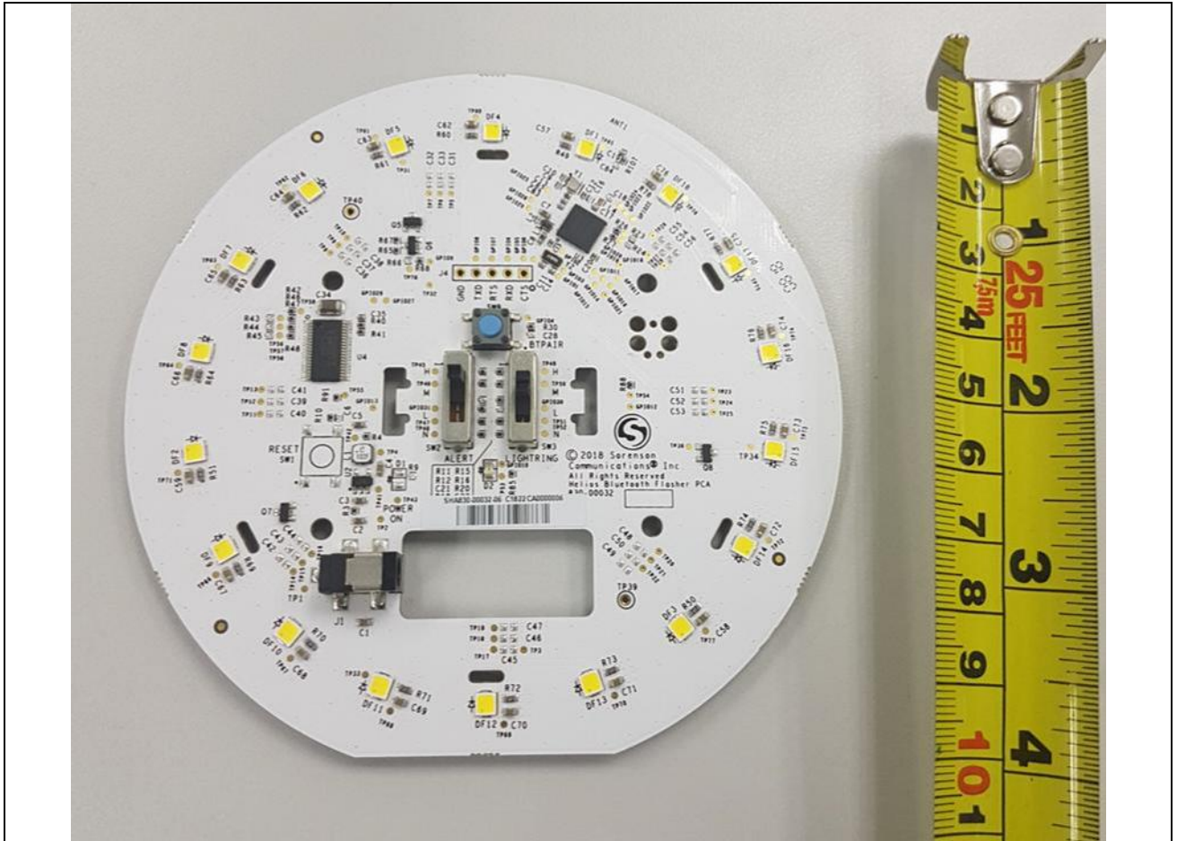
Component Side View
