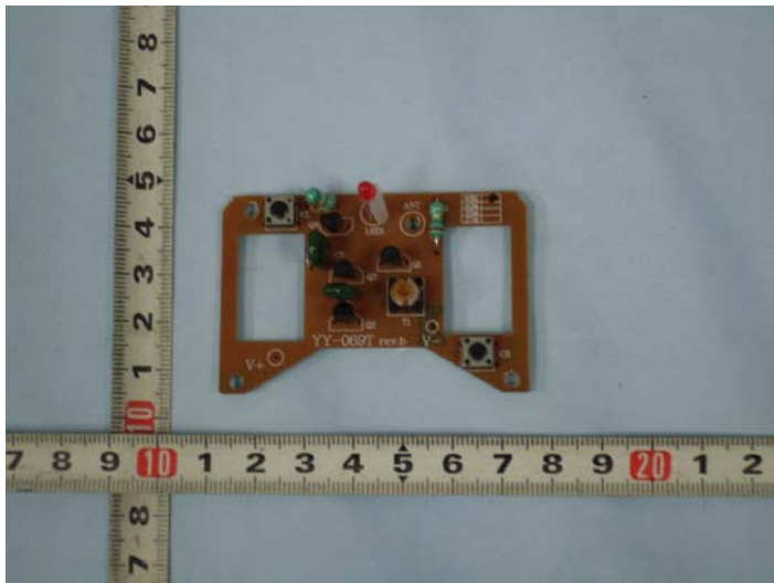
EUT-PCB View (Transmitter)
