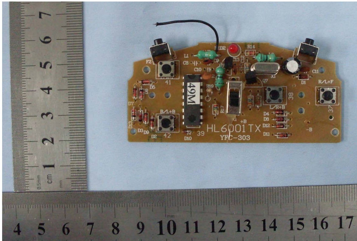
EUT-PCB View (Transmitter)
