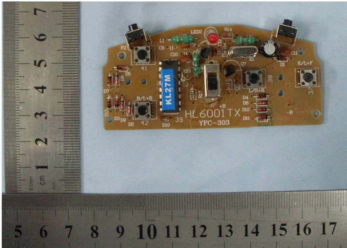
EUT-PCB View (Transmitter)
