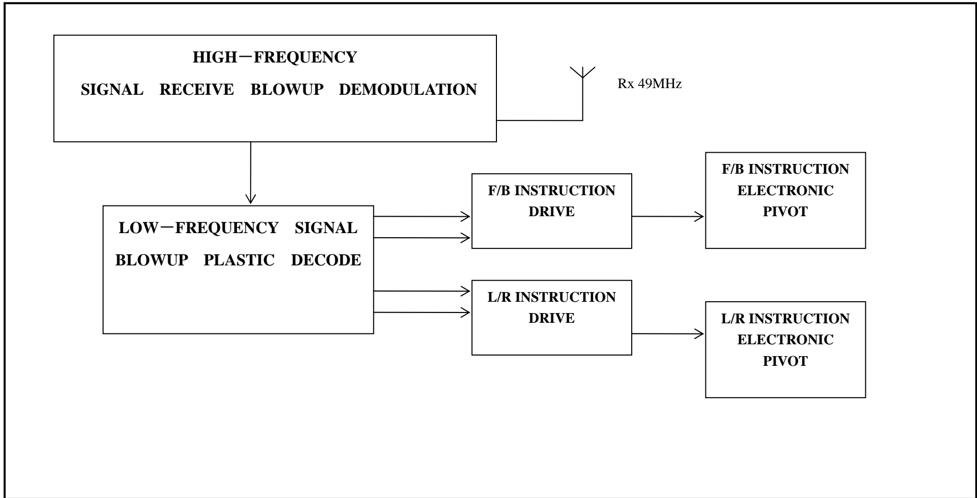
Block Diagram
