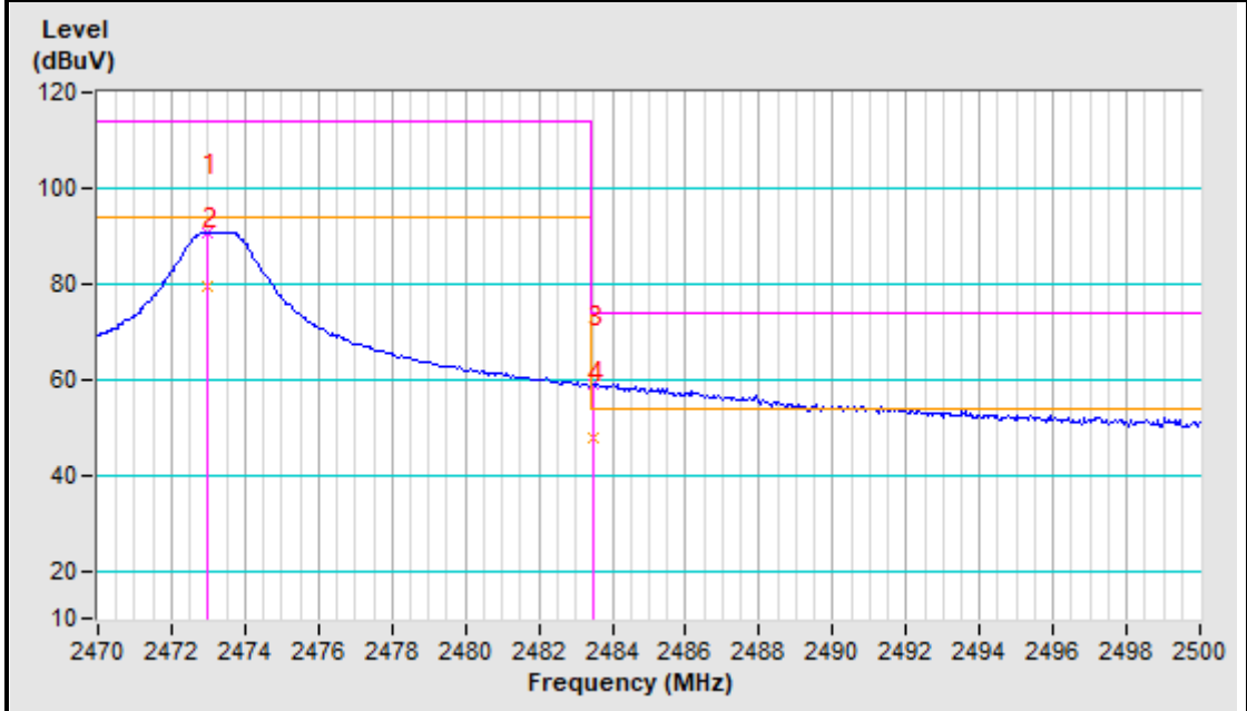
2473MHz Vertical
