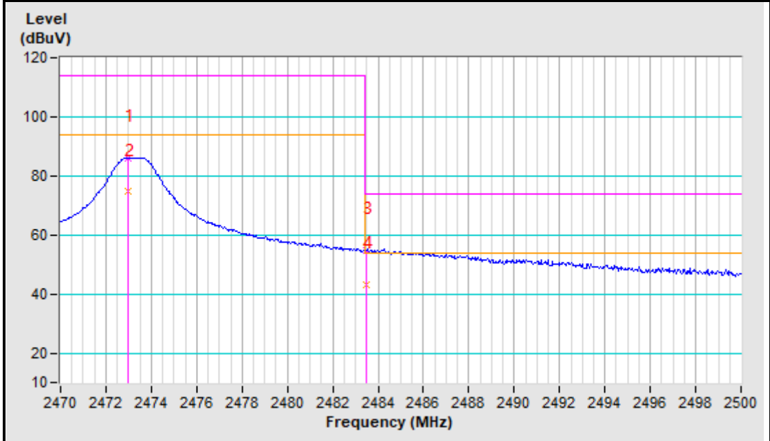
2473MHz Vertical
