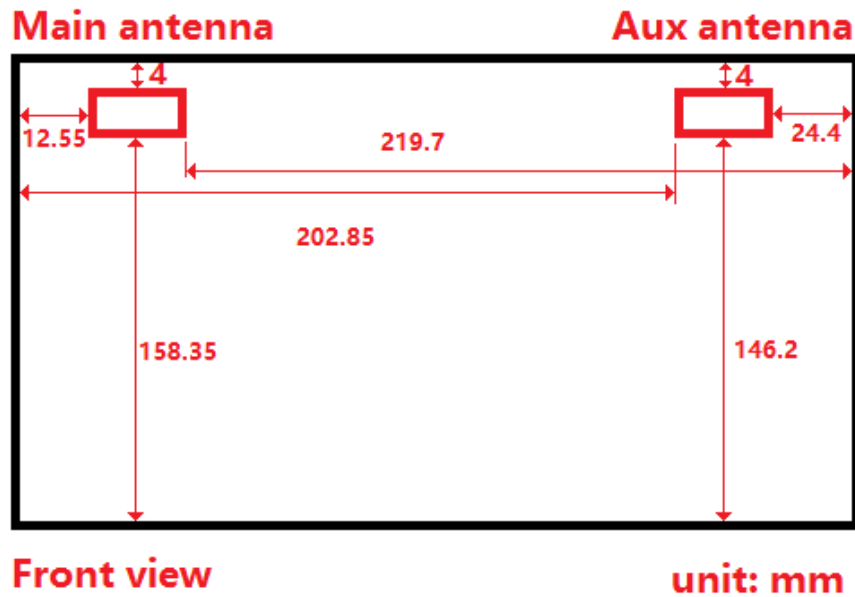
Fig.11 Antenna location
