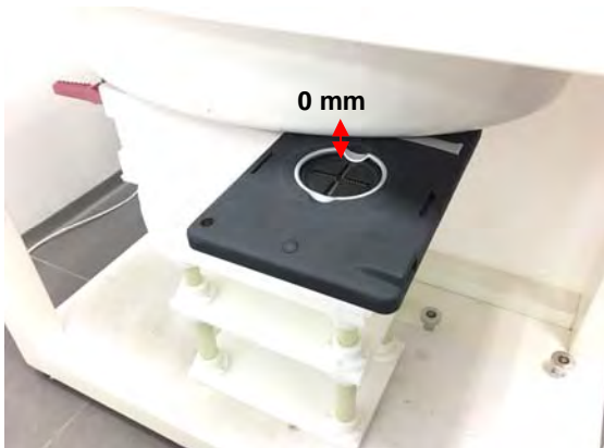
Fig.3 EUT Back side_Main to flat phantom
