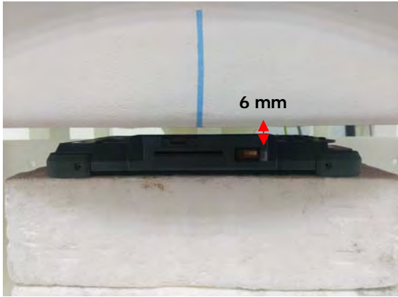
Fig.6 EUT back side to flat phantom
