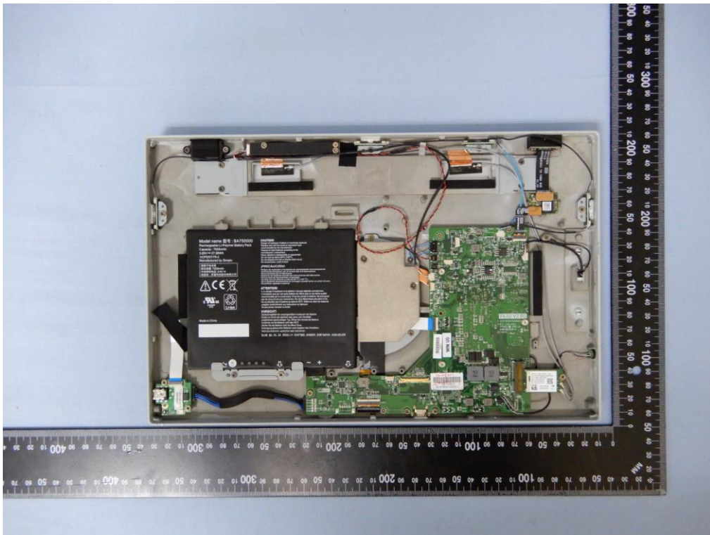
Open View of EUT-2_M278WHL
