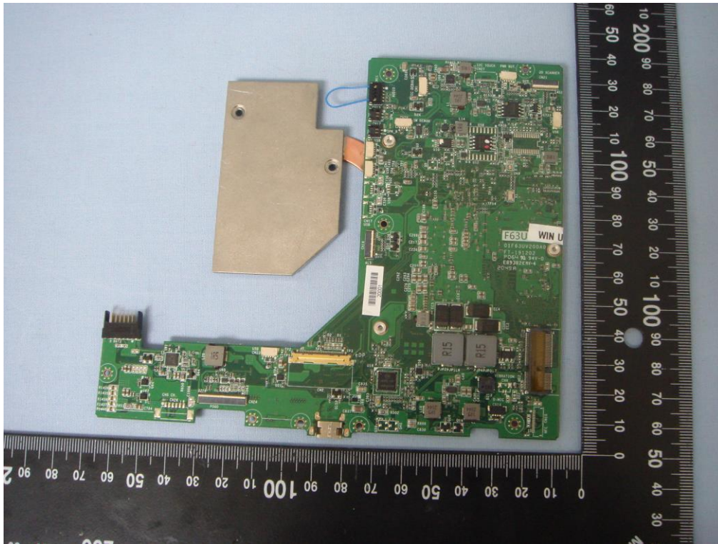
Internal View of EUT –4_M278WHL
