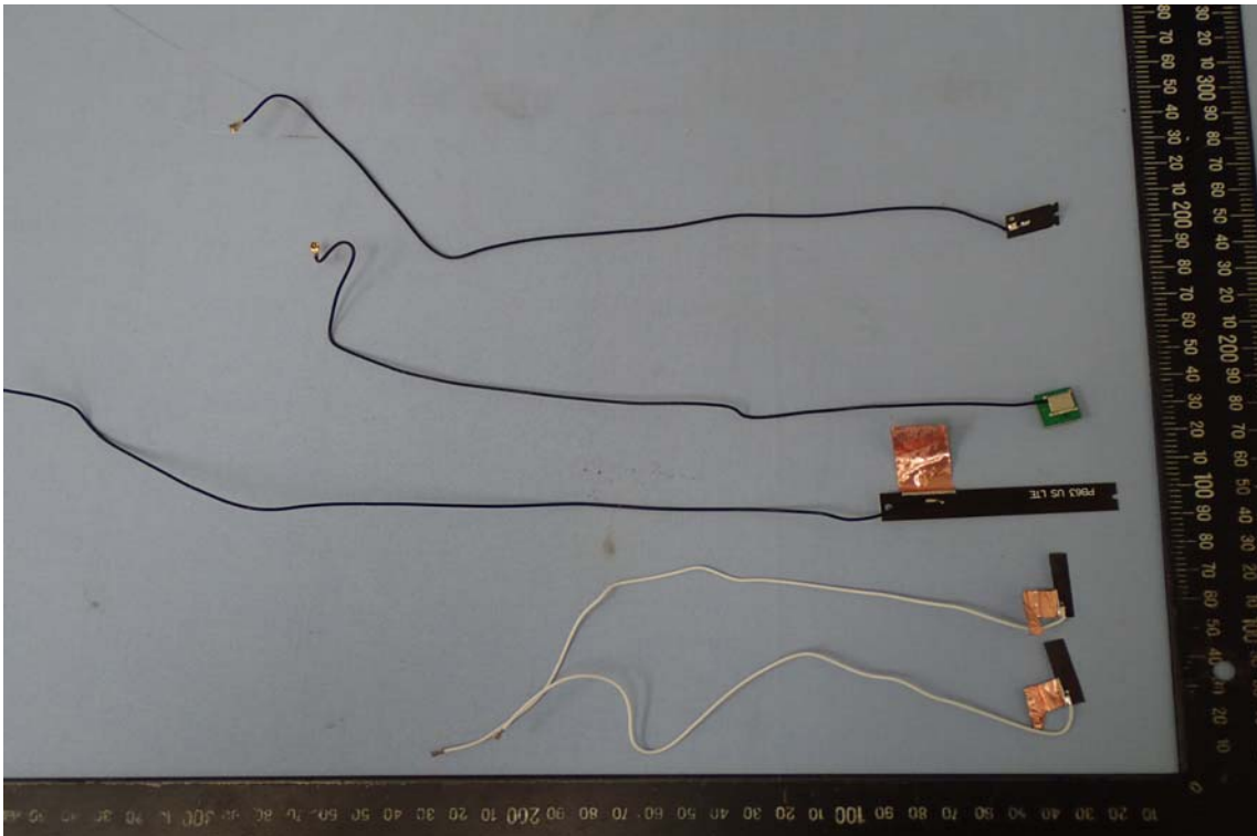
WLAN / WWAN / GPS Antenna - 1
