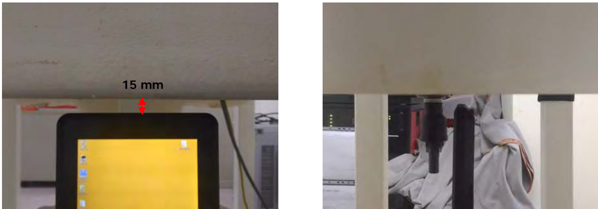
Fig.7 EUT Left side (15mm) to flat phantom
