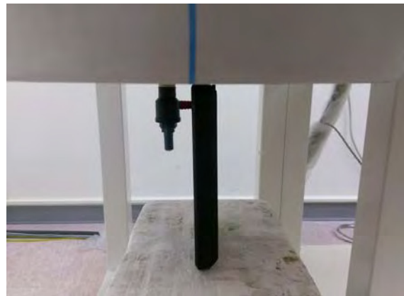
Fig.7 EUT Left side (0mm) to flat phantom
