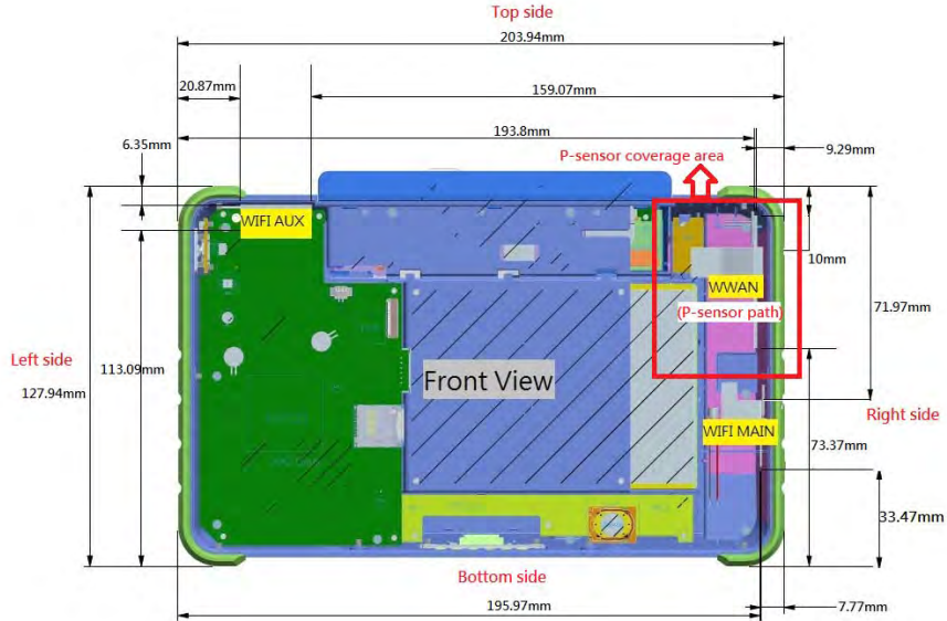
Fig.13 Antenna position of EUT (Front view)
