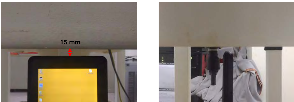
Fig.8 EUT Left side (15mm) to flat phantom
