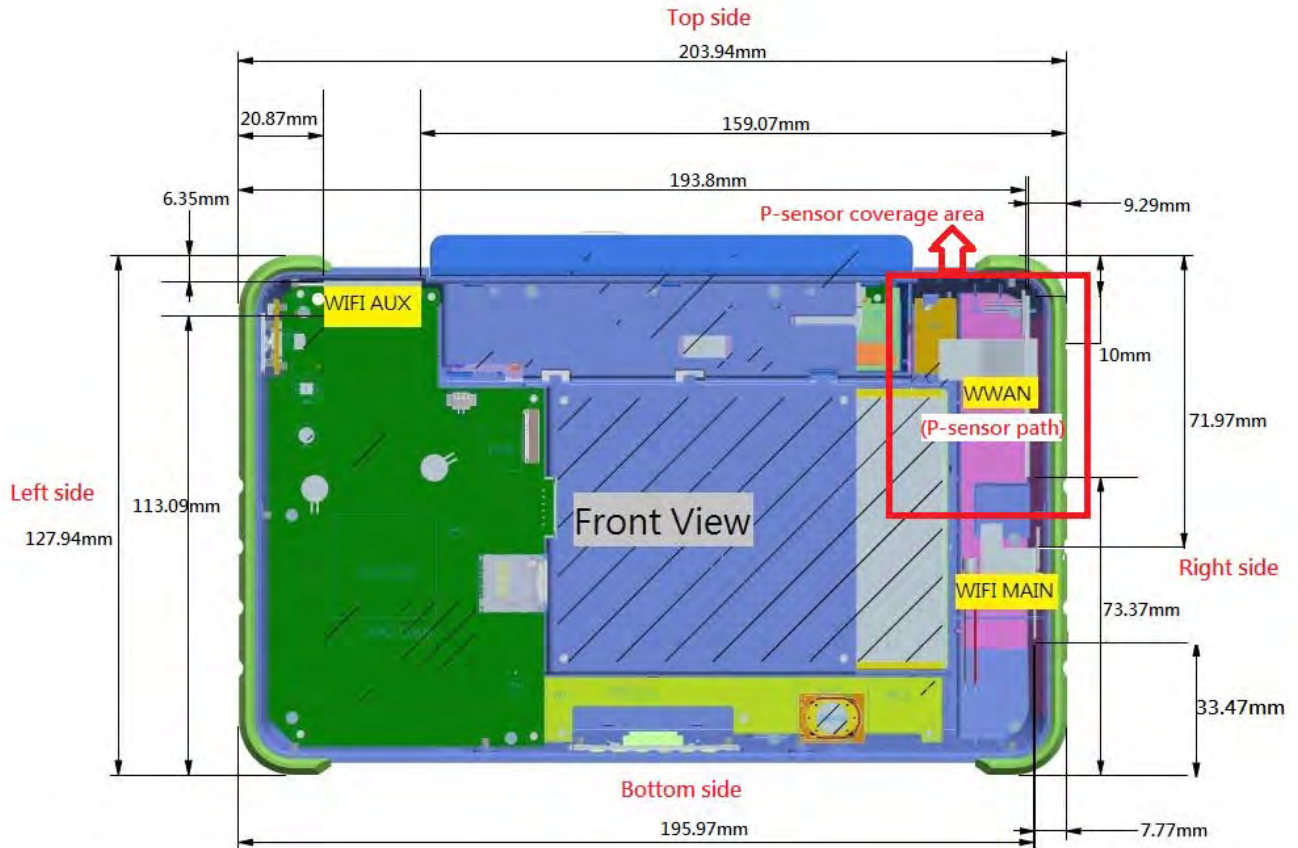
Fig.14 Antenna position of EUT (Front view)
