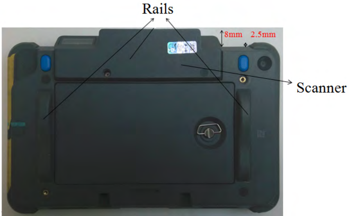
Fig.12 Back view of EUT(with scanner and rails)
