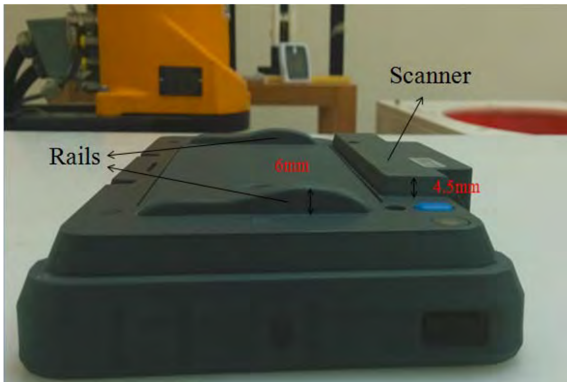
Fig.13 Side view of EUT(with scanner and rails)
