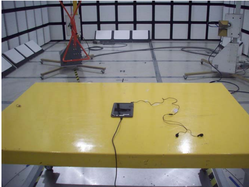
X-AXIS WITH LAPTOP PHOTO
