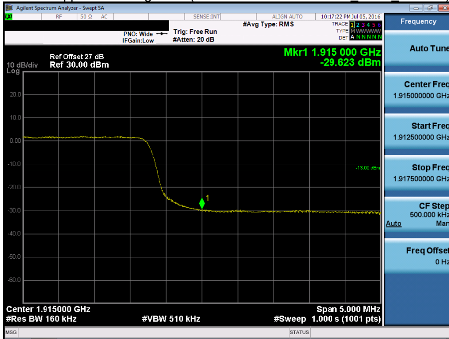
BAND 25. Upper Band Edge Plot (15M BW Ch. 26615 QPSK RB75 Offset 0) -2
