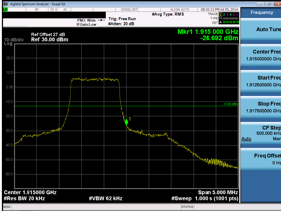
BAND 25. Upper Band Edge Plot (1.4M BW Ch. 26683 QPSK_RB6_Offset 0) -2
