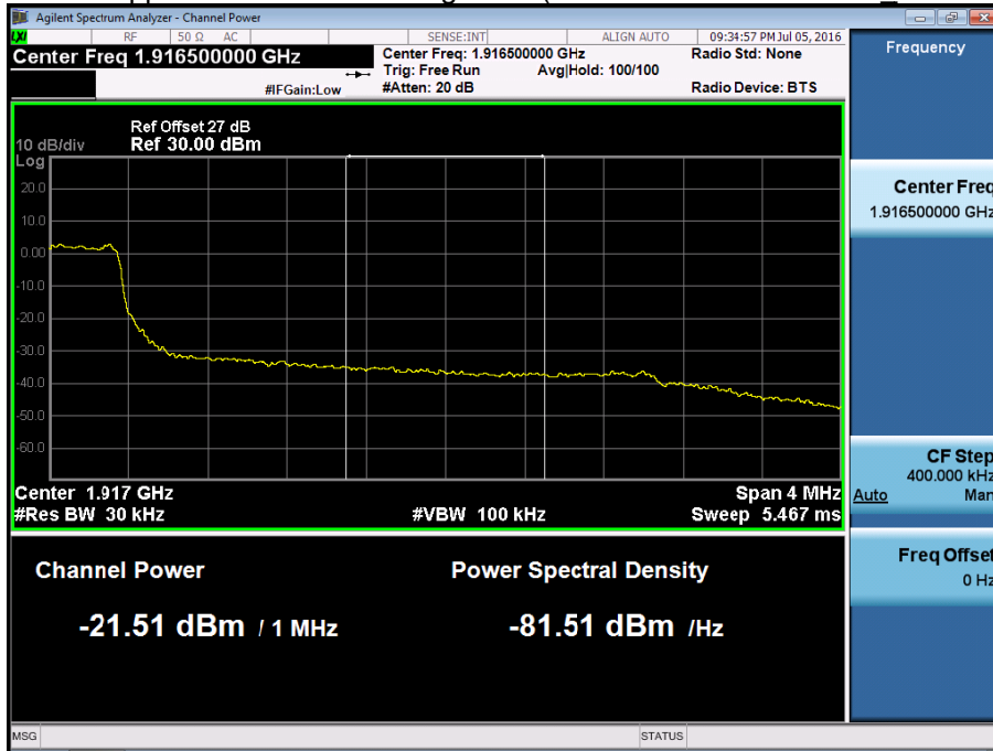
BAND 25. Upper Extended Band Edge Plot (3M BW Ch. 26675 QPSK_RB15 0) -3
