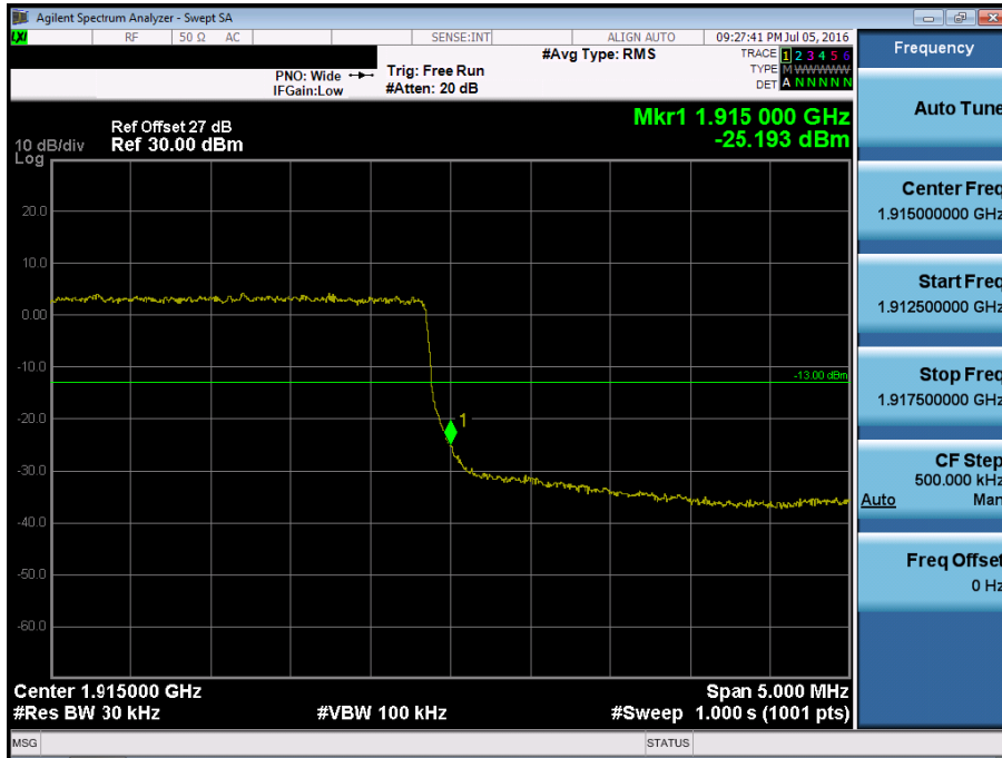
BAND 25. Upper Band Edge Plot (3M BW Ch. 26675 QPSK_RB15_Offset 0) -2
