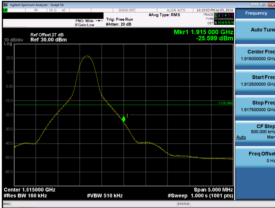
BAND 25. Upper Band Edge Plot (15M BW Ch.26615 QPSK_RB1_Offset 74) -1
