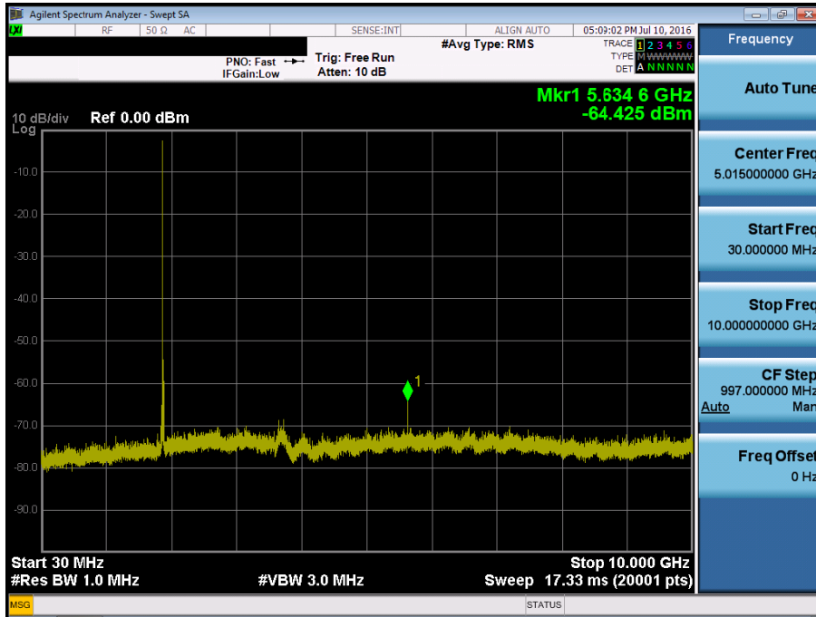
BAND 25. Conducted Spurious_1 (26365 ch_10MHz_QPSK_RB 1_0)
