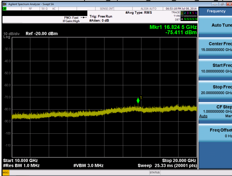
BAND 25. Conducted Spurious_2 (26365 ch 10MHz QPSK RB 1_0)
