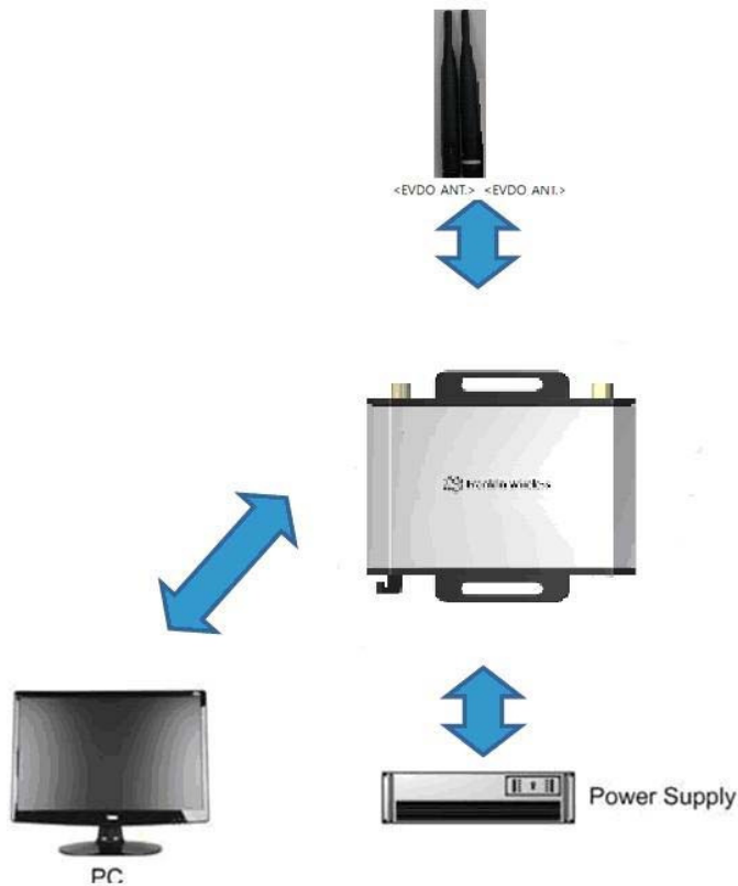
2. Diagram of connecting the S600C and the antenna Figure-3. Diagram of connecting the module and the antenna
