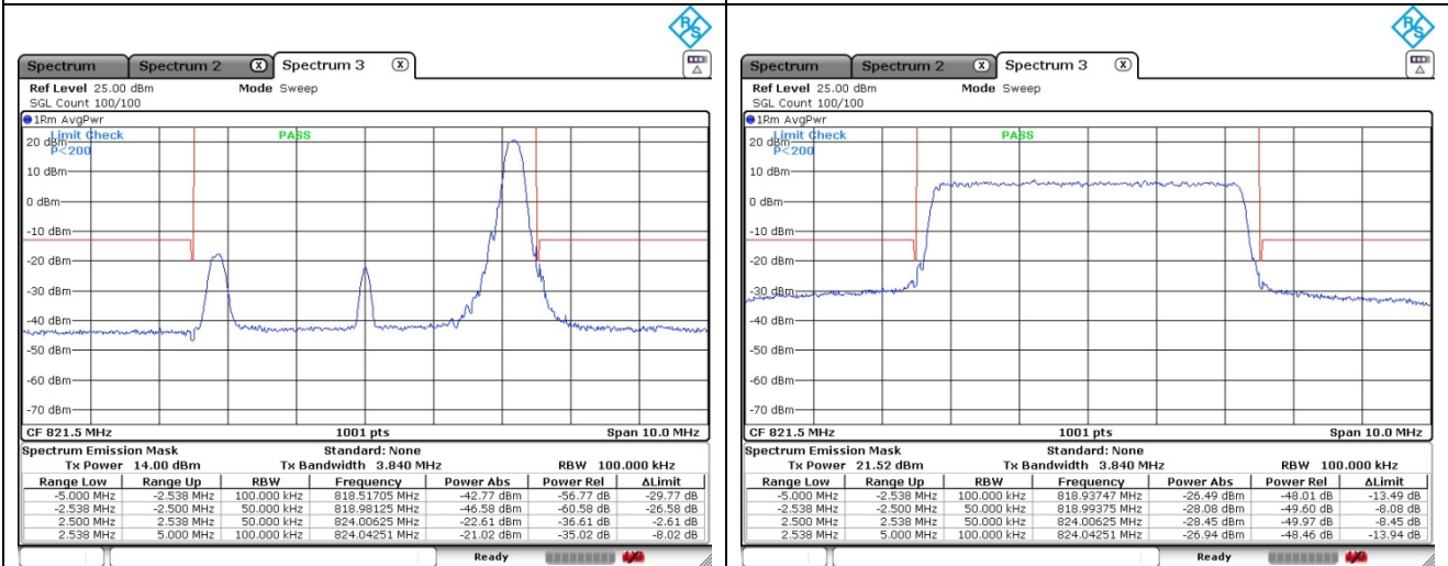
5 MHz QPSK High Channel - 1 RB
