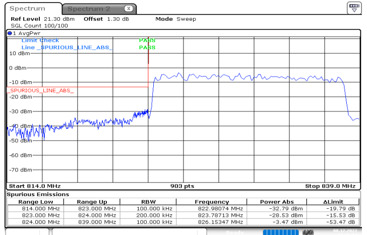
n5_15MHz_15kHz_831.5MHz_DFT-s-OFDM QPSK_RB75@0
