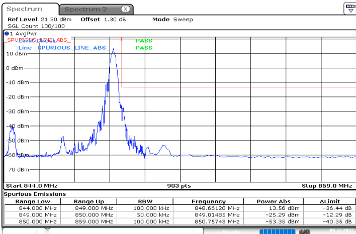
n5_5MHz_15kHz_846.5MHz_DFT-s-OFDM QPSK_RB1@24
