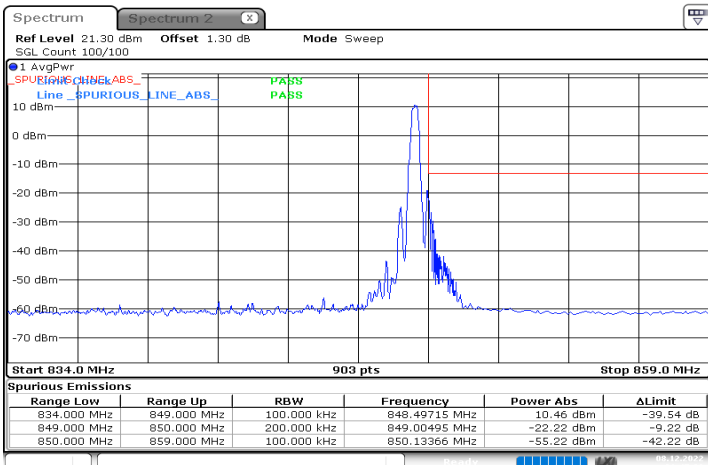
n5_15MHz_15kHz_841.5MHz_DFT-s-OFDM QPSK_RB1@78
