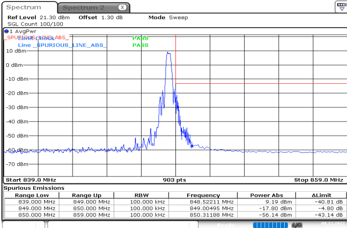
n5_10MHz_15kHz_844MHz_DFT-s-OFDM QPSK_RB1@51
