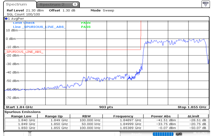
n2_5MHz_15kHz_1852.5MHz_DFT-s-OFDM QPSK_RB25@0
