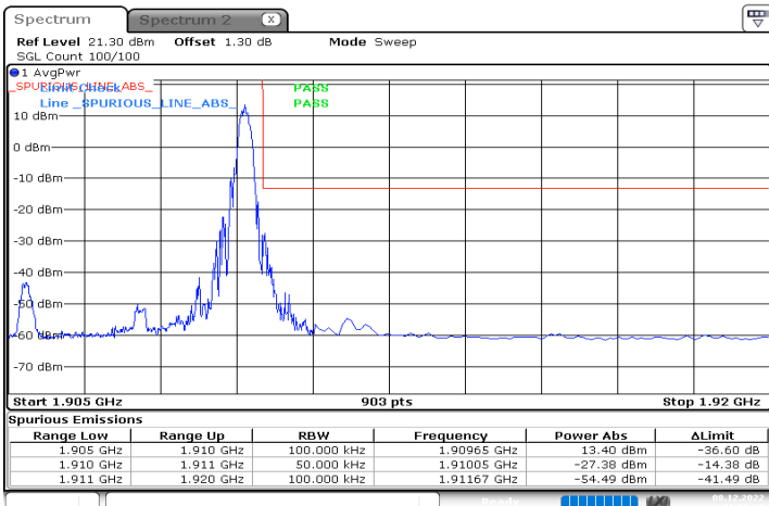
n2_5MHz_15kHz_1907.5MHz_DFT-s-OFDM QPSK_RB1@24
