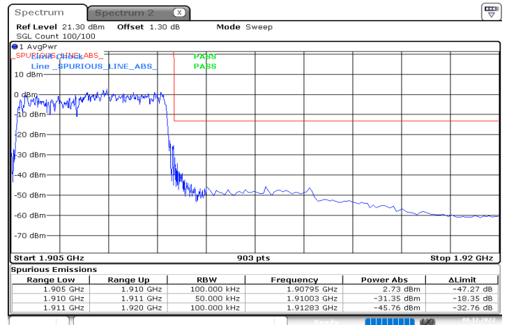
n2_5MHz_15kHz_1907.5MHz_DFT-s-OFDM QPSK_RB25@0
