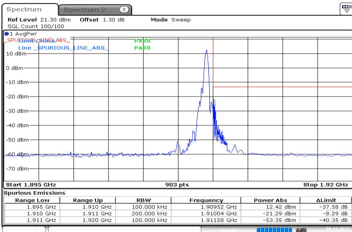
n2_15MHz_15kHz_1902.5MHz_DFT-s-OFDM QPSK_RB1@78
