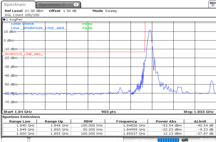
n2_5MHz_15kHz_1852.5MHz_DFT-s-OFDM QPSK_RB1@0
