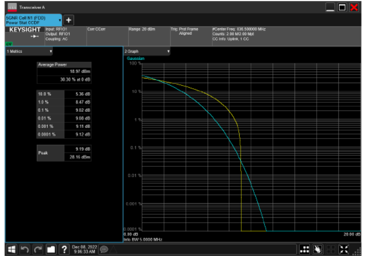
n5_5MHz_15kHz_836.5MHz_CP-OFDM QPSK_RB25@0
