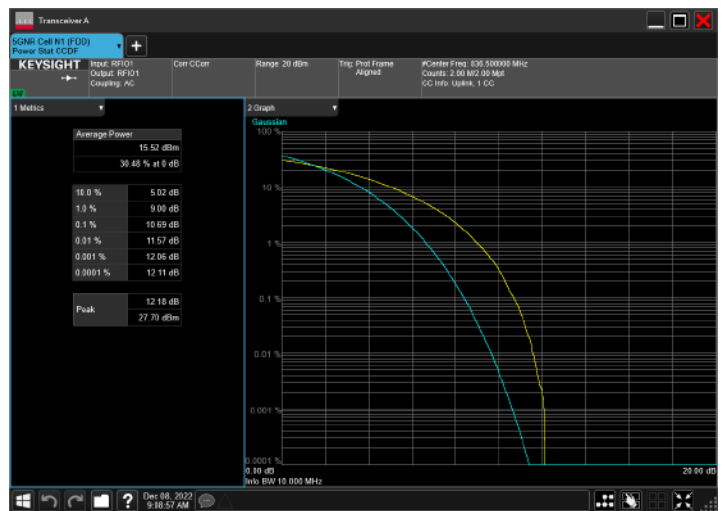
n5_10MHz_15kHz_836.5MHz_CP-OFDM 256 QAM_RB52@0
