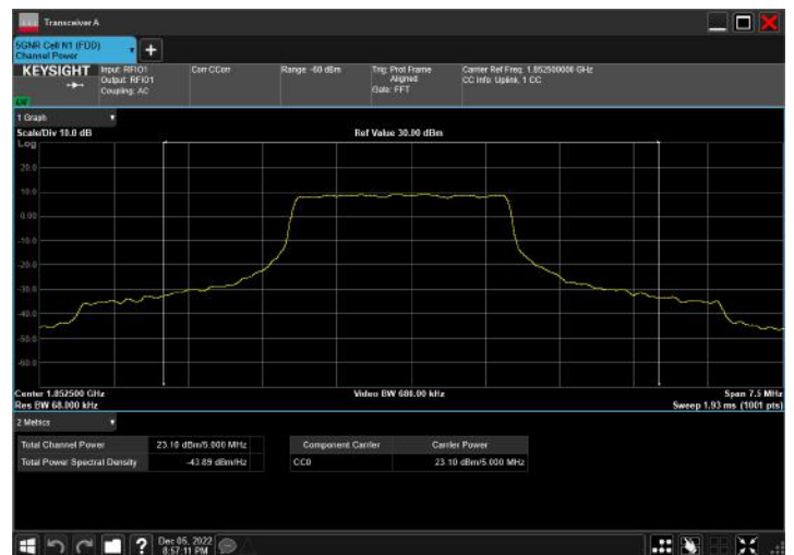
n2_5MHz_15kHz_1852.5MHz_DFT-s-OFDM QPSK_RB12@6
