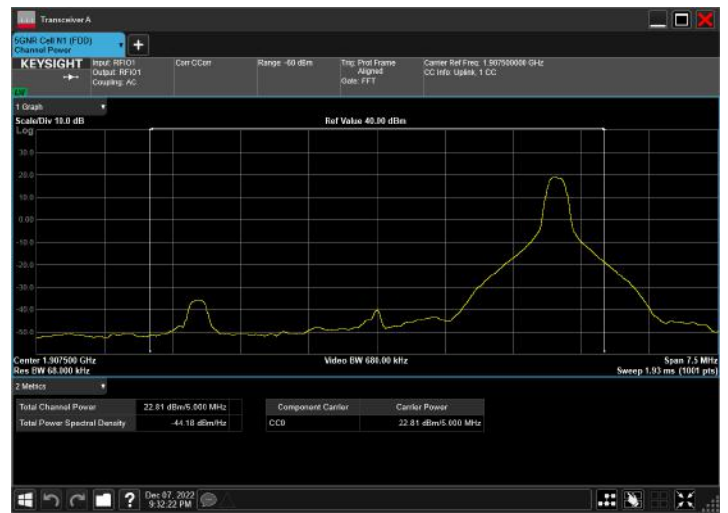
n2_5MHz_15kHz_1907.5MHz_CP-OFDM 16 QAM_RB25@0
