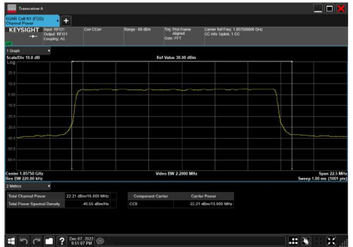
n2_15MHz_15kHz_1857.5MHz_DFT-s-OFDM 64 QAM_RB75@0
