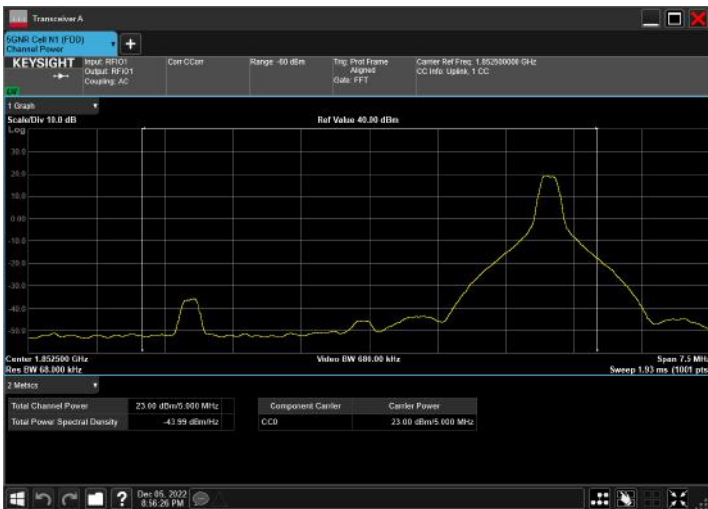
n2_5MHz_15kHz_1852.5MHz_DFT-s-OFDM PI/2 BPSK_RB1@23
