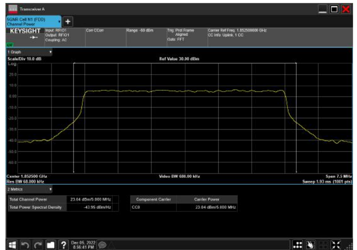
n2_5MHz_15kHz_1852.5MHz_DFT-s-OFDM PI/2 BPSK_RB25@0
