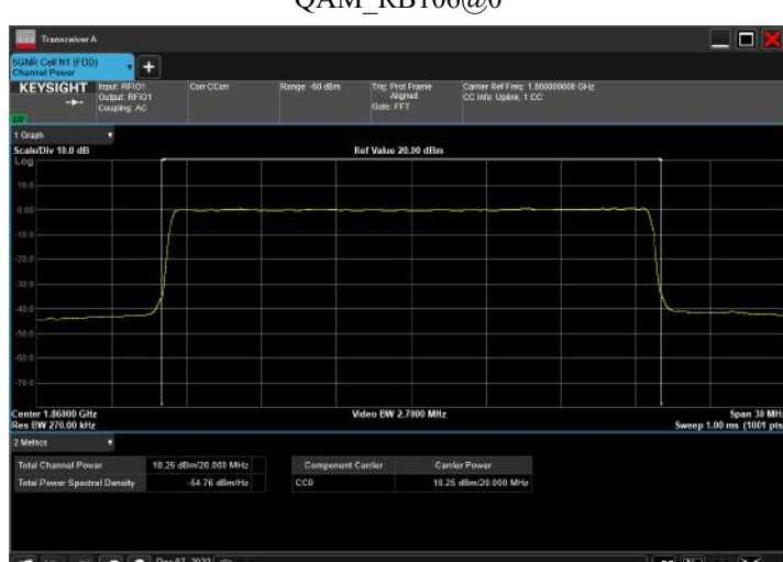
n2_20MHz_15kHz_1860MHz_CP-OFDM 256 QAM_RB106@0
