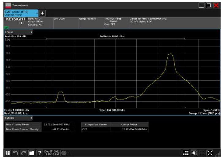
n2_5MHz_15kHz_1880MHz_DFT-s-OFDM 16 QAM_RB25@0
