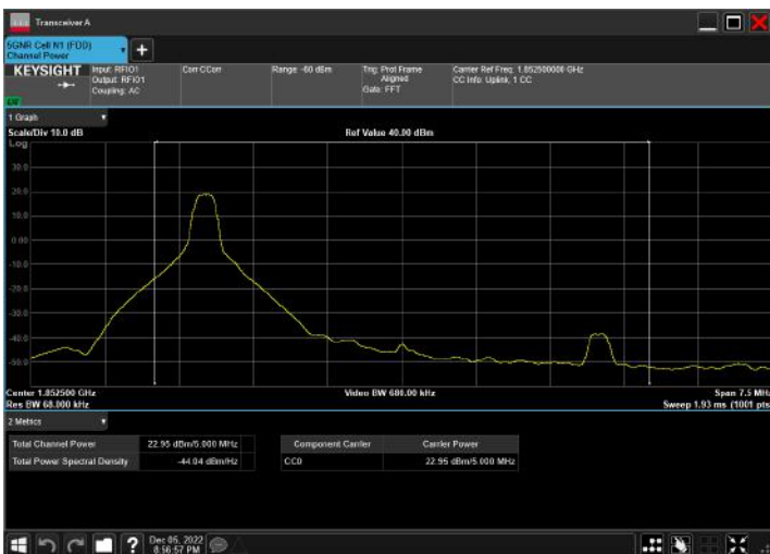
n2_5MHz_15kHz_1852.5MHz_DFT-s-OFDM QPSK_RB1@1
