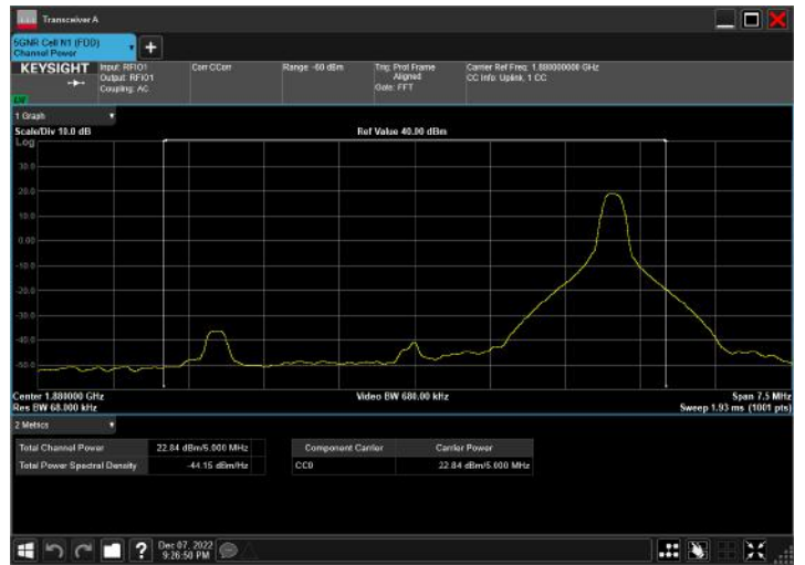
n2_5MHz_15kHz_1880MHz_CP-OFDM 16 QAM_RB25@0
