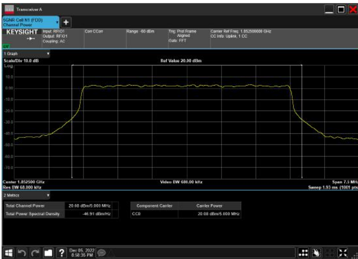
n2_5MHz_15kHz_1852.5MHz_DFT-s-OFDM 256 QAM_RB25@0
