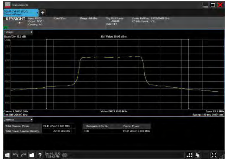
DC_66A_n2A_10MHz|15MHz_15kHz_1775MHz|1902.5MHz_QPSK|DFT-s-OFDM 256 QAM_RB12@38|RB36@18
