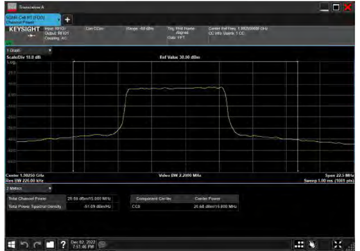
DC_66A_n2A_10MHz|15MHz_15kHz_1775MHz|1902.5MHz_QPSK|DFT-s-OFDM 16 QAM_RB12@38|RB36@18
