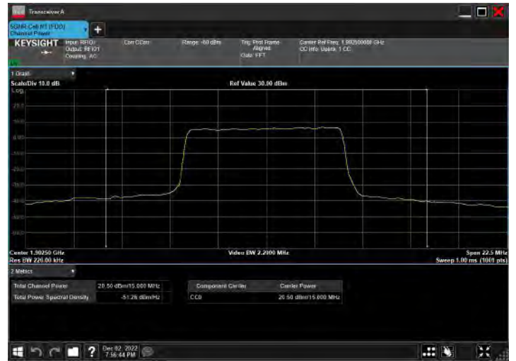
DC_66A_n2A_10MHz|15MHz_15kHz_1775MHz|1902.5MHz_QPSK|CP-OFDM 64 QAM_RB12@38|RB39@19
