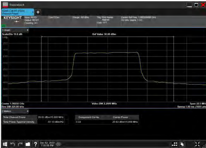
DC_66A_n2A_10MHz|15MHz_15kHz_1775MHz|1902.5MHz_QPSK|CP-OFDM 16 QAM_RB12@38|RB39@19
