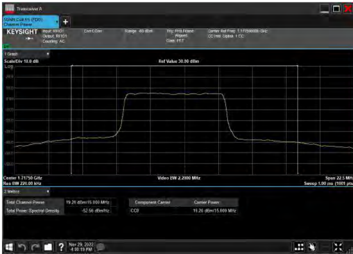
DC_2A_n66A_10MHz|15MHz_15kHz_1855MHz|1717.5MHz_QPSK|DFT-s-OFDM 256 QAM_RB12@0|RB36@18
