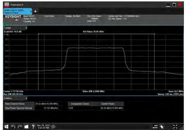
DC_2A_n66A_10MHz|15MHz_15kHz_1855MHz|1717.5MHz_QPSK|CP-OFDM 16 QAM_RB12@0|RB39@19
