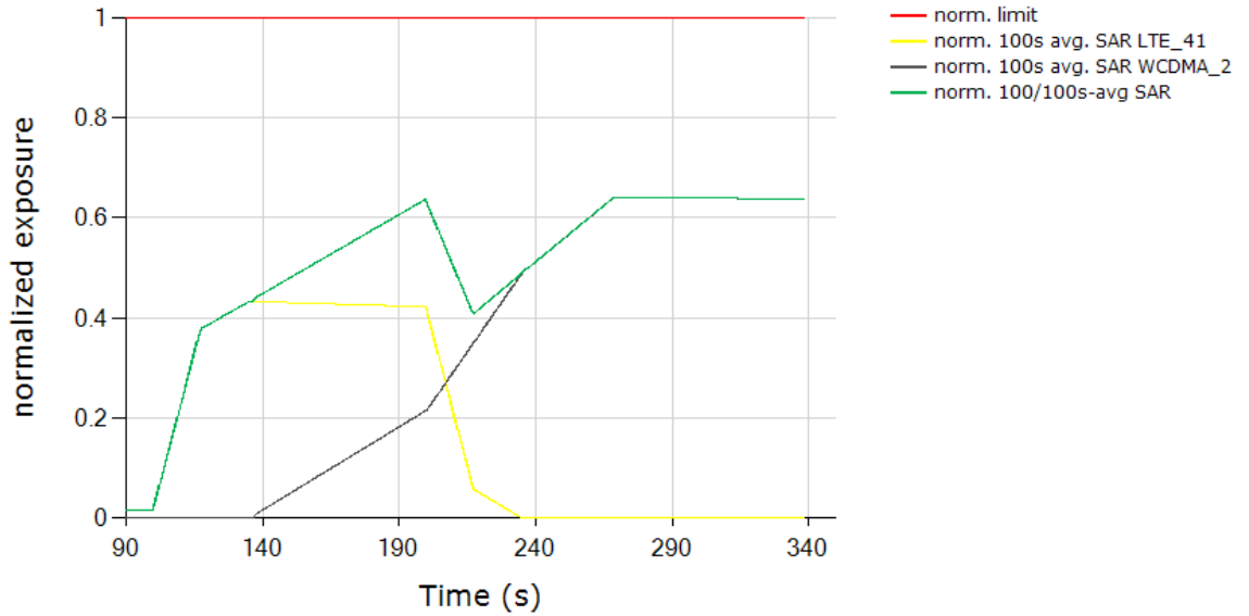
Total Normalized Time-averaged RF Exposure Tech: LTE, Band 41 / Tech: WCDMA, Band 2
