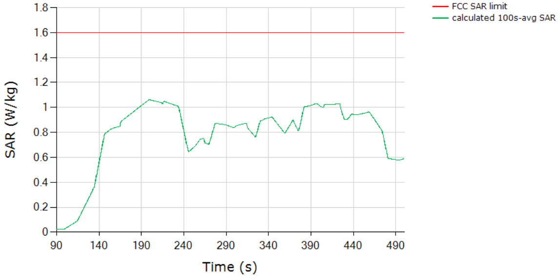
SAR (Test Sequence 2) Tech: LTE, Band 41
