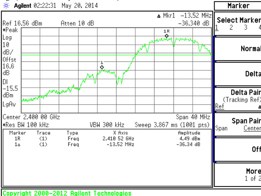
Plot #2 Band Edge {802.11b / 1 Mbps / 2.412 MHz}I
