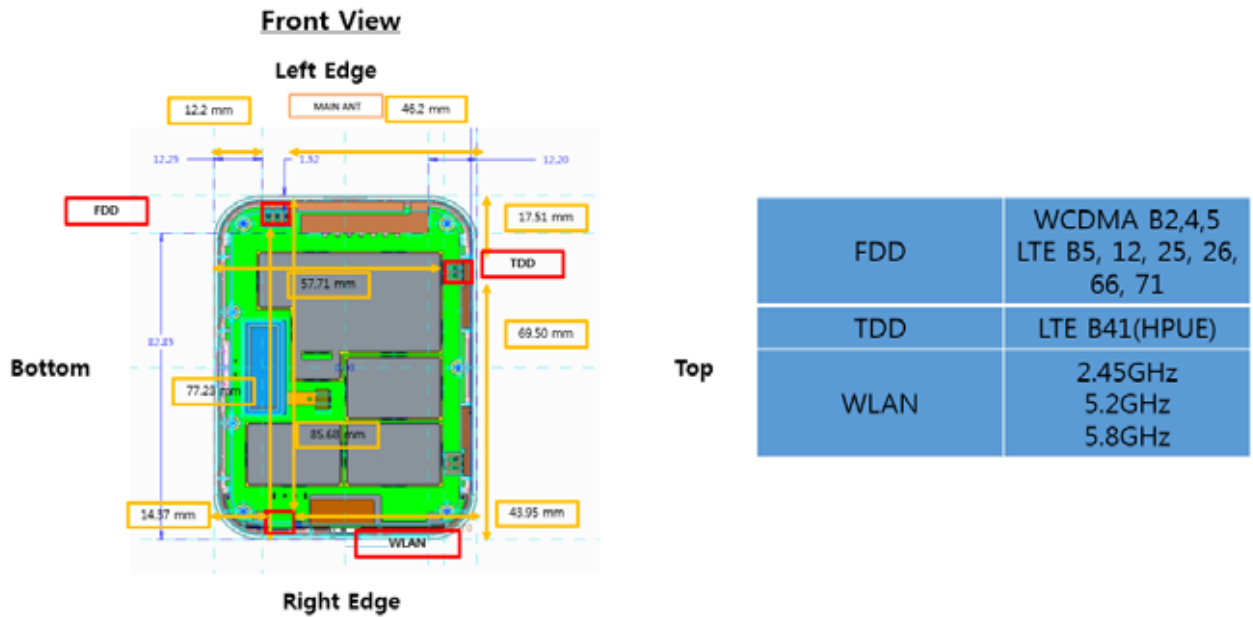
<The Distance information of Antenna to Edges of Wireless Router>
